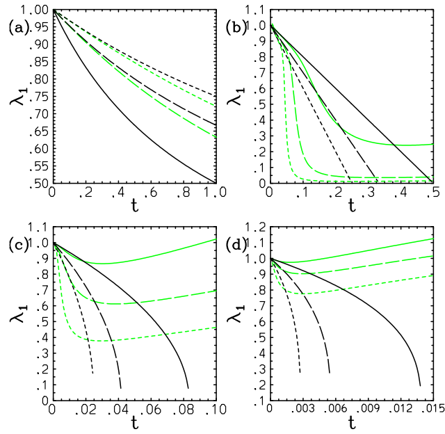
Figure 2. Plot of the obtained time series of \lambda_1 with m = 0 (a), \underline{1-2} (b), \underline{2-3} (c), and \underline{3-4} (d) with the weight exponents, n = 1 (solid), n = 2 (long dash), and n = 3 (short dash). The values of \lambda_1 evaluated from \langle \phi^n \rangle obtained by using the exact solutions are further overlaid by greens.
