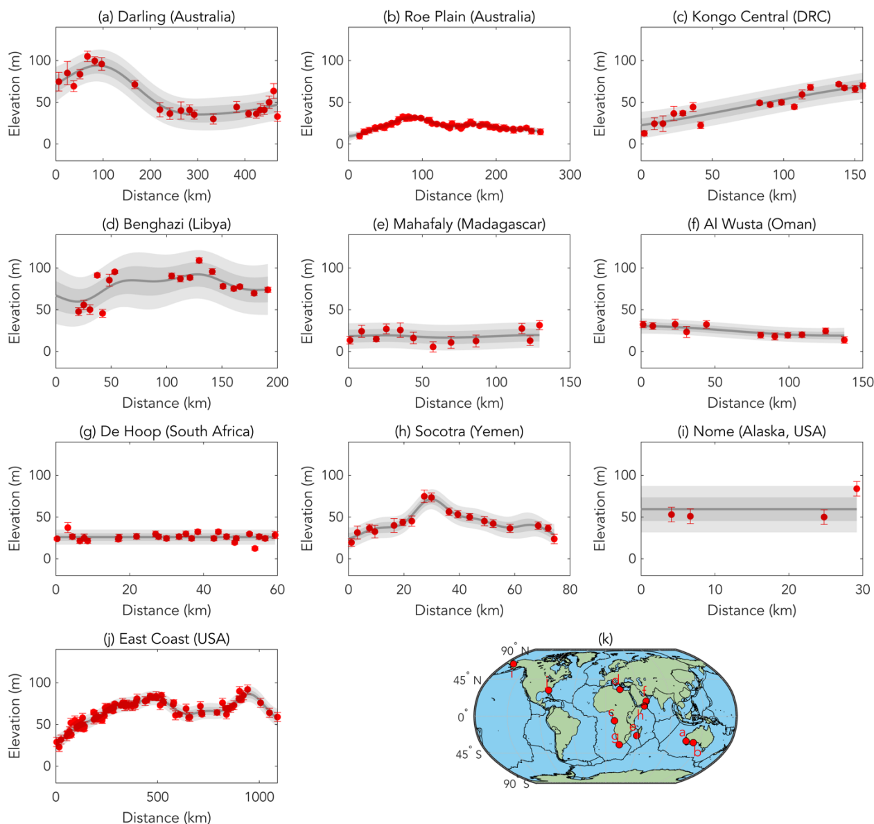
Figure 5: Along-scarp elevations profiles without geodynamic corrections. Red points indicate the mapped elevations of each scarp with uncertainties associated with the TerraceM analysis (Jara-Muñoz et al., 2016), field measurements, and indicative range. Gray line shows Gaussian Process Regression model trained by the data. Dark and light gray bands correspond to 1\sigma and 2\sigma uncertainties of the model, respectively. (a) Darling (Australia); (b) Roe Plain (Australia); (c) Kongo Central (DRC); (d) Benghazi (Libya); (e) Mahafaly (Madagascar); (f) Al Wusta (Oman); (g) De Hoop (South Africa); (h) Socotra (Yemen); (i) Nome (Alaska, USA); (j) East Coast (USA); (k) map inset showing site locations.
