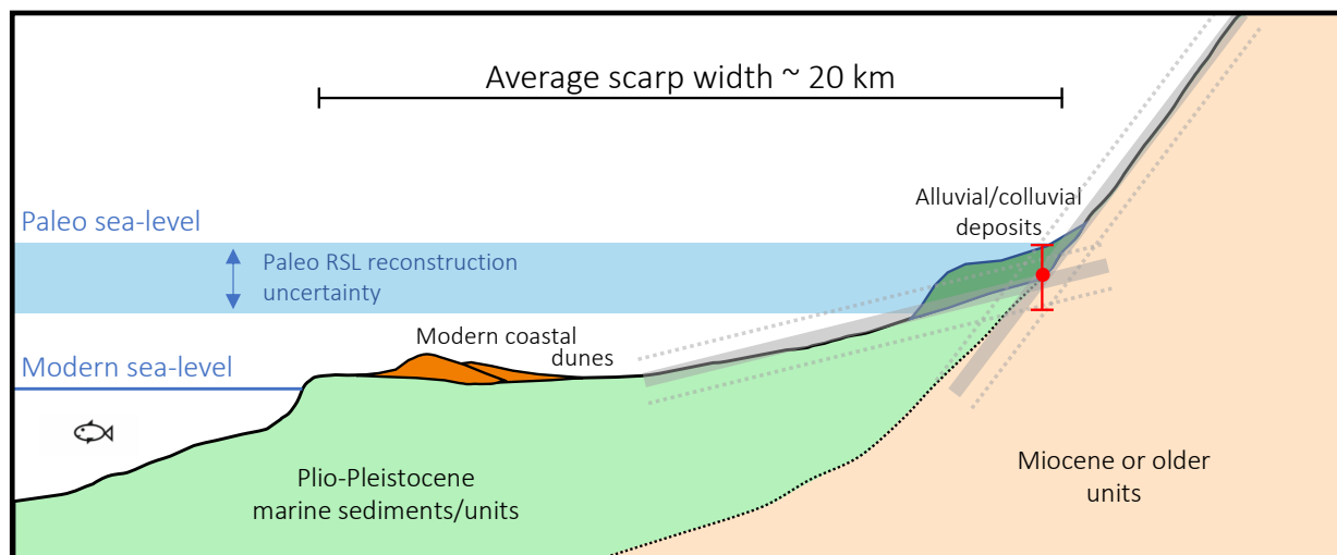
100 Figure 1: Schematic illustration of coast-perpendicular scarp profile. The grey lines (dashed lines indicate 2\sigma uncertainty bands) represent the TerraceM analysis, where the cliff and platform surfaces have been extrapolated to determine their geometric intersection, which often is buried under meters of alluvial/colluvial material (colored in dark green). The red point corresponds to the scarp toe elevation, and the red uncertainty bar describes the RSL estimate before the indicative range, GIA, or DT change corrections have been applied.
