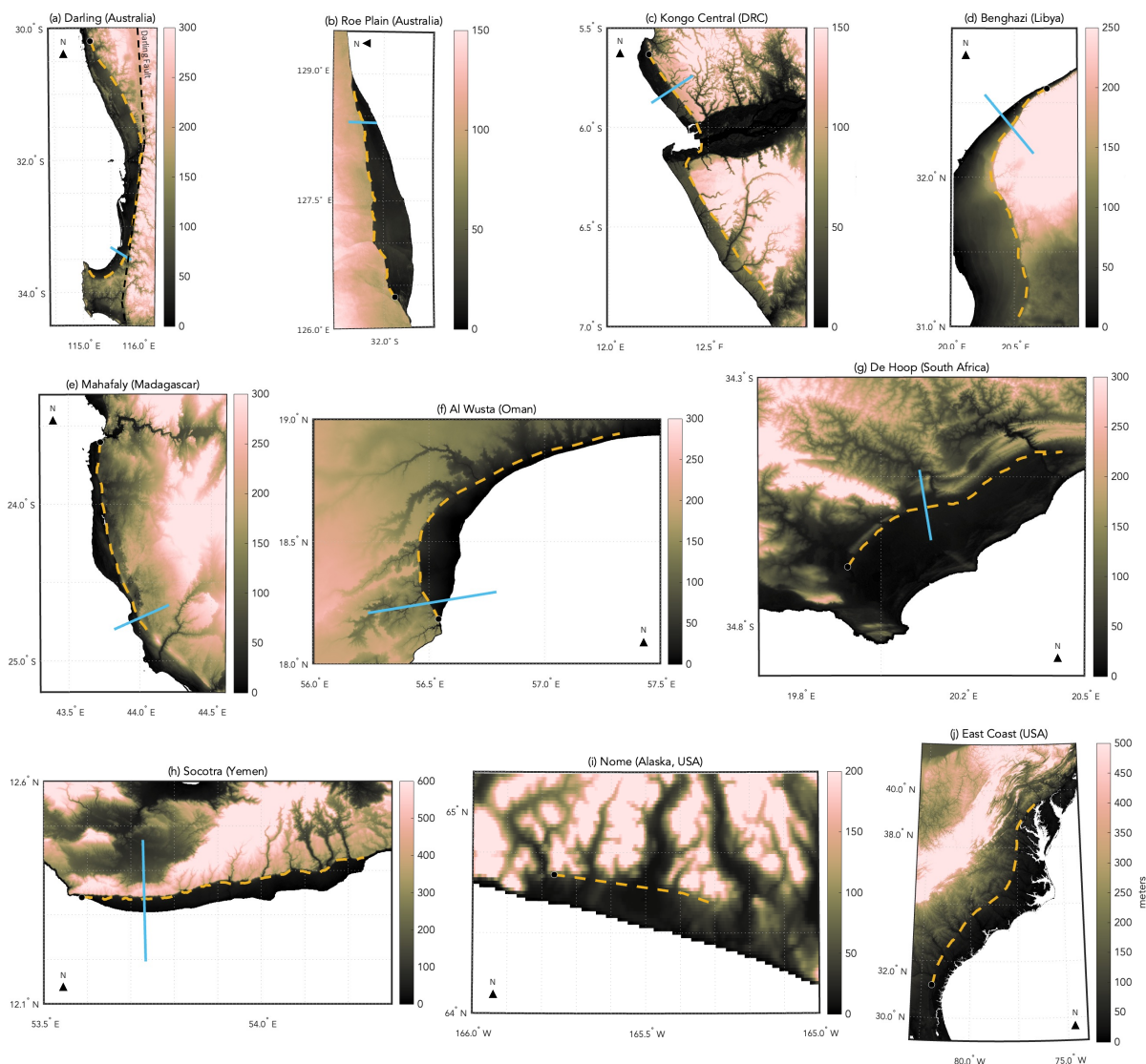
150 Figure 3: Compilation of DEMs for Pliocene-aged scarp database. (a-h): DEMs from the SRTM (Farr et al., 2007). (i & j): DEMs from the General Bathymetric Chart of the Oceans (GEBCO) 2023 grid (GEBCO Compilation Group, 2023). GEBCO DEMs were not used in our analysis of scarp geomorphology. Black circles indicate distance zero of the along-scarp profile, and the yellow dashed lines trace the along-scarp profile. Teal lines show the specific locations of the profiles perpendicular to the scarp, which were analyzed with TerraceM and are shown in Figure 4.
