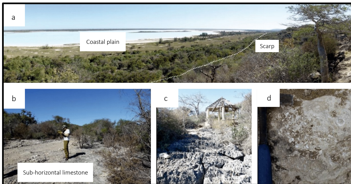
340 Figure 6: Field photos from Mahafaly (Madagascar) scarp taken in 2016. (a): View from the top of the cliff, looking seawards. (b): Sub-horizontal limestone at the base of the scarp. (c): Limestone at the top of the Mahafaly cliff. (d): Detail of the shell-rich limestone outcrop on the coastal plain, between the inner margin of the scarp and the coast.
