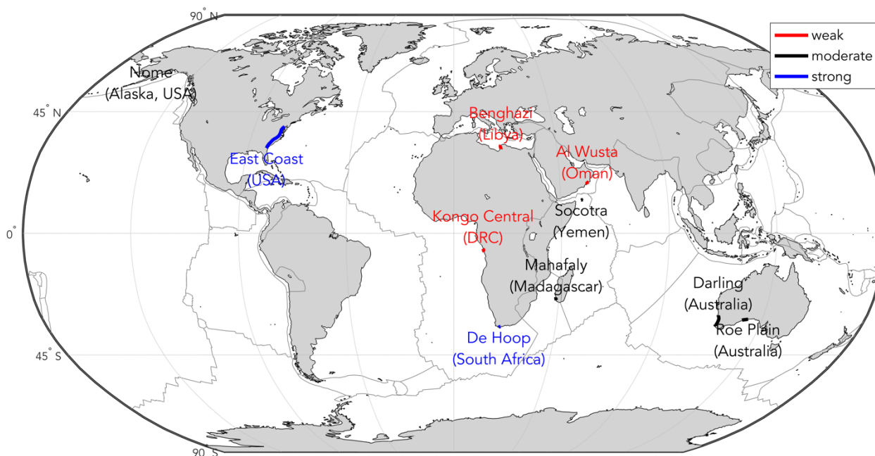
Figure 2: Global compilation of ten Pliocene-aged scarps. Colors indicate the quality of the age constraint relative to the MPWP (3 Ma).
