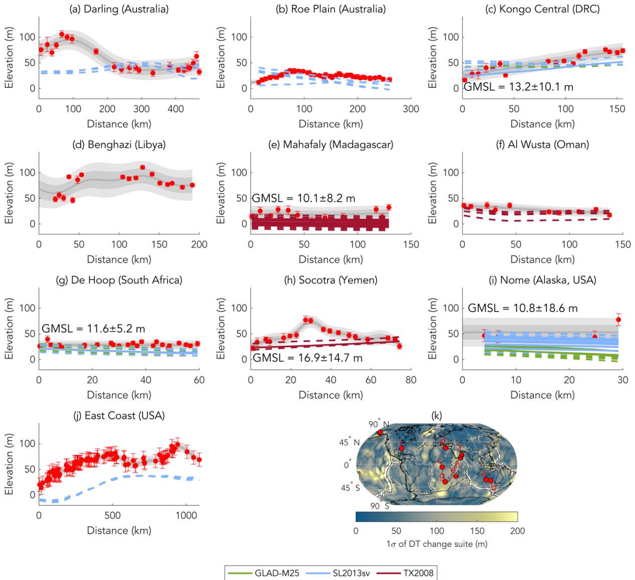
470 Figure 8: Comparison of GIA-corrected scarp deformation with predictions of DT change. Red points indicate mapped scarp elevations corrected for GIA. Their uncertainties are the square root of the sum of the squares of the individual uncertainties from the indicative range, field measurements, TerraceM analysis (Jara-Muñoz et al., 2016), and the GIA correction. Gray lines show Gaussian Process Regression models trained with the GIA-corrected elevation data. Dark and light gray bands correspond to 1\sigma and 2\sigma uncertainties of the Gaussian model, respectively. Green, blue, and red lines show predictions of DT change with upper mantle structures from the GLAD-M25, SL2013sv, and TX2008 tomography models, respectively (Lei et al., 2020; Schaeffer & Lebedev, 2013; Simmons et al., 2009). Solid colored lines correspond to DT change solutions that fit the stringent fitting criteria. Dashed colored lines correspond to DT change solutions that meet the weak fitting criteria. The inferred GMSL and fully propagated uncertainty is shown for sites that meet the stringent fitting criteria. (a) Darling (Australia); (b) Roe Plain (Australia); (c) Kongo Central (DRC); (d) Benghazi (Libya); (e) Mahafaly (Madagascar); (f) Al Wusta (Oman); (g) De Hoop (South Africa); (h) Socotra (Yemen); 480
