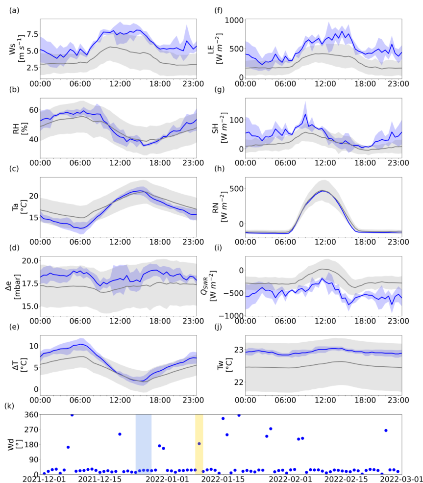
445 Figure 8: Extreme surface heat loss case study mean diurnal cycle (LT) during the event (blue) and the reference DJF 2021 period (gray), in the shaded area the \pm 1 SD span. (a) Wind speed ( Ws ), (b) relative humidity ( RH ), (c) air temperature ( Ta ), (d) vapor pressure difference ( \Delta e ), (e) water-air temperature difference ( \Delta T ), (f) latent heat flux ( LE ), (g) sensible heat flux ( SH ), (h) net radiation ( RN ), (i) water temperature ( Tw ), (k) DJF mean daily wind direction, the blue shaded area marks the heat loss event (25-28 December 2021), and the yellow shaded area is the comparison event (9 January 2022) where the wind is sea originated; therefore, high air temperature and relative humidity prevent high rates of heat loss.
