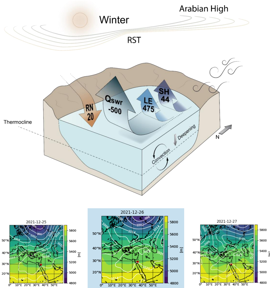
410 Figure 7: Surface heat loss case study synoptic maps (bottom) and schematic representation of the mean energy partitioning during the event (top). (Bottom) Average daily ERA5 reanalysis variables synoptic maps, sea level pressure (hPa) plotted in white in contour (Hersbach et al., 2023b), and the 500hPa geopotential height (m) plotted in shaded colors (Hersbach et al., 2023a). The event occurred between 25-27.12.2021 (shaded map marks the peak of the event) and involved the intensification of the Arabian High and the Red Sea Trough. (Top) Surface energy fluxes are given in W m^{-2} . The large heat loss is affecting the deepening of the thermocline and the winter annual vertical water column mixing. 415
