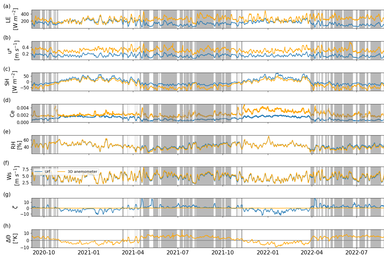
350 Figure 5: Comparison between the 3-day (LT) rolling average EC-measured sensible and latent heat fluxes and meteorological parameters (orange) and the bulk formula calculation using TOGA-COARE 3.6 algorithm (blue) computed with the NMP micrometeorological data. Shaded in gray are instances where the TOGA-COARE 3.6 algorithm bulk Richardson number is within the range of 0-0.2 indicating stable conditions. The wind speed panel compares the measurements of the 3D sonic anemometer and the interpolated referenced height (7 m) of the TOGA-COARE 3.6 algorithm. (a) Latent heat ( LE ), (b) friction velocity ( u^* ), (c) sensible heat ( SH ), (d) vapor transfer coefficient (reversed calculated from the EC measurements Eq. (9)), (e) relative humidity ( RH ), (f) wind speed ( Ws ), (g) stability ( \zeta ), (h) air and water potential temperature difference ( \Delta\theta ). Key variations between the EC method and the bulk formula are higher evaporation rates measured with the EC system during stable conditions, consistent higher friction velocity measured with the 3D sonic anemometer, and low variation within the stability parameter calculated with the EC system.
