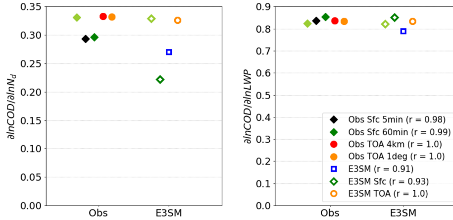
Figure 11: \ln COD as a function of (left) \ln N_d and (right) \ln LWP for observational and E3SM datasets. Estimates are obtained from ordinary least squares multiple linear regression with Pearson correlation coefficients shown in the legend. Light green symbols represent Obs Sfc 60min and E3SM Sfc datasets with a recomputed N_d that assumes 80% adiabaticity like the TOA retrievals.
