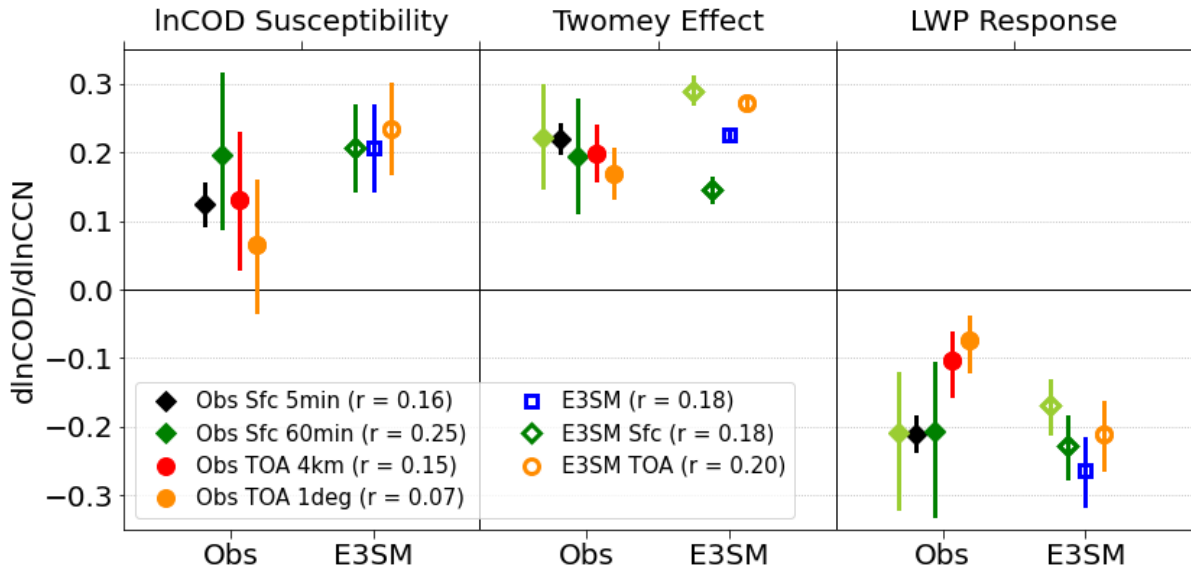
Figure 19: (left) \ln COD susceptibility to CCN concentration with (middle) Twomey effect (\frac{\partial \ln COD}{\partial \ln N_d} \frac{d \ln N_d}{d \ln CCN}) and (right) LWP response (\frac{\partial \ln COD}{\partial \ln LWP} \frac{d \ln LWP}{d \ln N_d} \frac{d \ln N_d}{d \ln CCN}) terms for observational and E3SM datasets with 95% confidence intervals. Pearson correlation ( r ) coefficients for \ln COD regressed on \ln CCN are shown in the legend. Light green symbols represent Obs Sfc 60min and E3SM Sfc datasets with a recomputed N_d that assumes 80% adiabaticity like the TOA retrievals.
