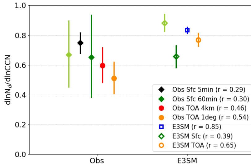
1180 Figure 17: \ln N_d as a function of \ln CCN for observational and E3SM datasets. Estimates are obtained from Theil-Sen robust linear regression with 95% confidence intervals. Pearson correlation coefficients are shown in the legend. Light green symbols represent Obs Sfc 60min and E3SM Sfc datasets with a recomputed N_d that assumes 80% adiabaticity like the TOA retrievals.
