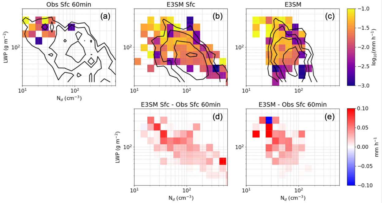
Figure 23: Median surface hourly rain rate as a function of LWP and N_d for (a) Obs Sfc 60min disdrometer retrievals, (b) E3SM Sfc, and (c) E3SM. (d) Absolute differences between E3SM Sfc and Obs Sfc 60min. (e) Absolute differences between E3SM and Obs Sfc 60min. Only rain rates exceeding 0.001 \text{ mm h}^{-1} are included in statistics due to observational sensitivity limitations. Black contours indicate sample size thresholds of 0.4, 0.8, 1.6, and 3.2%, respectively.
