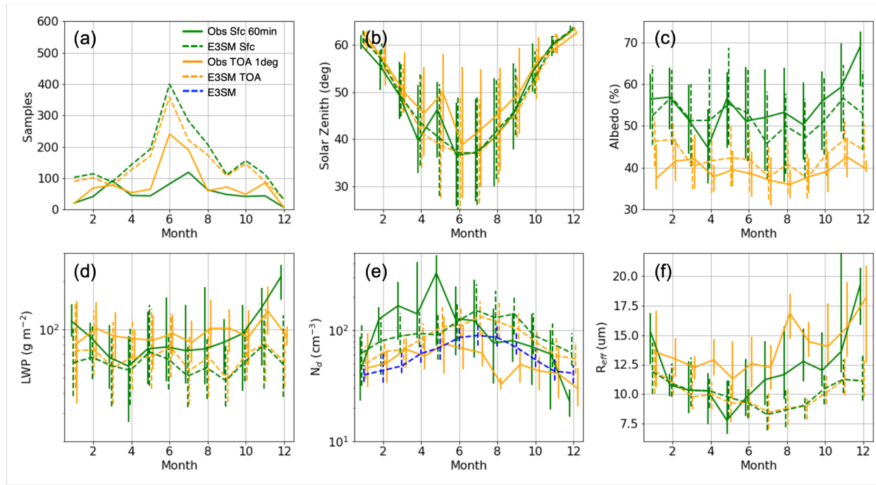
Figure 10: Seasonal cycles of (a) number of samples and interquartile ranges (vertical bars) connected by medians for (b) SZA < 65^\circ , (c) TOA or cloud effective albedo, (d) cloud LWP, (e) layer-mean N_d , and (f) R_{eff} .
