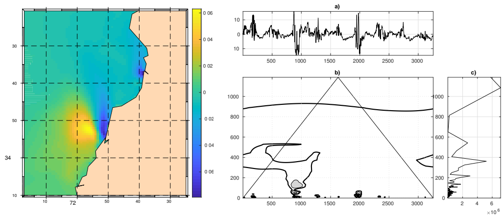
Figure 14. (Left panel) EOF Mode 2 map. (a) EOF PC 2 time series, (b) Wavelet spectrum of the PC series and (c) cumulative global wavelet spectrum.
