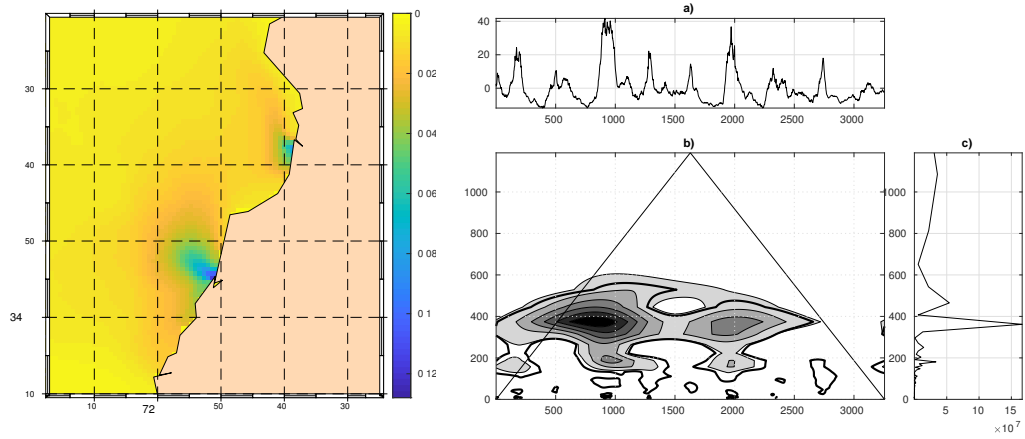
Figure 13. (Left panel) EOF Mode 1 map. (a) EOF PC 1 time series, (b) Wavelet spectrum of the PC series and (c) cumulative global wavelet spectrum.
