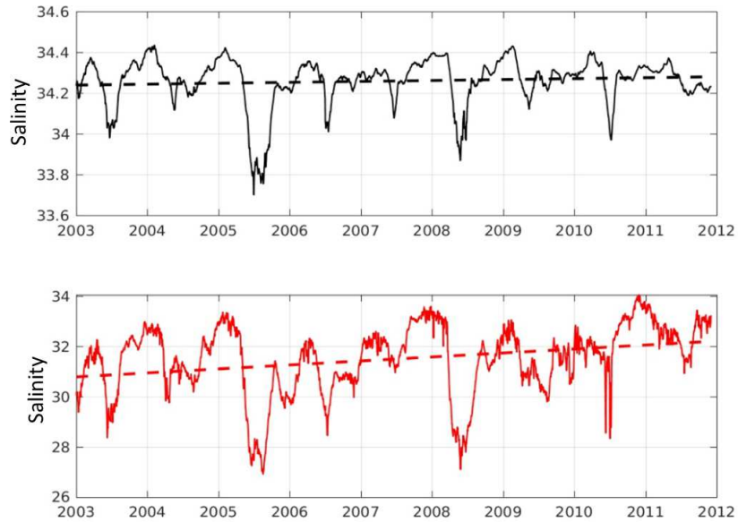
Figure 8. Time series and trends of the (top panel) maximum and (bottom panel) minimum surface salinity over the domain
