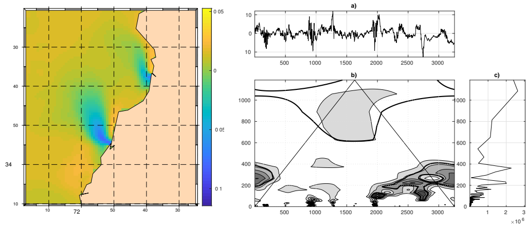
Figure 15. (Left panel) EOF Mode 3 map. (a) EOF PC 3 time series, (b) Wavelet spectrum of the PC series and (c) cumulative global wavelet spectrum.
