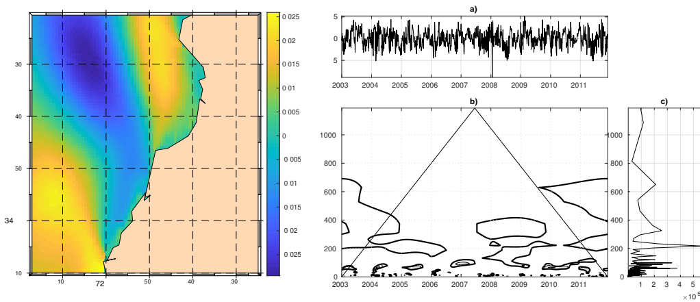
Figure 18. (Left panel) Meridional velocity EOF Mode 3 map. (a) EOF PC 3 time series, (b) Wavelet spectrum of the PC series and (c) cumulative global wavelet spectrum.
