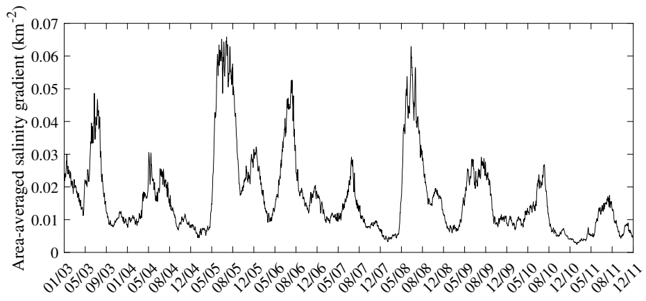
Figure 9. Variation of the area-averaged salinity gradient (AASG) in the Maipo-Rapel plume area.
