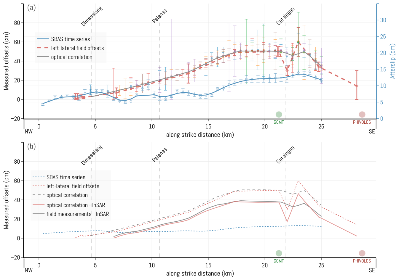
Figure 12. Combined slip distribution plots. A) Solid gray line shows the weighted moving mean of the six valid optical correlation pairs. Dashed red line represents the weighted moving mean of the field measurements. Blue line and markers represent the afterslip from InSAR placed in a secondary axis. B) Residual curves of the weighted moving mean pixel offsets and field measurements with InSAR to estimate the coseismic slip.
