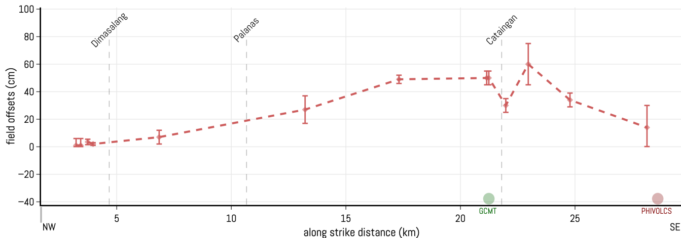
Figure 11. Along strike distribution of measured field offsets acquired on May 2022.
