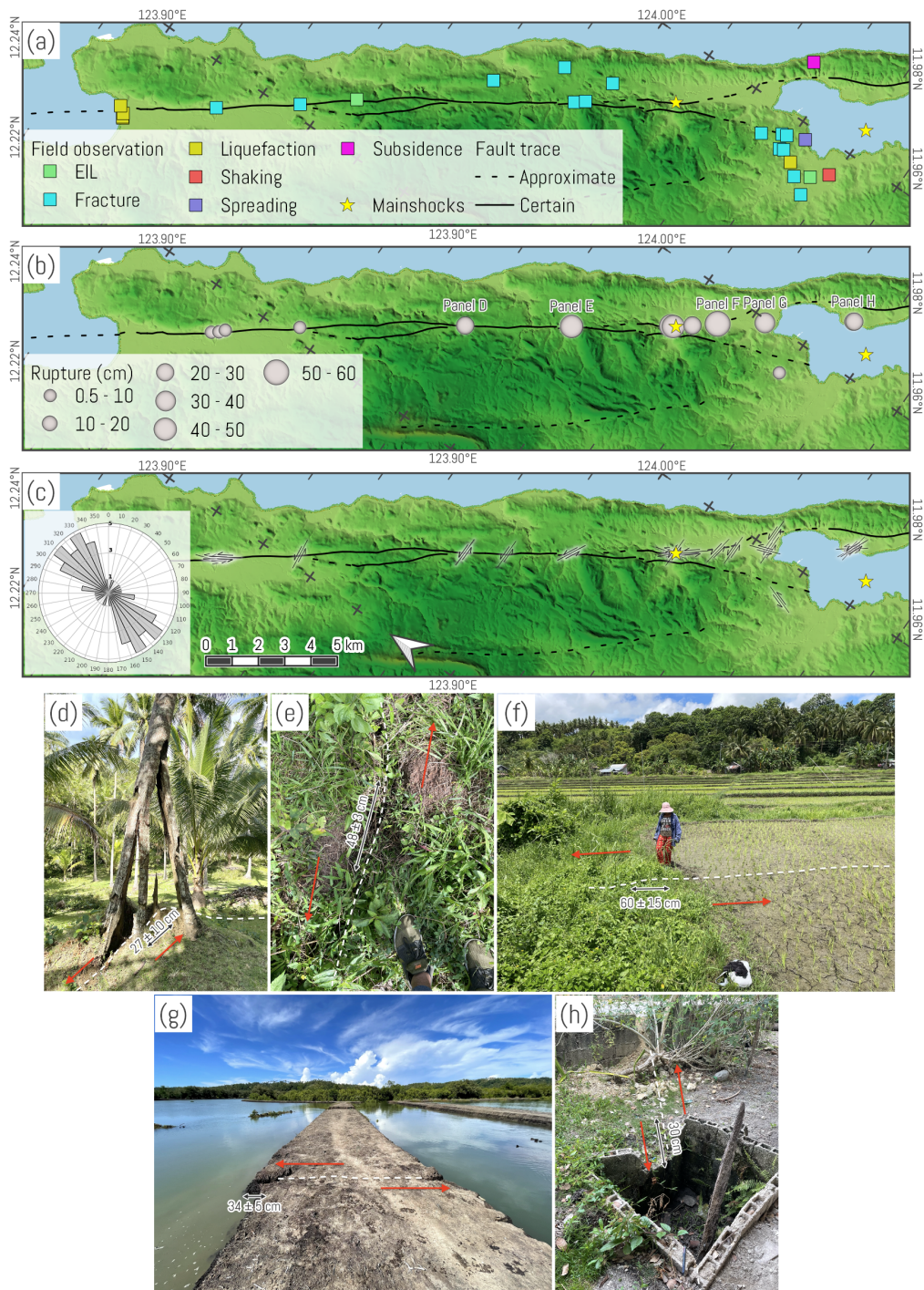
Figure 10. Compiled ground-truthing data. A) Earthquake hazards aside from ruptures. B) Ruptures symbolized by size showing the amount of slip. C) Rupture orientations. D) Ruptured tree showing cumulative 87 cm slip from 2003 and 2020 events with estimated 27 \pm 10 cm offset from the 2020 earthquake. E) Soil mound cut by the fault highlighting a 48 \pm 3 cm left lateral offset. F) Rice field embankment traversed by fault showing 60 \pm 15 cm displacement. G) Ruptured fishpond dike recording a 34 \pm 5 cm offset. H) Abandoned septic tank showing a 30 cm displacement south of Cataingan Bay.
