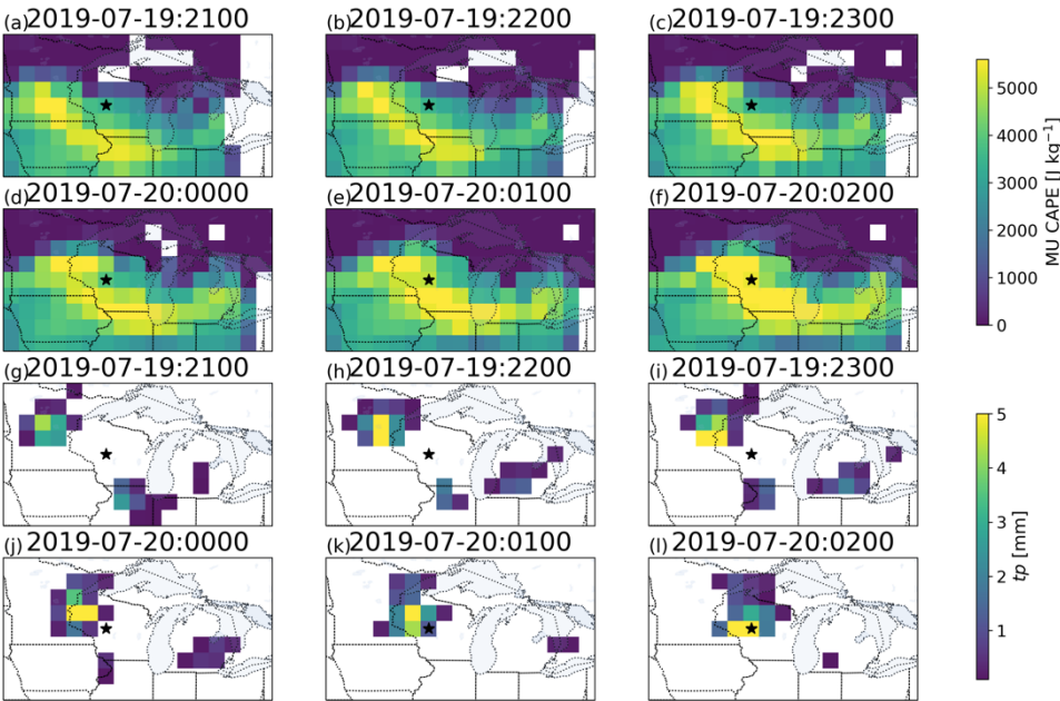
320 Figure 5. (a—f) ERA5-FCST calculated most-unstable parcel CAPE over the US upper-Midwest for the six hours starting 2100 UTC. (g—l) ERA5 hourly precipitation in the same area. Star added at 44.5 °N, 90.5 °W represents the location of peak precipitation at hour 6.
