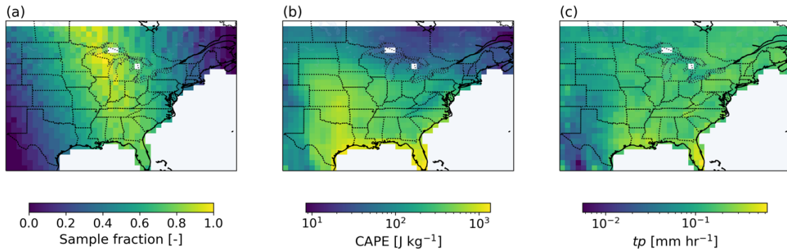
270 Figure 1. March—November 2019 means of (a) fraction of days with AIRS swath coverage location, including cloudy-sky footprints, (b) ERA5 mean CAPE during overpass time, (c) ERA5 mean precipitation during overpass time. Grid cells are masked if they contain no land; this includes the ocean and some cells in the Great Lakes.
