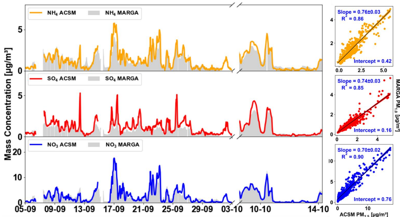
Figure 4 Time series of TOF-ACSM measured SIA-PM 2.5 during the whole period. MARGA measured PM 1.0 from September 5 th to September 30 th in 2021, and PM 2.5 from October 3 rd to October 15 th in 2021. The corresponding linear regression fitting correlations between MARGA PM 1.0 and TOF-ACSM PM 2.5 .
