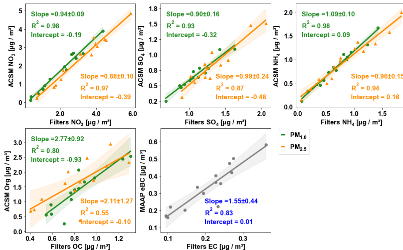
Figure 1 Comparison of the online (ACSM and MAAP) and offline (Filters) mass concentrations of various chemical components. PM 1.0 is indicated in green and PM 2.5 in orange. The shaded area represents the 95% confidential interval of the best fit line.
