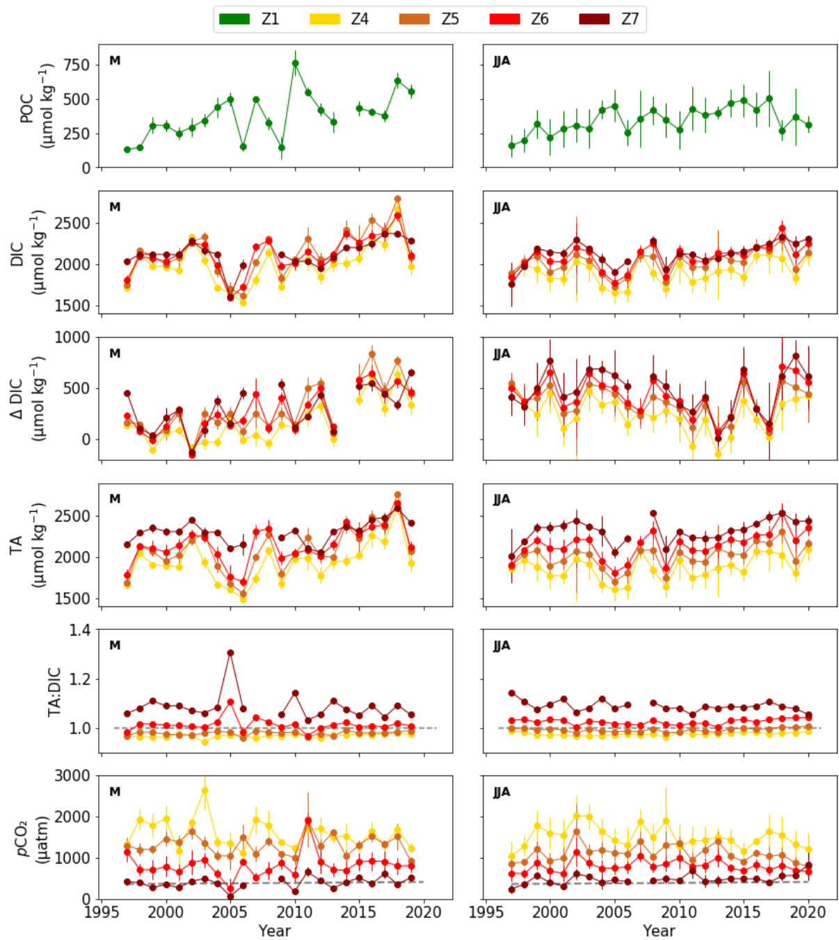
375 Figure 4. Late spring (May, M) and summer (June–August, JJA) POC in zone 1 (Z1) and DIC, along-estuary DIC gain ( \Delta\text{DIC} ), TA, TA:DIC ratio (1 indicated by grey dashed line), and p\text{CO}_2 , with atmospheric \text{CO}_2 values (grey dashed line) from Global Monitoring Laboratory (Lan et al., 2023), in the mid to outer estuary (zone (Z) 4–7, see Fig. 1b) from 1997 to 2020 (in May to 2019). Note differences in y-axis scales. Error bars represent the standard deviations of the mean. 380
