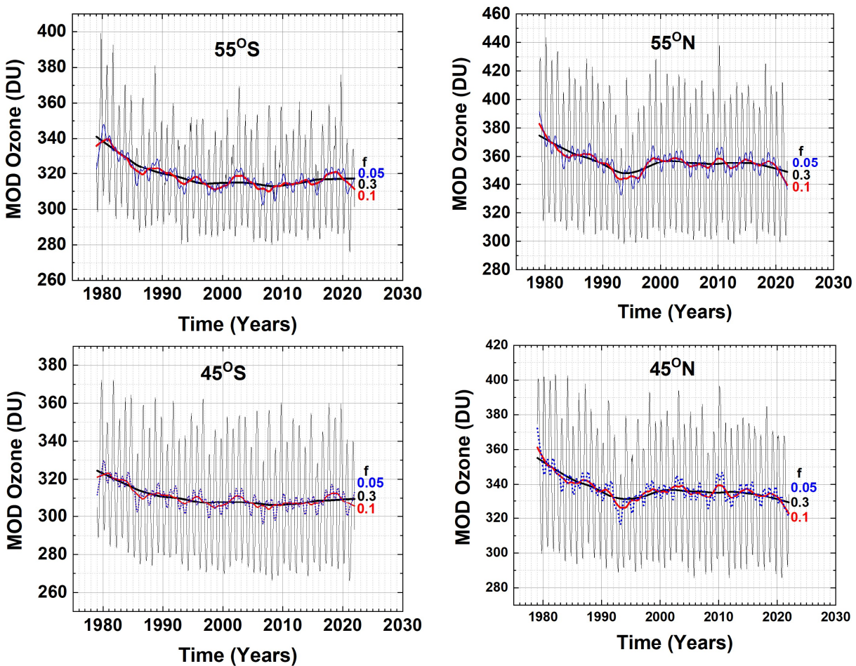
Fig. 5 \Omega_{\text{MOD}} in four latitude bands and Lowess(0.3) fitting functions ( f = 0.3 , black lines). Examples of different f = 0.1 (Red) and 0.05 (blue dots) are shown at 45^\circ\text{S} and 45^\circ\text{N} . Note the slight downturn since 2010 in the Lowess(0.3) at 45^\circ\text{N} and 55^\circ\text{N} .
