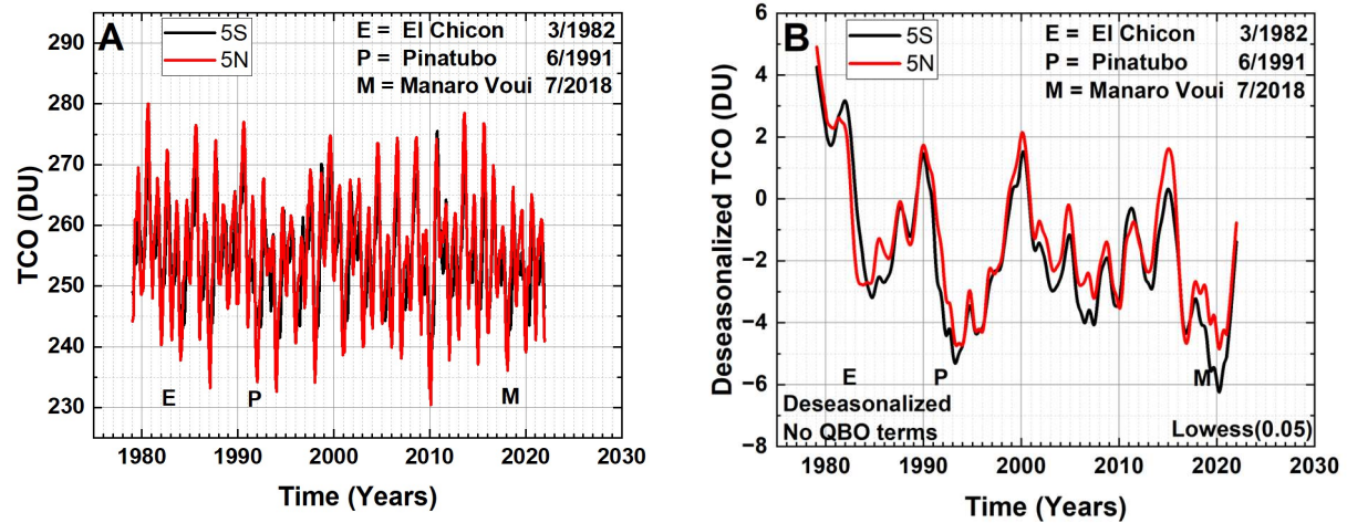
Fig. 4. A. \Omega_{\text{MOD}} time series for \theta = 5^\circ\text{N} and 5^\circ\text{S} . B. The deseasonalized TCO time series for \theta = 5^\circ\text{N} and 5^\circ\text{S} without removing QBO effects (Eq. 1). The approximate dates are shown of volcanic eruptions that injected large amounts of \text{SO}_2 into the stratosphere leading to minima approximately 1 year later.
