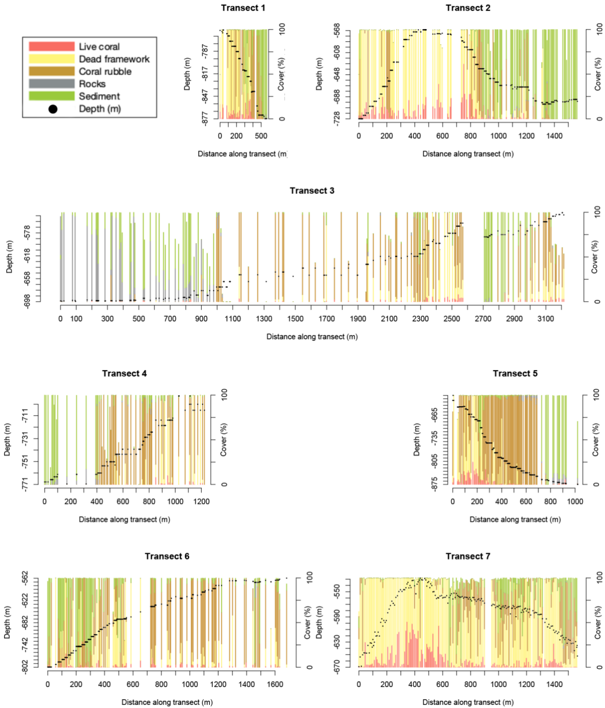
Figure 2. Stacked barplots show the benthic cover (in percent of the annotated frame) of the seven transects. Each bar represents one annotated video frame. Note: for visibility, only frames at >5.5 m distance apart are shown. Benthic cover types shown are the
