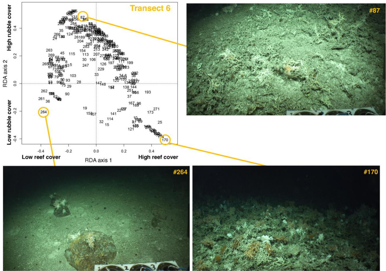
Figure 3. Annotated video frames from transect 6 plotted on the first (x-axis) and second (y-axis) redundancy analysis (RDA) axes, with three representative images from the seafloor. The first RDA axis separates images with low reef cover (such as image #264) from images with high reef cover (such as image #170). The second RDA axis separates images with low rubble cover (such as image #264 and #170) from images with high coral rubble cover (such as image #87). Note: images are directly extracted from the videos without modifications or annotations. The videos were obtained during the Changing Oceans 2012 expedition with RRS James Cook ©2012 Laurence De Clippele.
