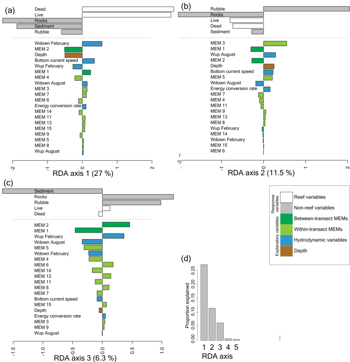
230 Figure 4. Bar plot of the components of the first (a), second (b), and third (c) axis of the redundancy analysis (RDA), explaining 27 %, 11.5 %, and 6.3 % of the variation in benthic cover respectively. The x-axis shows the value on the RDA axis. RDA axes 1 to 4 were significant ( p < 0.05 ), but axis 4 is not shown as it explained < 1 % of the variation in benthic cover (d). The benthic cover (response) variables are shown at the top (reef variables in white and non-reef variables in grey) and below that, the explanatory
