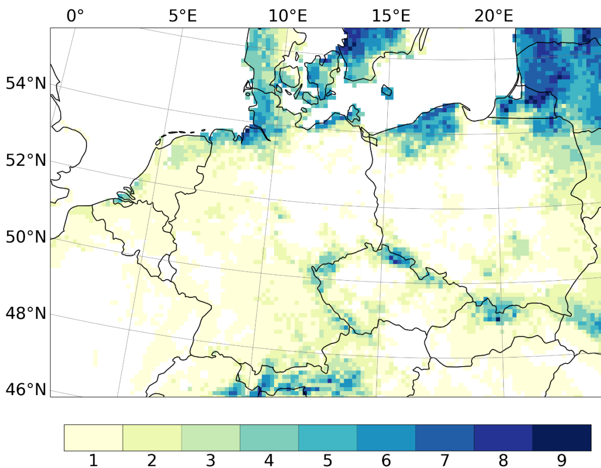
Fig: Number of models that disagree with the multi-model mean shown in Fig. 2. For these models the difference in the number of events between the historical and the scenario period is statistically significant at the 95% level but of the opposite sign.
