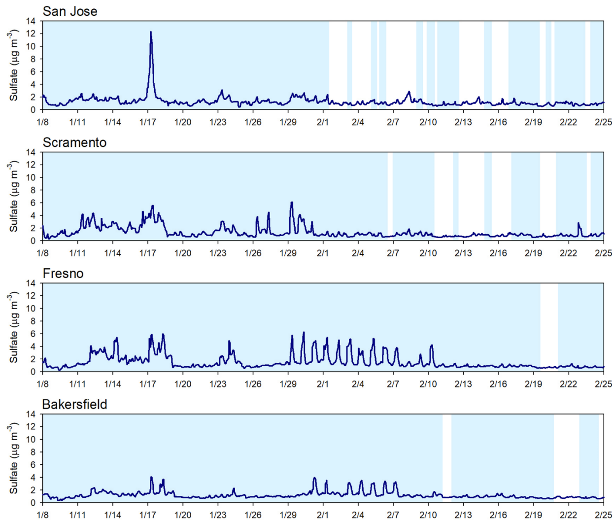
Fig. S11. Time series of hourly simulated (a) Sulfate, (b) Nitrate, and (c) Ammonium at each site between January and February in 2018.
