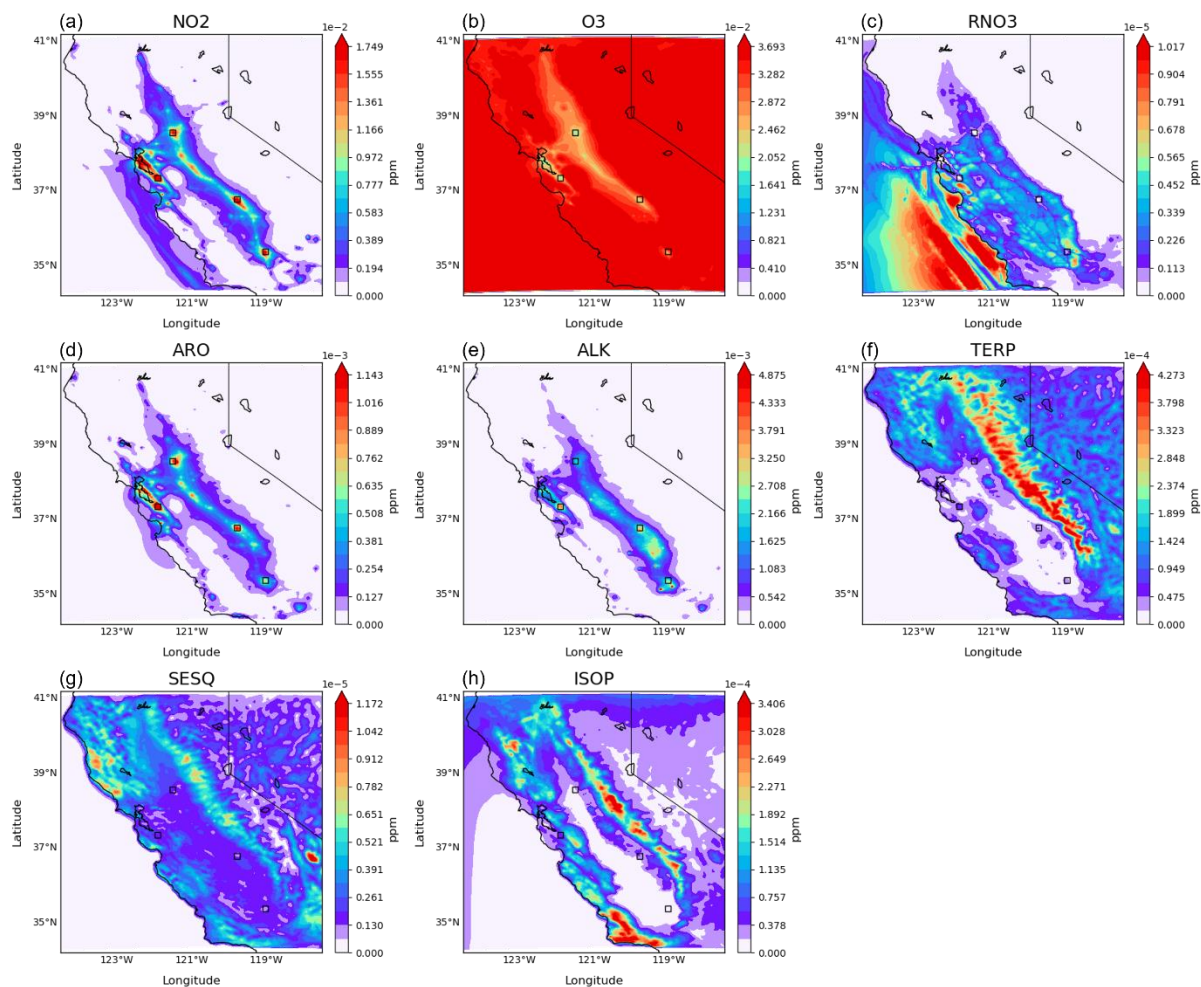
Fig. S10. Spatial distributions of (a) NO 2 , (b) Ozone, (c) Nitrate radical, (d) ARO, (e) ALK5, (f) TERP, (g) SESQ, and (h) ISOP concentrations averaged between 01/23/2018 and 02/24/2018. ARO is the sum of benzene, toluene, o-xylene, p-xylene, m-xylene, and 1,2,4-trimethylbenzene.
