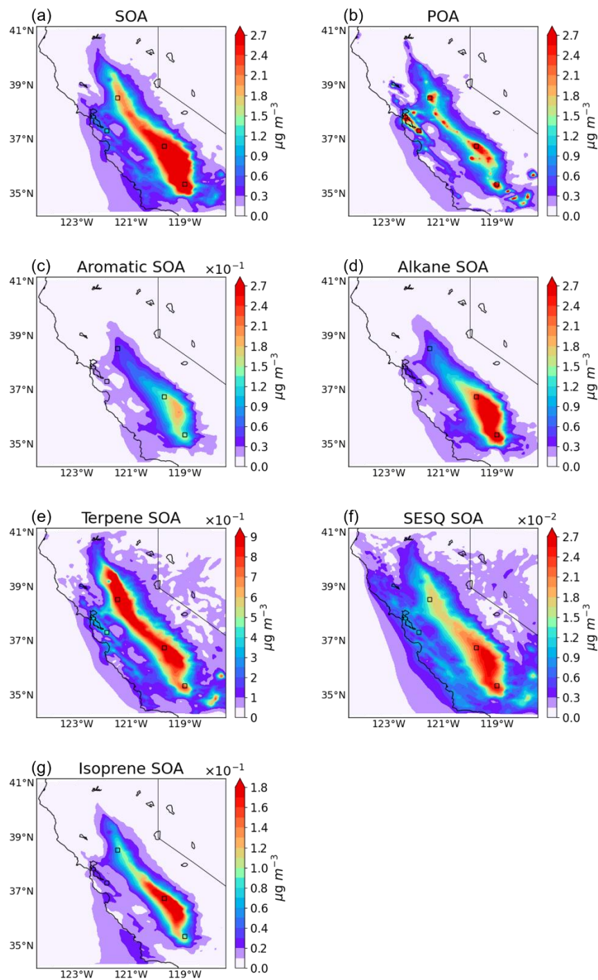
925 Fig. 6. Spatial distribution of (a) total SOA, (b) POA, (c) aromatic SOA (OMP_AR+OMH_AR), (d) alkane SOA (OMP_AK+OMH_AK), (e) terpene SOA (OMP_TE+OMH_TE), (f) sesquiterpene SOA (OMP_SP+OMH_SP), and (g) isoprene SOA (OMP_IS+OMH_IS). The simulation results at the surface level were averaged between 01/23/2018 and 02/24/2018.
