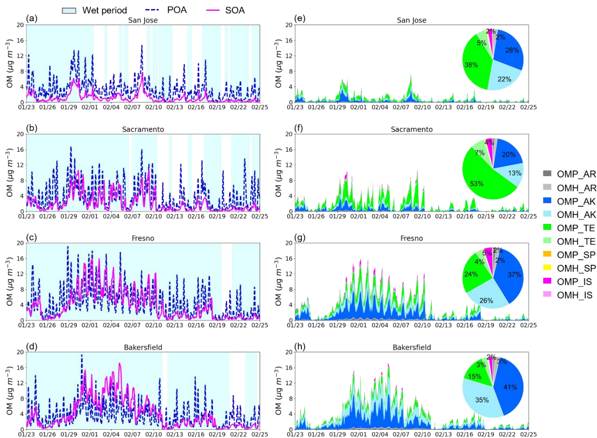
915 Fig. 4. (a–d) Time series of simulated POA, SOA, and salted aerosol phase state (wet and dry). (e–h) Time series of simulated SOA species in the UNIPAR model at each site and the pie charts to represent the fraction of SOA species associated with graphs (e–h).
