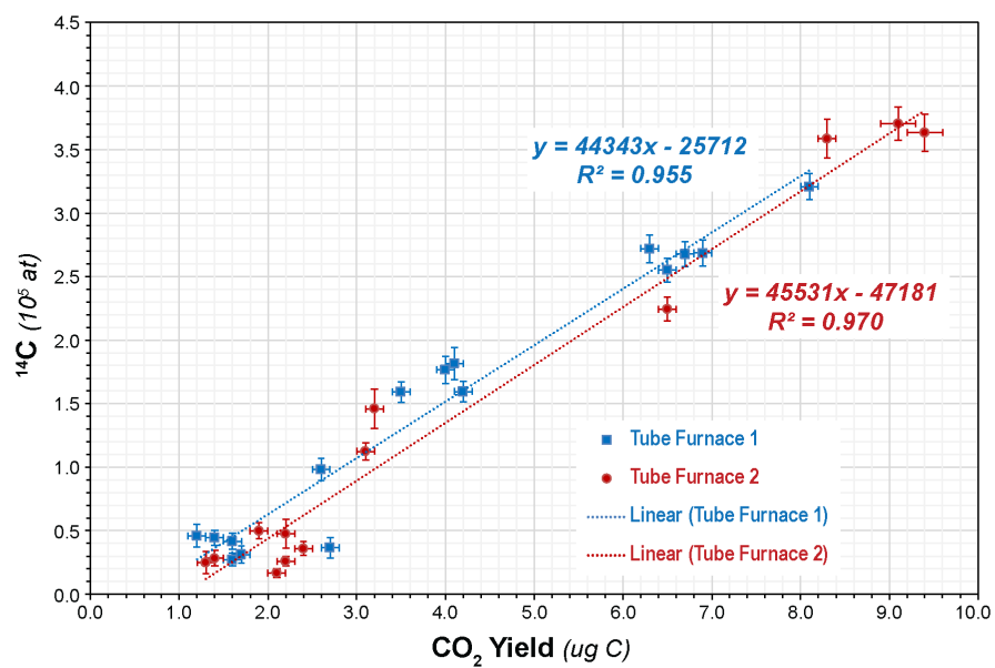
545 Figure 5: Linear fit between CO 2 yield in µg C vs. procedural blank in 14 C atoms, for Tube Furnaces 1 and 2 (1σ uncertainties shown).
