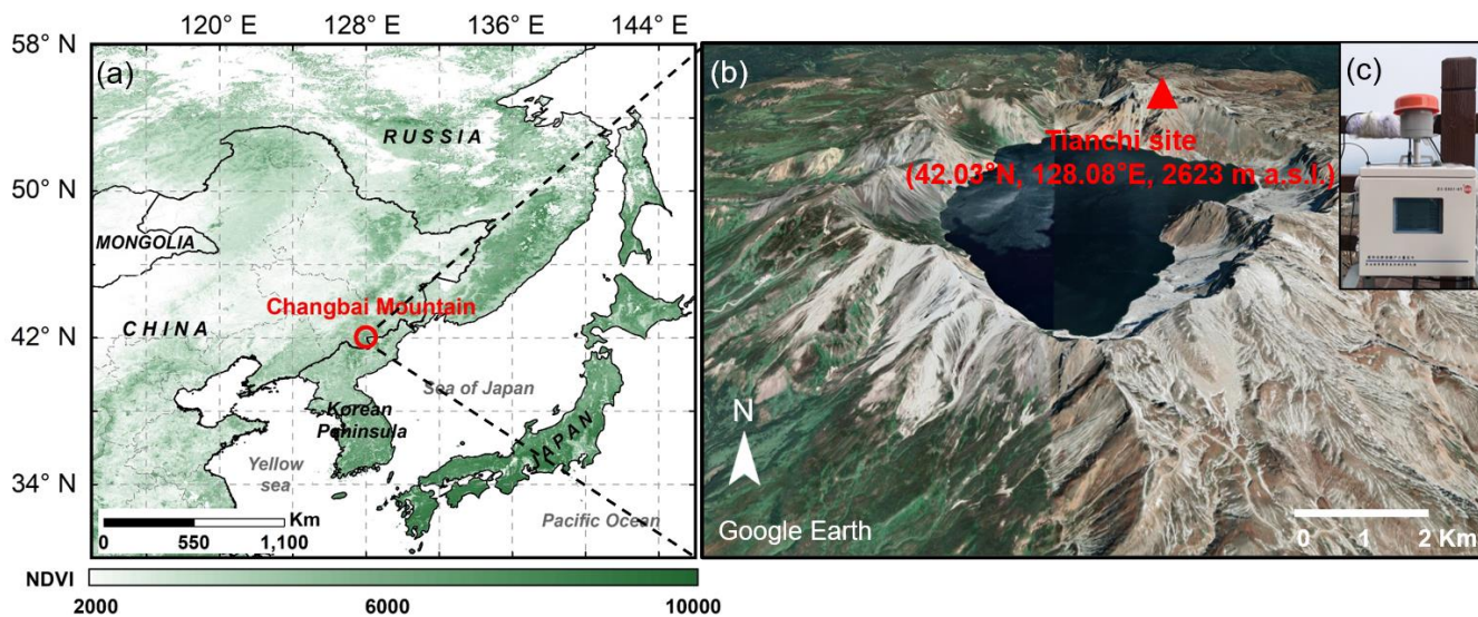
710 Figure 1. Geographical maps showing the location of Changbai Mountain. (a) This map is color-coded according to the normalized difference vegetation index (NDVI) in 2015, which was downloaded from the Geospatial Data Cloud ( https://www.gscloud.cn/search ). (b) This map shows the three-dimensional shape of the sampling site, which was obtained from Google Earth. (c) The ice nuclei sampler (The TH-150D medium flow sampler, Wuhan Tianhong Corporation, China).
