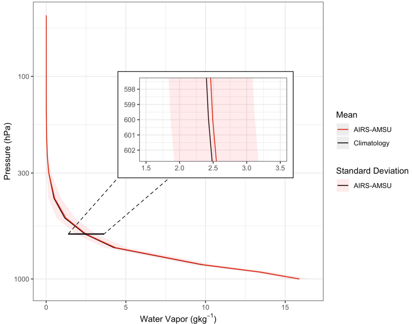
Figure A2. Mean water vapor (in gkg -1 ) reference profiles for the AIRS/AMSU (red line) and the mean climatology AIRS/AMSU profile (black line) for this regime. Also shown is the profile of the standard deviations of all the analogue differences (versus the reference profiles) from the AIRS/AMSU (red shading) analogues.
