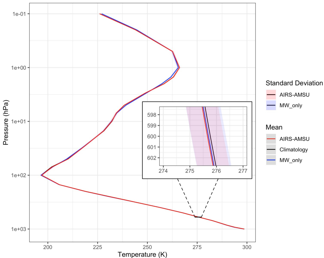
235 Figure A1. Mean temperature (in K) reference profiles for AIRS/AMSU (red line) and MW-only (blue line) retrievals, together with the mean climatology AIRS/AMSU profile (black line) for this regime. Also shown are the profiles of the standard deviations of all the analogue differences (versus the reference profiles) from both the AIRS/AMSU (red shading) and MW-only (blue shading) analogues.
