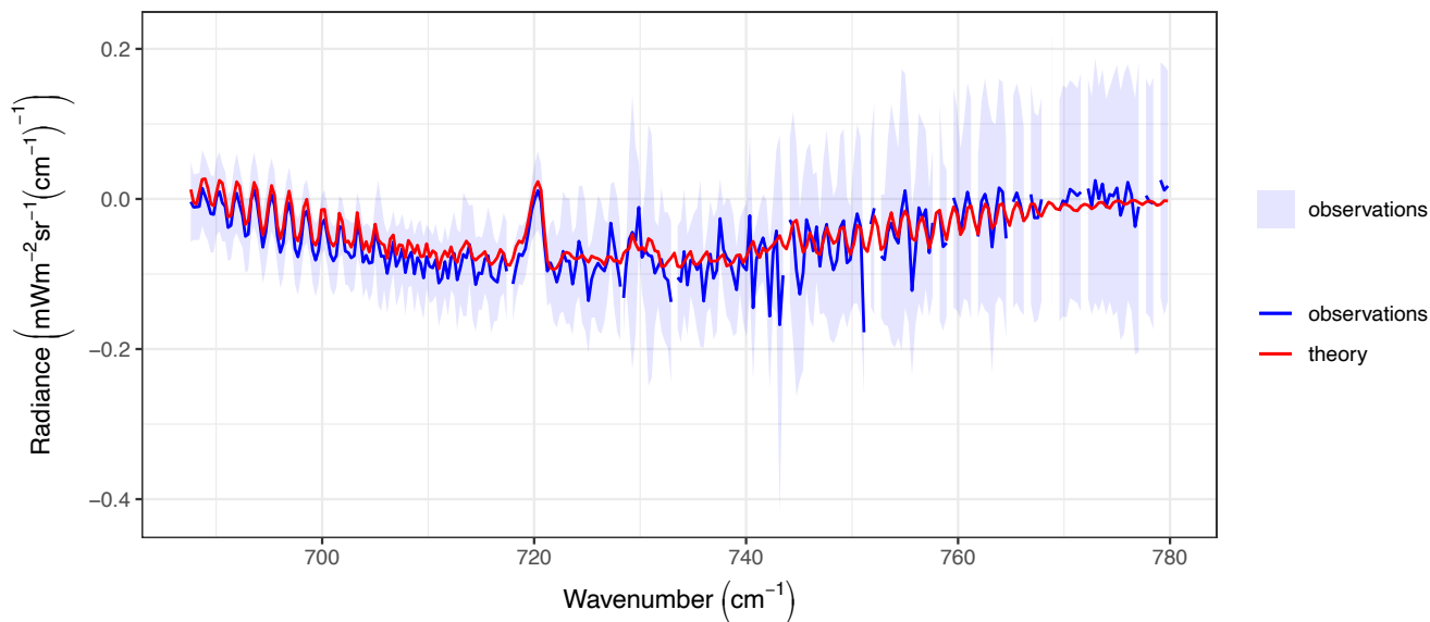
160 Figure 2: Annual mean radiance differences (in mWm -2 sr -1 (cm -1 ) -1 ) due to CO 2 increase, from the AIRS observations (blue line) and from theory (red line), and standard deviations for the AIRS observations (blue shading), following the methodology described and illustrating the direct impact of CO 2 increase on the spectral radiances during the 2003-2012 period (see text for details). Based on observations with scan-angle between -5° and 5°.
