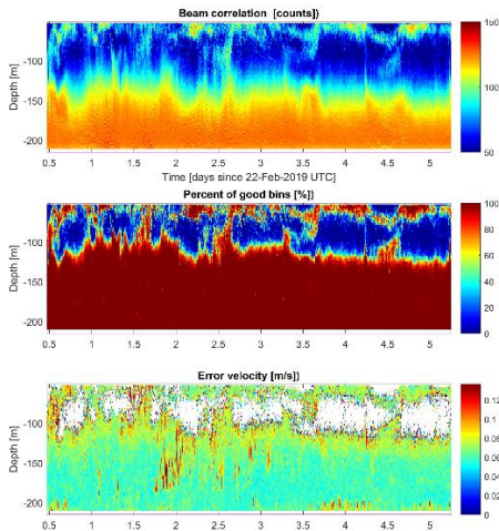
Figure S3: Validation parameters of mooring ADCP deployed during EL19.
