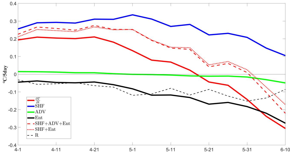
Figure 3: Contribution of different processes to the temperature variation of the warm pool mixed layer in the AS (°C/5 day), where \frac{\partial T}{\partial t} (solid red line) is the temperature variation of the warm pool mixed layer with time, SHF (solid blue line) represents the sea surface heat flux forcing, ADV (solid green line) represents the horizontal advection, ENT (solid black line) represents the
