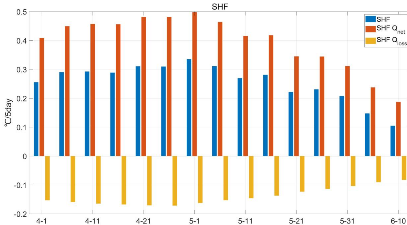
Figure 4: Contribution of the sea surface heat flux forcing to the mixed layer temperature ( ^{\circ}\text{C}/5 day), where blue bars represent the total sea surface heat flux forcing, red bars represent the contribution of the net surface heat flux, and yellow bars represent the contribution of penetrating shortwave radiation at the bottom of the mixed layer.
