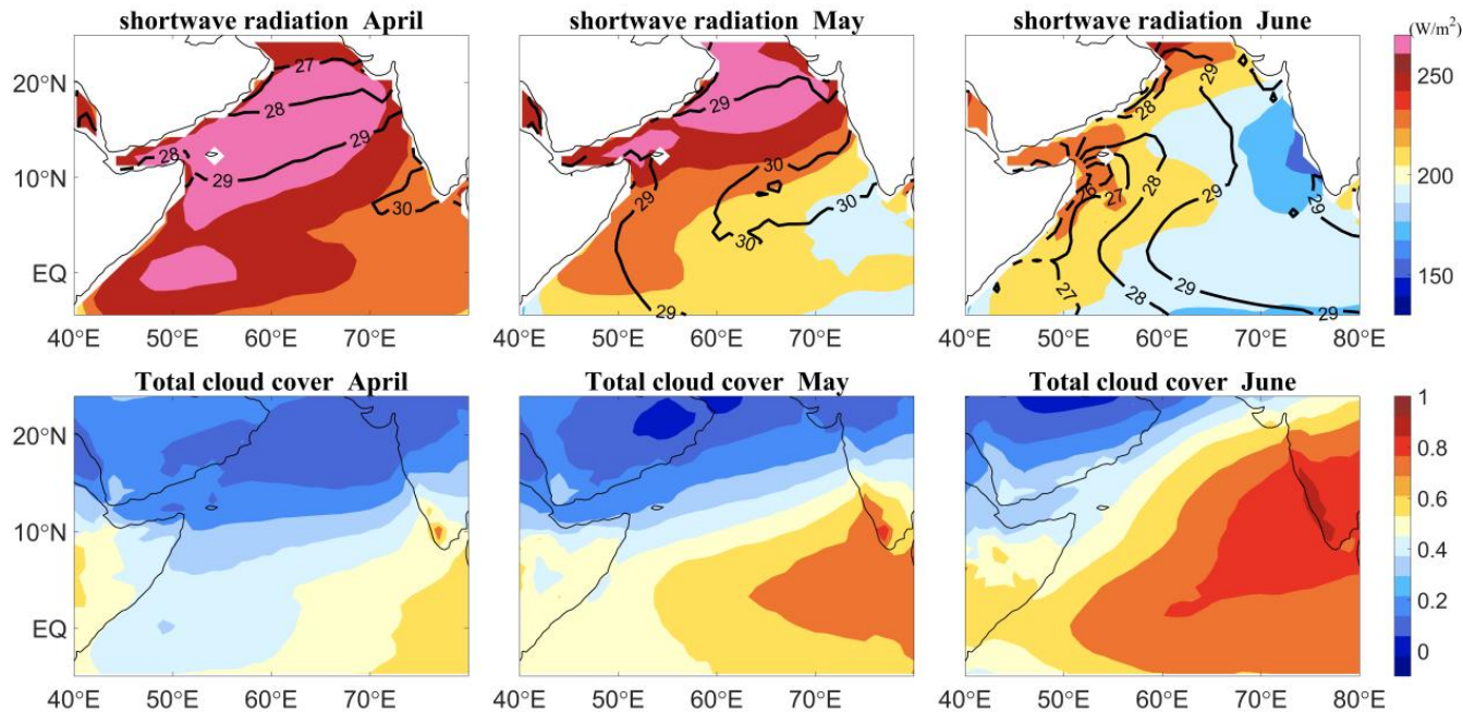
Figure 5: The upper panel: Monthly climatology of shortwave radiation flux (shading; W/m^2 ) and mixed layer temperature (black contours; ^{\circ}C ). The lower panel: the distribution of total cloud coverage.
