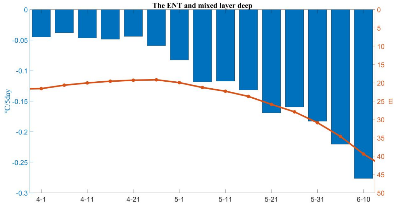
240 Figure 7: Variation of the vertical entrainment and mixed layer depth, where the blue bars represent the vertical entrainment (°C/5 day) and the red line represents the mixed layer depth (m). 删除: s
