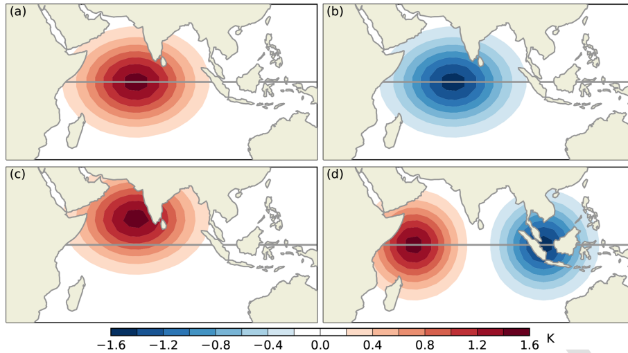
Figure 1. SST biases (in K) used in the sensitivity experiments: (a) EXP_POS, (b) EXP_NEG, (c) EXP_10N, and (d) EXP_IOD. The grey line marks the Equator.
