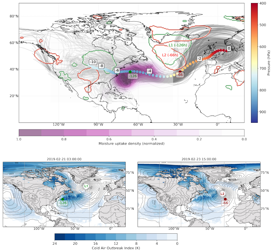
Figure 10. Same as Fig.9 but for trajectories that do not cross into the quadrant to the southeast of latitude of 30°N and longitude of 50°W.
