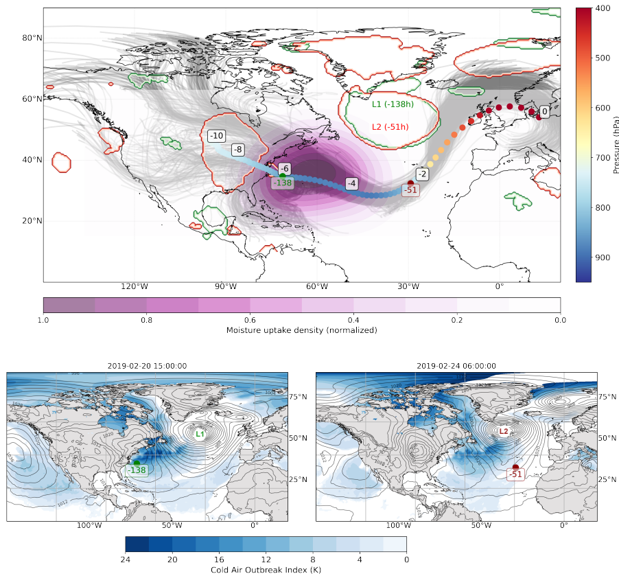
Figure 9. 10-day backward trajectories initialized on 26 February 2019 at 09:00 UTC. (a) Colored dots represent the mean location and pressure (hPa) of trajectories crossing the latitude of 30°N and longitude of 50°W (to southeast), while light grey lines represent individual trajectories used for the calculation of the mean. Black labels mark days prior to arrival in the upper-level NPVA. The green dot (with its corresponding green label) indicates the average moisture uptake time (in hours) for the displayed trajectories, and the green contours outline cyclones present at that moment. The red dot (with its corresponding red label) indicates the average time of start of ascent (in hours) for the displayed trajectories, and the red contours outline cyclones present at that moment. Purple shading represents the normalized (0-1) density of the trajectory positions at the time of most intense moisture uptake. (b) Cold Air Outbreak Index (K) (shading) and mean sea level pressure at the average time of most intense uptake (-138 h), (c) same as (b) but for the average time of start of ascent (-51 h).
