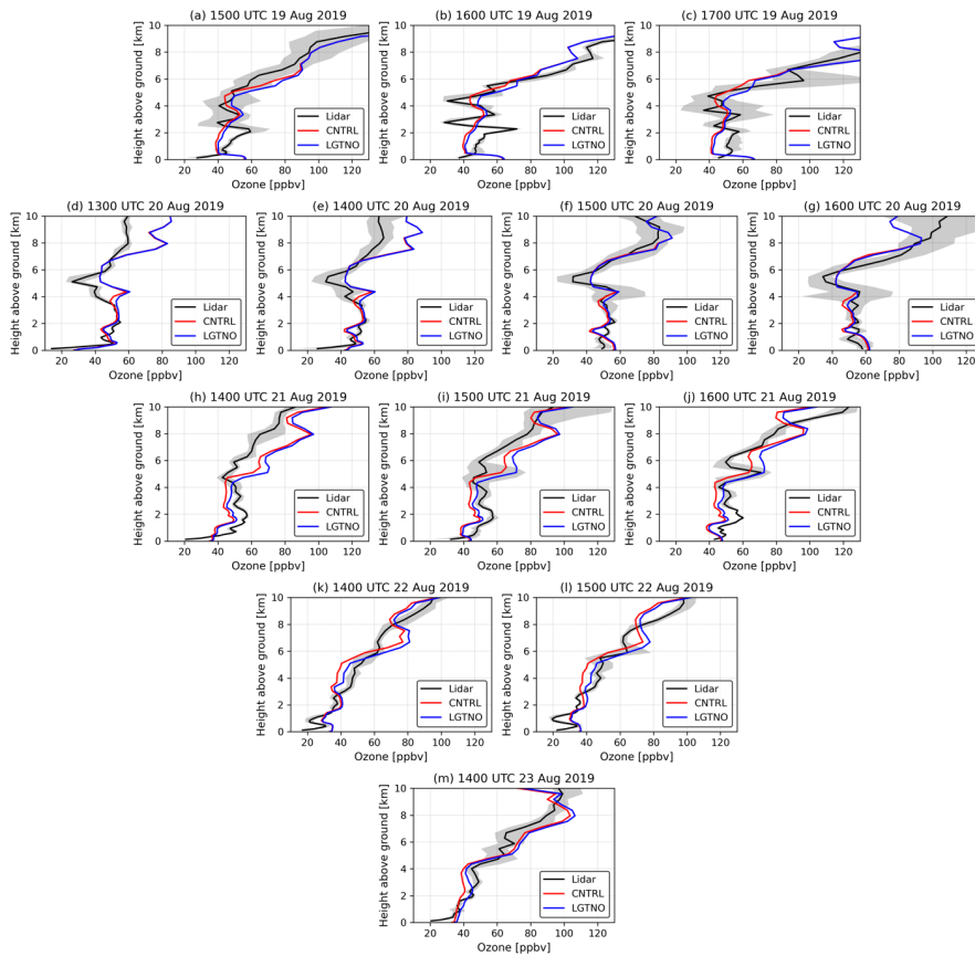
820 Figure 8: Hourly mean lidar-measured and model-simulated ozone profiles at Huntsville, AL, for all lidar observation periods between 19 and 23 August 2019. Black lines represent lidar observations after being averaged hourly and vertically to match the model resolution. Shaded regions indicate ranges of lidar measurements within each hour for each model layer. The red and blue lines represent model predictions of the CNTRL and the LGTNO, respectively.
