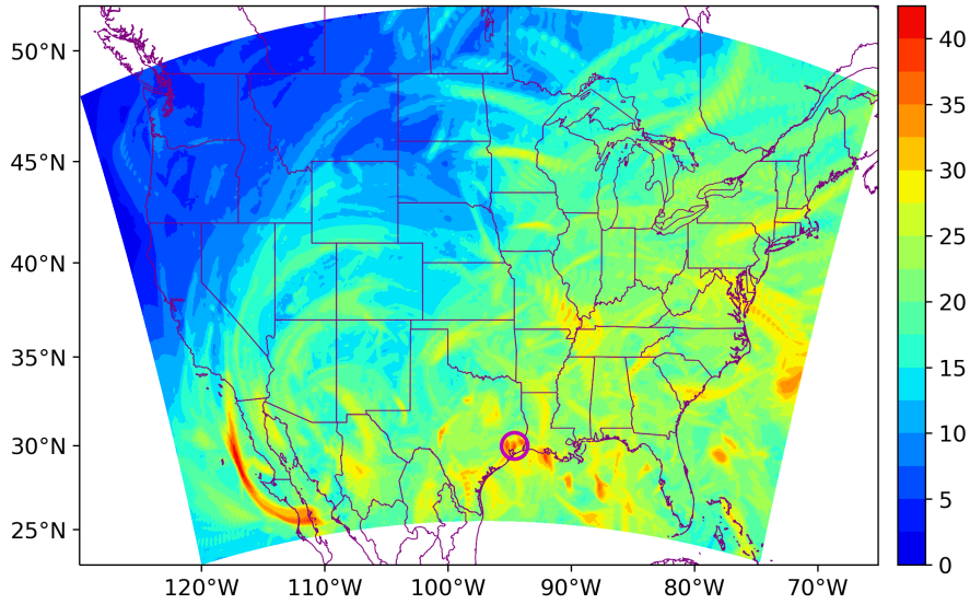
835 Figure 10: Spatial distribution of maximum ozone enhancement (entire simulation and all grid cells) within the troposphere due to LNO emission. The case of interest showing a ~38.6 ppbv ozone increase occurred at 2100 UTC on 29 June 2019 at 29.97°N, 94.58°W (located between Houston, TX, and Beaumont, TX, highlighted by the magenta circle) at ~5.9 km above ground level.
