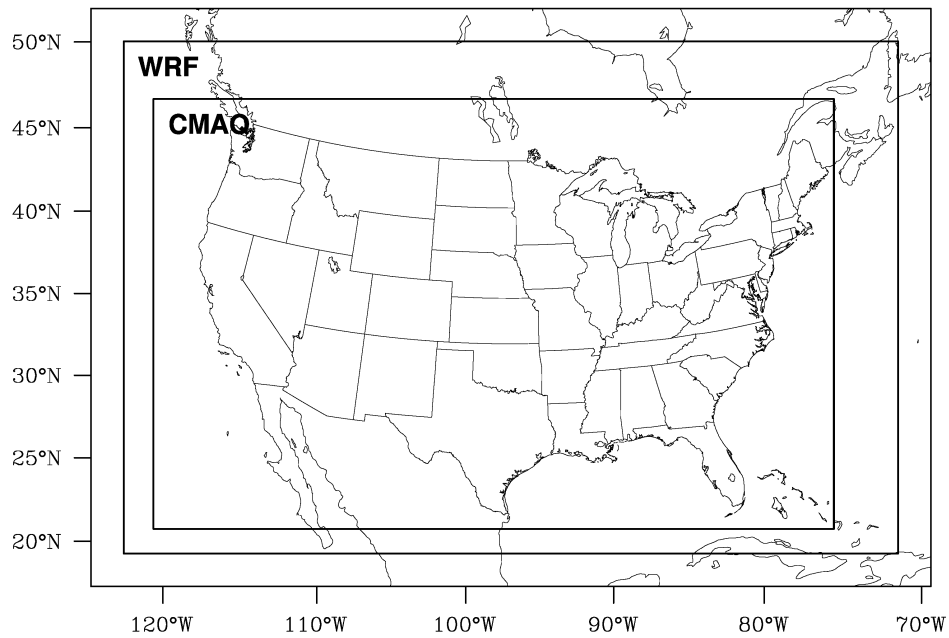
Figure 1: WRF and CMAQ model domain.
