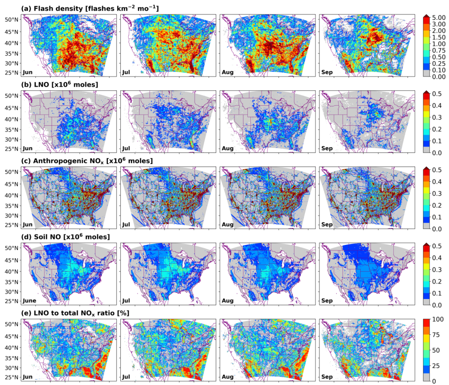
785 Figure 2: Spatial distribution of monthly flash density and NO x emissions from lightning, anthropogenic, and soil sources for June through September 2019. (a) Total flashes per km 2 per month; monthly total NO x emissions (in 10 6 moles) from (b) lightning, (c) anthropogenic, and (d) soil sources per model grid cell (12 km × 12 km, or 144 km 2 ); (e) the ratio of LNO to total NO x emissions.
