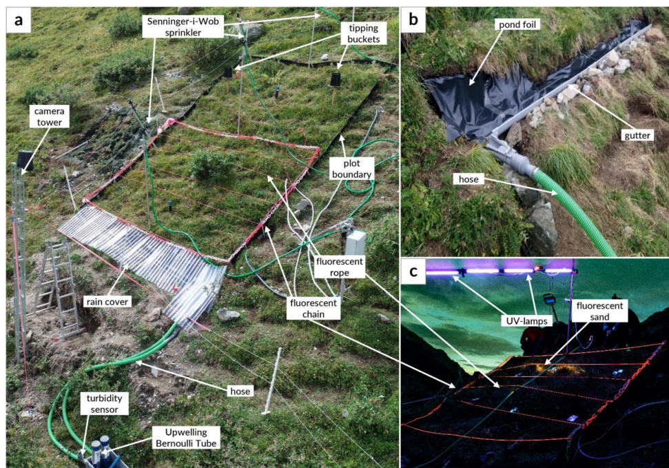
1000 Figure 2: Photos showing the experimental set-up for the study plots (a), the collection system for overland flow (OF), biomat and very shallow subsurface flow (b), and the set-up for the fluorescent sand imaging (c). Important components, such as the plot borders, sprinklers, tipping bucket rain gauges, pond foil, gutter and hose, turbidity sensor, Upwelling Bernoulli Tube, fluorescent segmented chain and fluorescent ropes, and camera tower below the plot are marked and labeled. At night UV lamps were used to illuminate the fluorescent sand on the plot (c).
