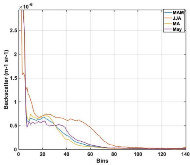
Both VDR and backscatter profile for MAM, JJA MA (without May) and May. 1 bin = 60m
