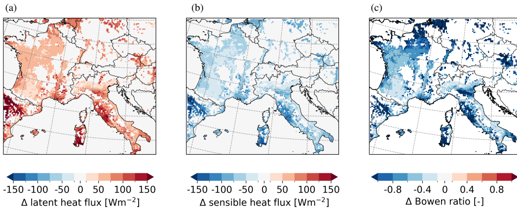
Figure 9. Effects-Irrigation effects based on the difference between the simulation with irrigation (S1) and the simulation without irrigation (S0) on surface fluxes as spatial distribution of means for AMJ for a) latent heat flux, b) sensible heat flux, and c) Bowen ratio shift.
