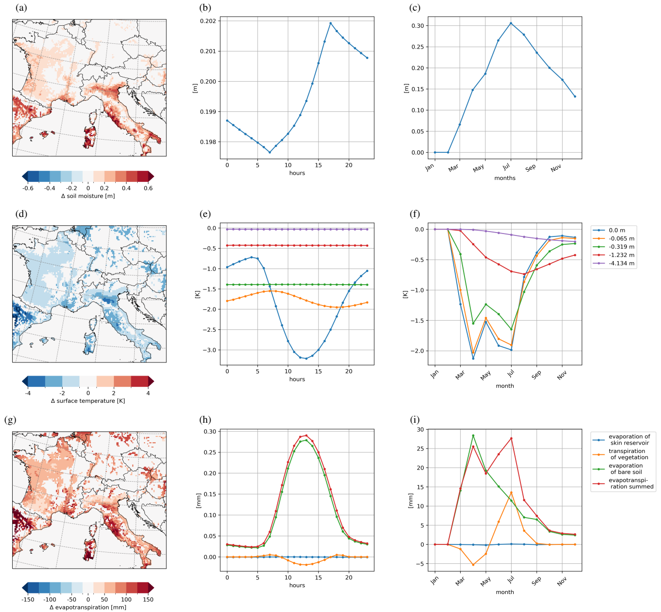
Figure 8. Effects Irrigation effects based on the difference between the simulation with irrigation (S1) and the simulation without irrigation (S0) on soil and surface processes on the irrigated fraction a,d,g) as spatial distribution of mean values of AMJ, b,e, h) as diurnal cycle of mean values of irrigated areas in AMJ, and c, f, i) as annual cycle of mean values of irrigated areas for a-c) soil moisture, d-f) soil temperature in different depths, g-i) evapotranspiration fractions.
