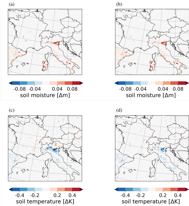
Figure A4. Differences between water application schemes in June 2017 for a) and b) soil moisture, c) - d) surface temperature between a) and c) flextime-prescribed flextime-prescribed schemes, b) and d) adaptive and prescribed scheme.
