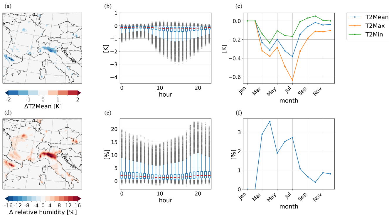
Figure 11. Effects-Irrigation effects based on the difference between the simulation with irrigation (S1) and the simulation without irrigation (S0) on the atmosphere above irrigated areas as a and d) spatial distribution of mean values of AMJ, b and e) mean diurnal cycle of mean values in AMJ with the box spanning from the 1st to the 3rd quartile, the red line showing the median, the whiskers showing the 5th and 95th percentile, and outliers as values outside of these limits, and c and f) as annual cycle of mean values for a-c) 2 m temperatures and d-f) 2 m relative humidity.
