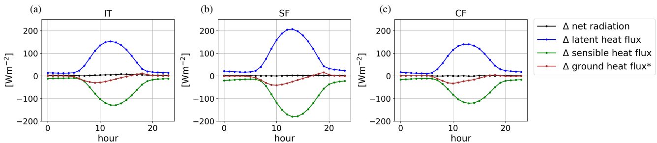
Figure 10. Effects-Irrigation effects based on the difference between the simulation with irrigation (S1) and the simulation without irrigation (S0) on the surface energy balance of the irrigated fraction as hourly mean values of AMJ in the analysis regions a) IT, b) SF, and c) CF.
