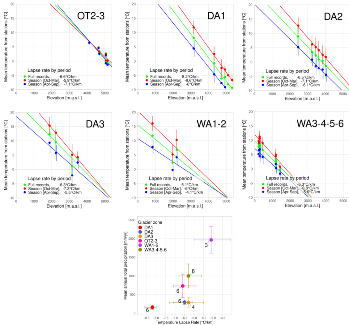
Figure S1. Temperature lapse rates at glaciological zone scale using meteorological records at monthly time step from 1980 to 2019.
