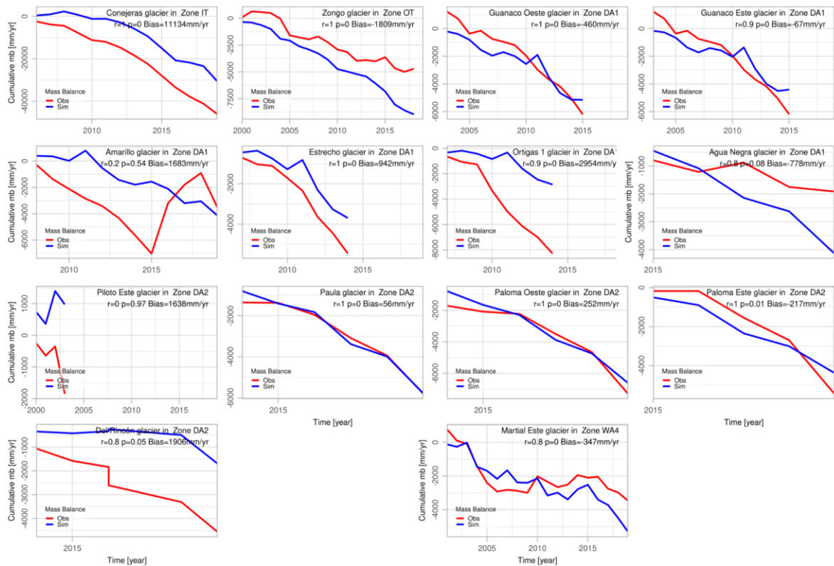
Figure S4. Cumulative mass balance differences between OGGM simulations and observations on 14 glaciers across the Andes (2000-2019).
