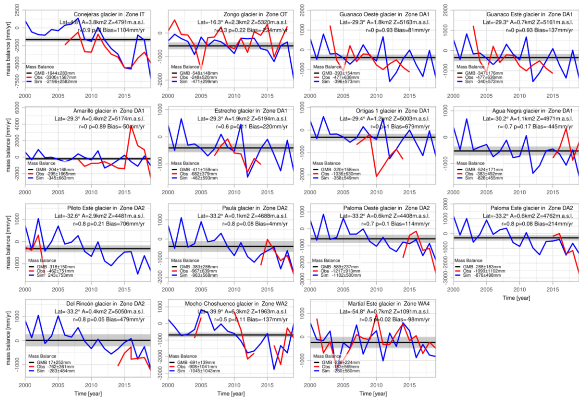
Figure S3. Annual mass balance differences between OGGM simulations and observations on 15 glaciers across the Andes (2000-2019).
