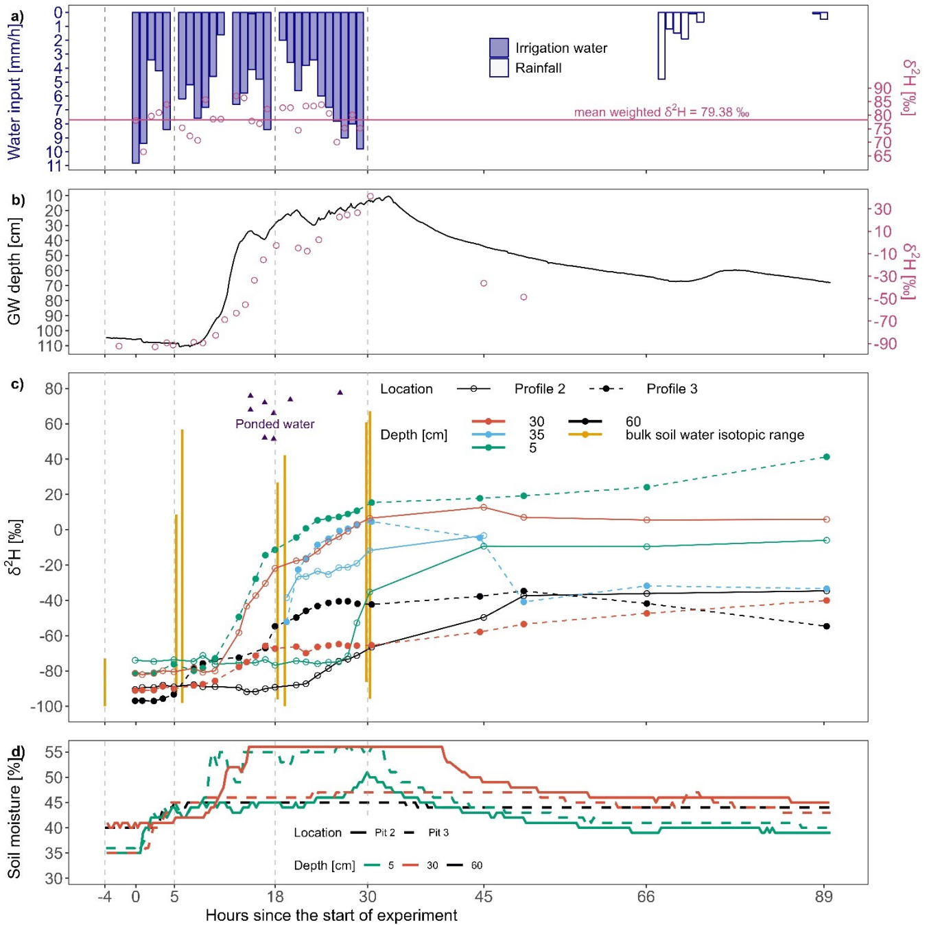
200 Figure 2. Soil water dynamics during the irrigation experiment. (a) Hourly water input intensity (bars). The dots show \delta^2\text{H} values of irrigation water and the vertical dashed grey lines indicate the timing of bulk soil sampling; (b) Groundwater table dynamics, dots representing \delta^2\text{H} values of groundwater; (c) Soil water \delta^2\text{H} signal. Suction lysimeters are at 5, 30 and 60 cm depth. The blue lines and dots (35 cm depth) show pan lysimeter data, the orange vertical lines denote bulk soil \delta^2\text{H} variability; (d) Volumetric soil moisture.
