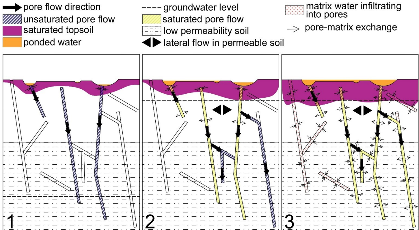
340 Figure 7. Infiltration mechanisms in shallow sub-arctic till soil: (1) the initiation of macropore flow; (2) the development of lateral fluxes; and (3) refilling of soil storage.
