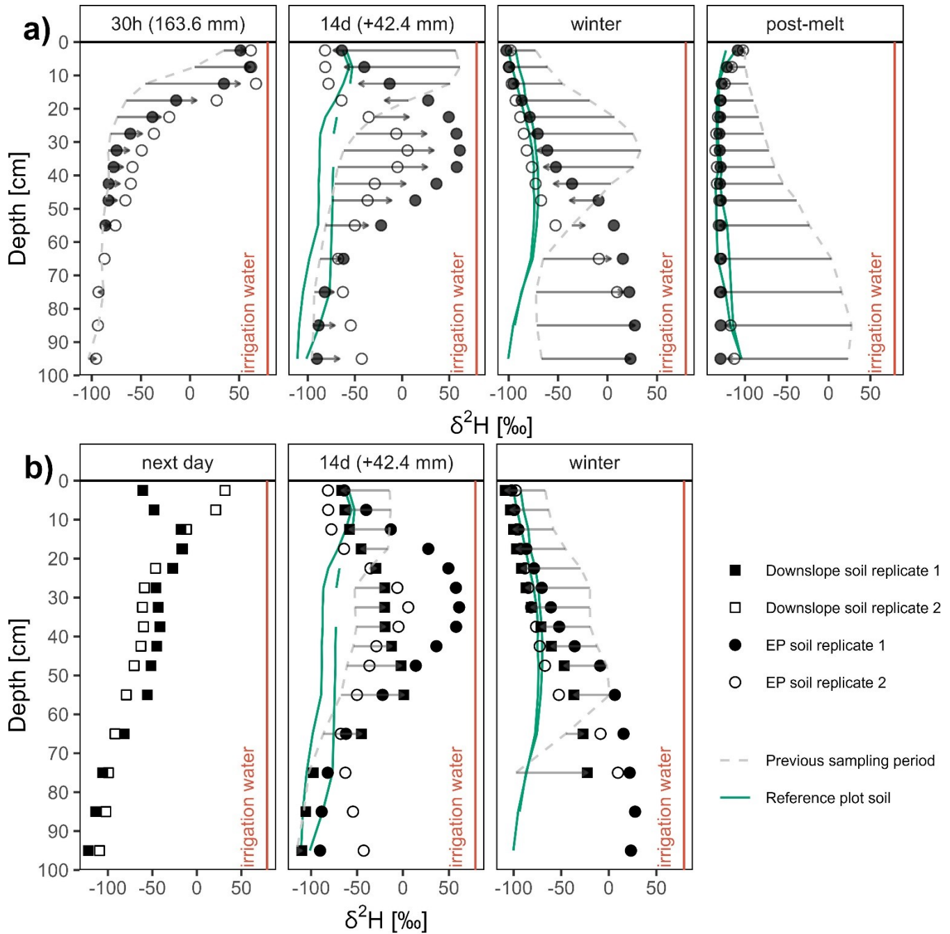
285 Figure 5. Bulk soil water \delta^2\text{H} dynamics after the experiment in the (a) Irrigation plot, and (b) in soil immediately downslope of the EP. Green lines show bulk soil water dynamics in a nearby reference plot, collected at the same time. The isotopic change between the mean values of current isotopic profiles (dots) and the previously sampled (dashed line) mean isotopic profile in the EP are indicated using arrows. Bulk soil \delta^2\text{H} values collected from the EP in the same period are displayed for comparison.
