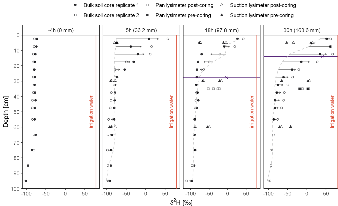
240 Figure 3. Bulk soil water \delta^2\text{H} dynamics during the experiment (dots). Triangles denote soil lysimeter \delta^2\text{H} values collected within 2 hours before (pre-coring) and after (post-coring) bulk soil sample collection. The difference and direction of isotopic changes between the mean values of current bulk soil isotopic profiles and previously sampled (grey dashed line) isotopic profiles are indicated by arrows. The horizontal line shows groundwater level, and groundwater isotopic composition is marked on the line.
