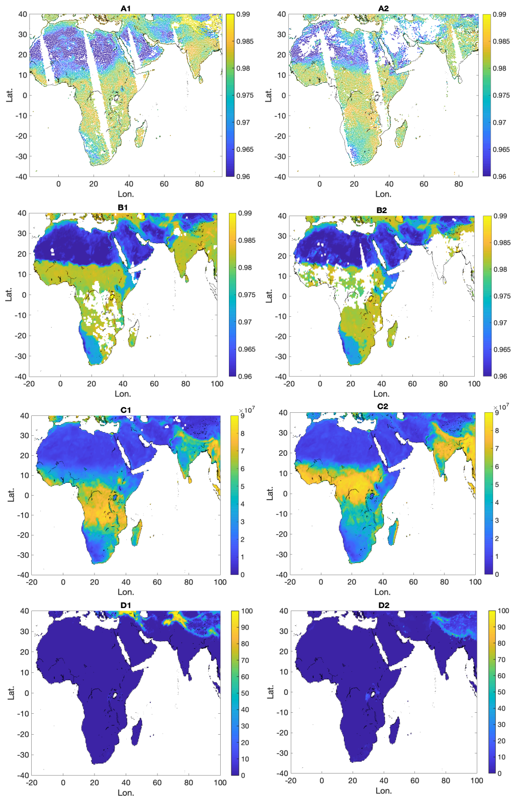
Figure 16 A1 and A2 – SiFSAP surface emissivity at 11 μm for January 14, 2016 and August 9, 2017, respectively; B1 and B2 – MODIS surface emissivity at 11 μm for January, 2016 and August of 2017, respectively; C1 and C2 – MODIS monthly NDVI values for January, 2016 and August of 2017, respectively; D1 and D2 – MODIS monthly snow coverage for January, 2016 and August of 2017, respectively; The area with relatively thicker clouds single (cloud optical depth larger than 1.0) are filtered out in subplots A1 and A2.
