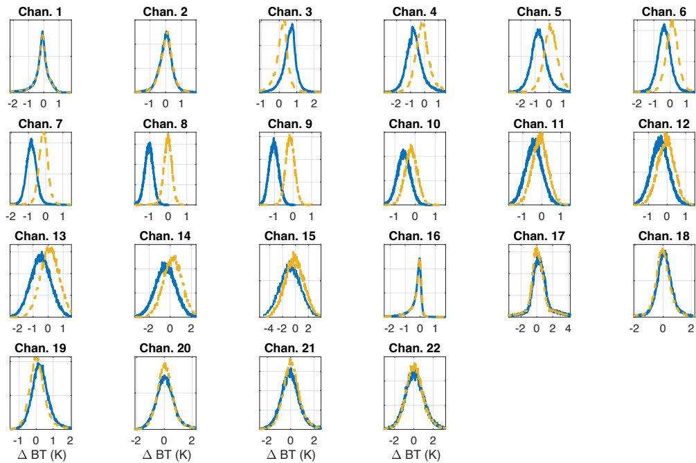
Figure 10 Blue curves: similar to Figure 9 but for histograms that illustrate the distributions of biases in different NOAA20-ATMS channels for over the ocean measurements the 52.725^\circ scan position. Yellow dash curves: histograms of biases after the correction following the regression-prediction scheme.
