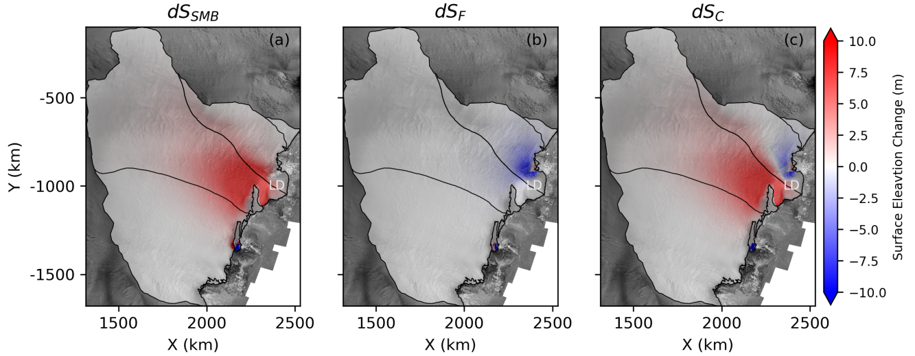
Figure 7. Surface elevation changes ( dS_i ) in the perturbation experiments compared with the control (m) for the 1^\circ\text{C} increase. (a) dS_{SMB} (expSMB 1 ), (b) dS_F (expFriction 1 ), and (c) dS_C (expCombined 1 ).
