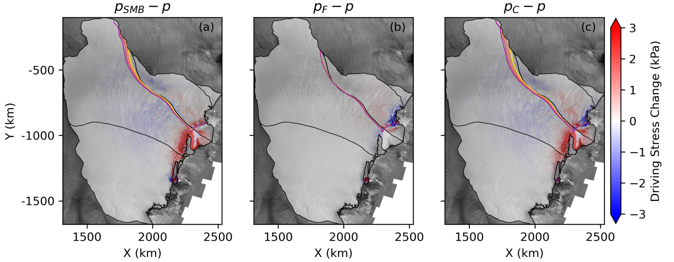
Figure 8. Driving stress changes (kPa) in the perturbation experiments for a 1^\circ\text{C} increase compared with the control (m). (a) dS_{SMB} (expSMB 1 ), (b) dS_F (expFriction 1 ), and (c) dS_C (expCombined 1 ). The contours are the changes in the catchment divides for each of the perturbation experiments for 1 to 7^\circ\text{C} , coloured brightest to dullest (yellow to purple), respectively.
