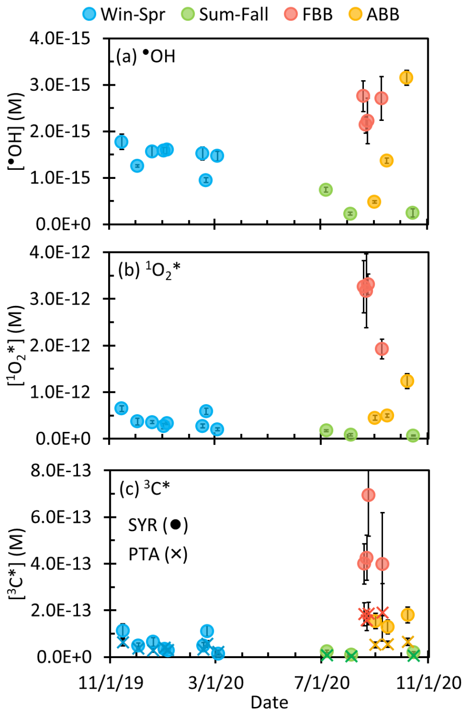
Figure 4. Steady-state concentrations of (a) hydroxyl radical, (b) singlet molecular oxygen, and (c) oxidizing triplet excited states of organics determined by syringol (circles) and (phenylthio)acetic acid (crosses) in particle extracts. Concentrations are all normalized by sampling duration and to midday winter solstice sunlight in Davis to highlight seasonal differences in particle reactivity; the equivalent plots with concentrations calculated for the midday sunlight of each sample collection period is shown in Figure S15. Sample dates are mm/dd/yy.
