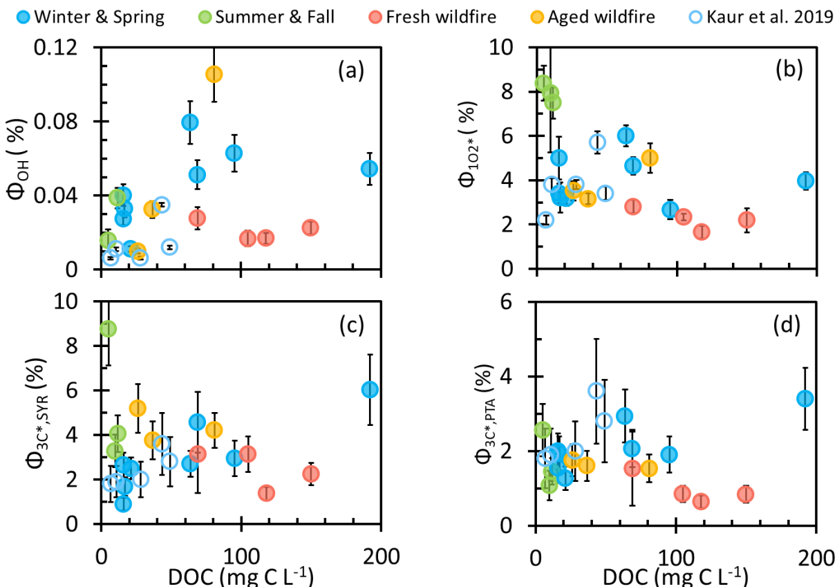
505 Figure 7. Apparent quantum yields of (a) hydroxyl radical, (b) singlet molecular oxygen, and oxidizing triplets determined by (c) syringol and (d) (phenylthio)acetic acid as a function of dissolved organic matter for each sample type (solid circles). Previous measurements made in Davis winter particle extracts are in open circles (Kaur et al., 2019).
