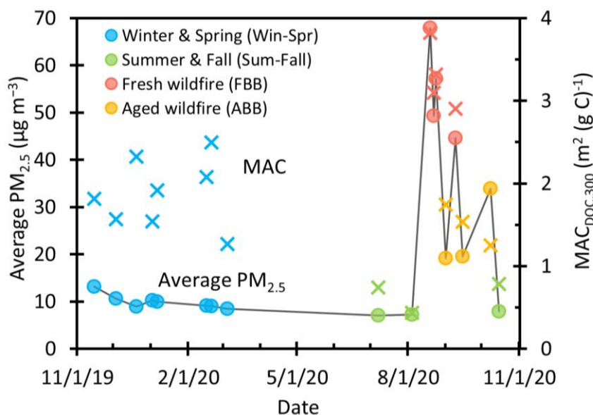
250 Figure 1. Average PM_{2.5} concentrations (circles) during each sampling period and DOC-normalized mass absorption coefficients at 300 nm ( \times ) in particle extracts for Winter & Spring samples (blue), Summer & Fall samples (green), Fresh biomass burning (red), and Aged biomass burning (yellow). The sampling date format is mm/dd/yy, e.g., the first sample was collected on November 15, 2019. PM_{2.5} concentrations were measured roughly 2 km west of our sampling site by the California Air Resources Board and were retrieved from
