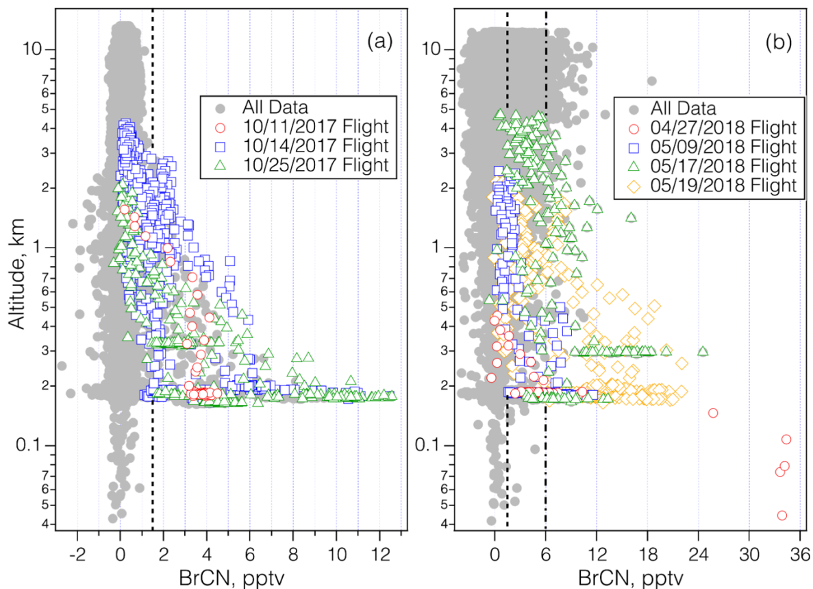
Figure 3. Vertical profiles of BrCN mixing ratios (10 s averages) measured during ATom-3 (panel a) and ATom-4 (panel b). The colored points correspond to the lowest 4 km of altitude profiles that encompassed polar boundary layer dips on dates noted when enhanced BrCN was observed, and the grey points show the remaining observations. The ATom-3 flights took place in October, 2017 and the ATom-4 flights took place in late April through May, 2018. The 10/11/17 flight took place over the Southern Ocean, the 10/14/17 and 5/09/18 flights took place over the Weddell Sea, and 05/17/18 flight took place over Greenland, and the 10/25/17 and 05/19/18 flights took place over the Arctic Ocean. The dotted-dashed line shows limit of detection (LOD) for the flights on May 12, 17 and 21, and the dashed line shows the LOD for the remainder of the flights.
