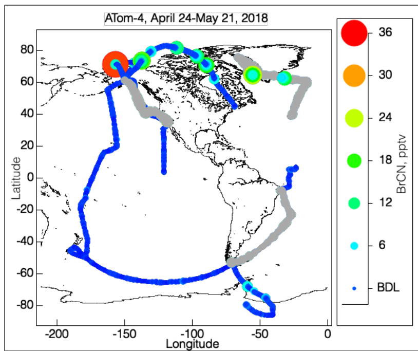
1035 Figure 2. Maps of the BrCN mixing ratios (10s averages) observed during ATom-3 (top panel) and ATom-4 (bottom panel) colored and sized by mixing ratio, as shown by the adjacent scales. The detection limits for most flights were 1.5 pptv, except for the observations made on May 12, 17 and 21, 2018 that had higher detection limit (6pptv) and are shown in grey.
