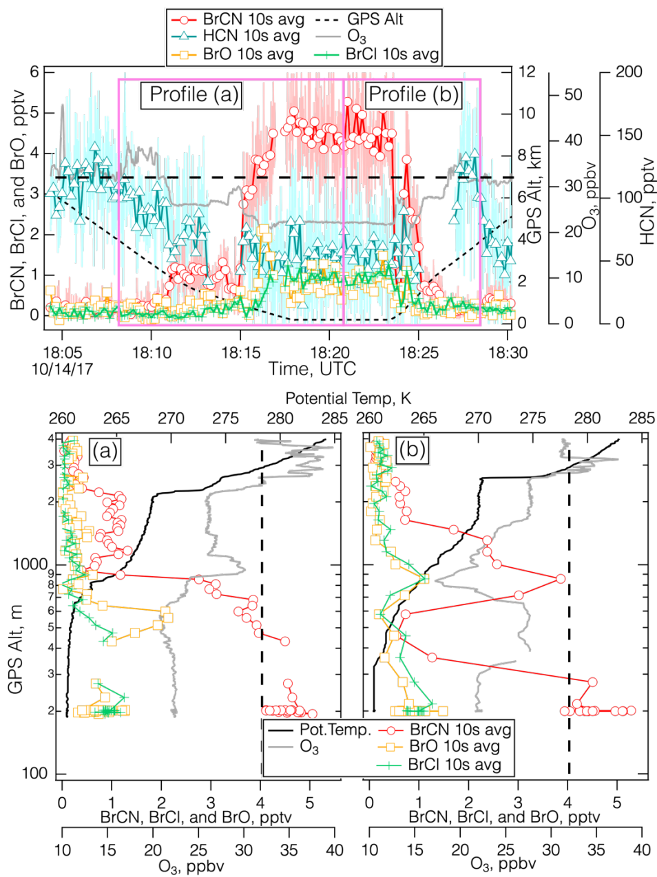
Figure 5. Details of the measurements during the polar boundary layer leg of the Oct. 14, 2017 flight over the Weddell Sea ( 75.7° S Lat, 50.1° W Long ) centered around 18:20 UTC. The top panel shows the time series for BrCN, BrO, BrCl, HCN, O 3 , and altitude, divided into vertical profiles during the descent (Panel a), and the ascent (Panel b), and a dashed line drawn at 32 ppbv O 3 .
