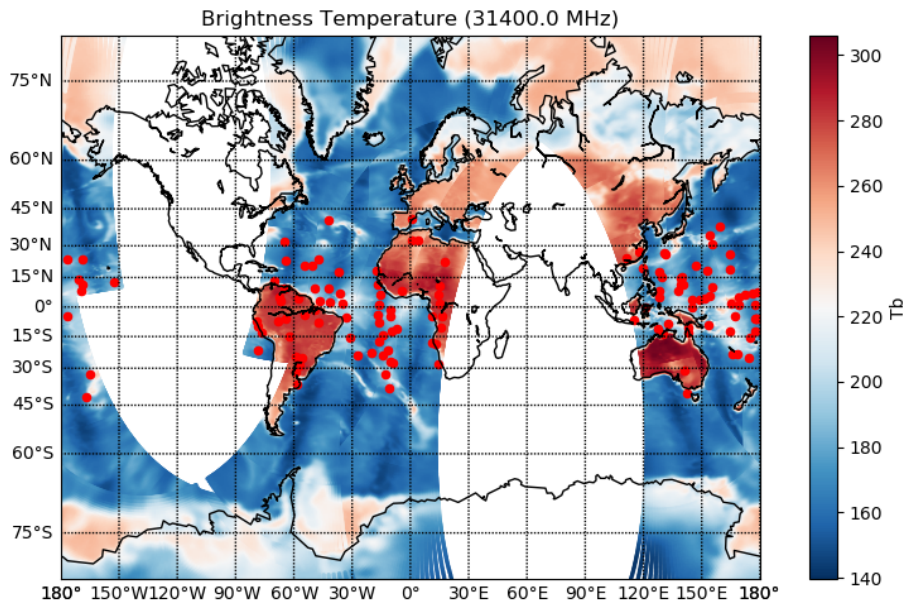
(a) Collocated cases between Suomi-NPP and COSMIC-2 on April 1, 2019, 00:00-06:00 UTC. The red dots are the tangent point location of each COSMIC-2 RO at its lowest penetration height, while the background color is the 31.4 GHz brightness temperature measurement from the onboard ATMS instrument
