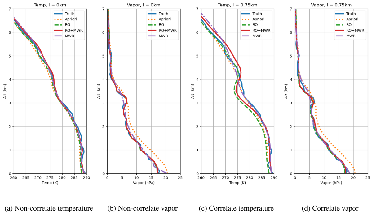
Figure 8. Sensitivity test of the (a, c) temperature and (b, d) vapor retrieval with respect to the off-diagonal term in the background covariance matrix. The diagonal matrix is used for the first two panels (a and b) and the off-diagonal elements are added in the last two (c and d) panels
