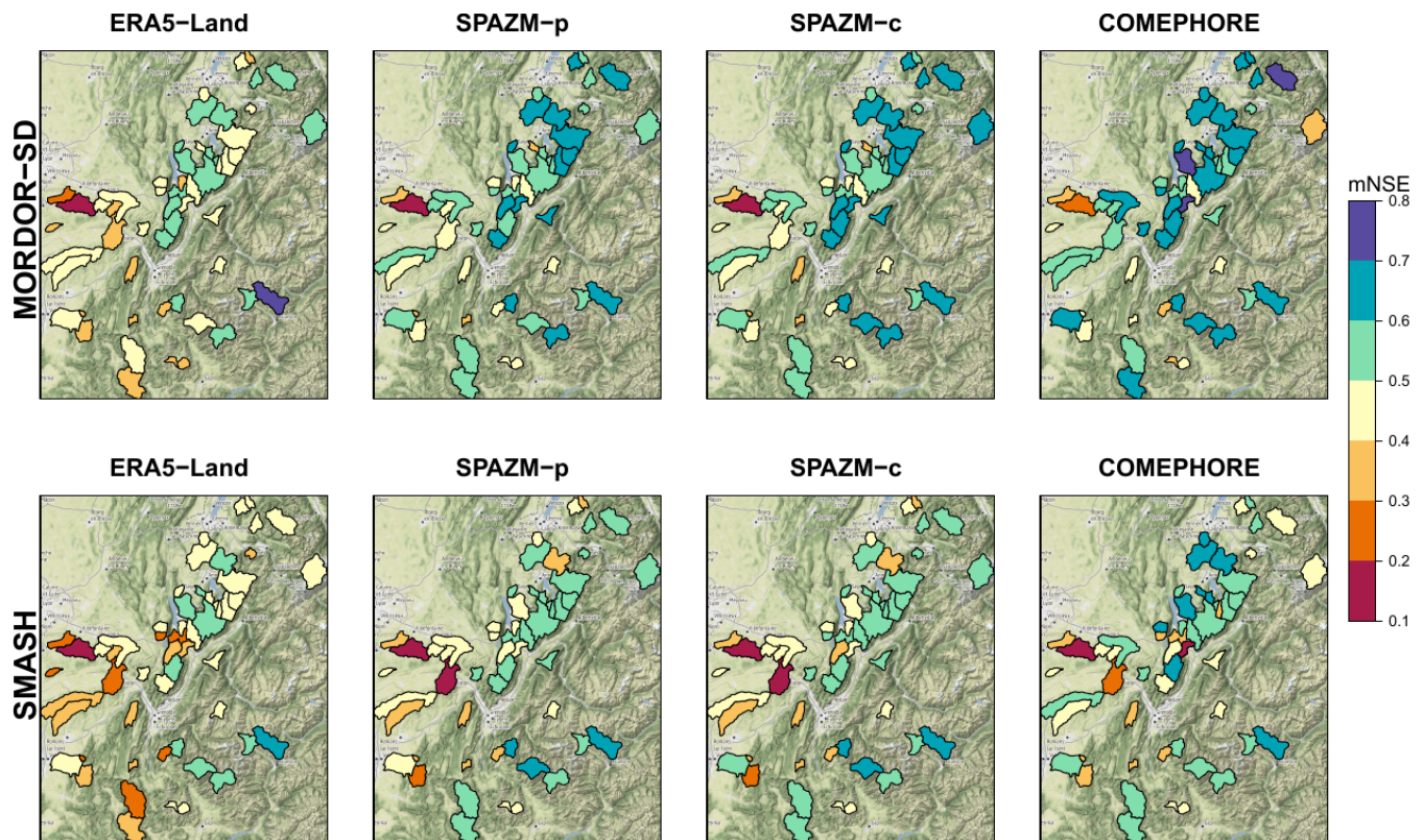
Figure 4. Maps of the mNSE(Q) in winter and spring (DJFMAM) obtained with MORDOR-SD (top row) and SMASH (bottom row) and the four types of precipitation forcings. Map tiles by Stamen Design, under CC BY 3.0. Data by OpenStreetMap, under ODbL.
