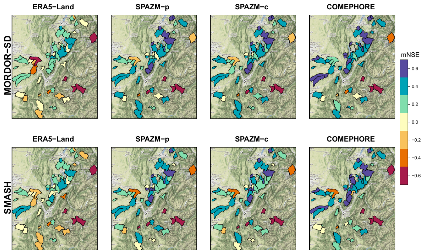
Figure 5. Maps of the mNSE for the 10 largest floods obtained with MORDOR-SD (top row) and SMASH (bottom row) and the four types of precipitation forcings. A few values exceed the lower bound of -0.7 (dark brown). Map tiles by Stamen Design, under CC BY 3.0. Data by OpenStreetMap, under ODbL.
