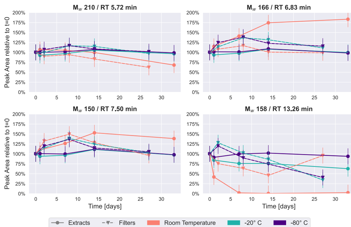
Figure 4: Time series plots of the four most intense peaks in the naphthalene SOA samples. Similar as for b-pinene SOA (Fig. 2), room temperature storage significantly affects the concentration of some compounds in naphthalene SOA.
