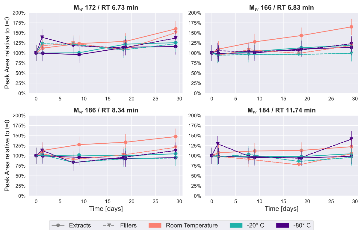
335 Figure 6: Time series of an average of HVAS 2-5 samples of four previously detected peaks in the SOA samples from \beta -pinene ( m/z 171.0663, m/z 185.0819 and m/z 183.1027) and from naphthalene ( m/z 165.0192).
