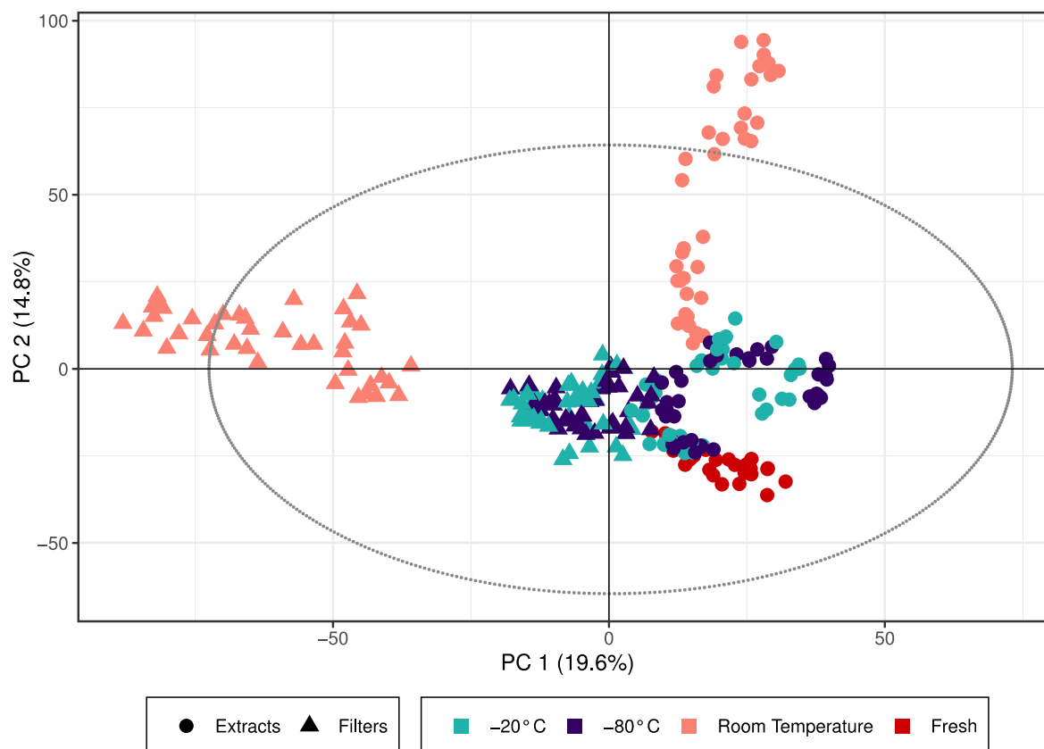
190 Figure 1: PCA scores plot of the \beta -pinene SOA samples. Colors represent storage temperature and the directly analyzed (i.e. fresh) samples and icons indicate the storage type. Hotelling's T2 ellipse (95%) represented by the dotted line. R^2X[1] = 0.196 , R^2X[2] = 0.148 , Q^2[1] = 0.190 , Q^2[2] = 0.176 .
