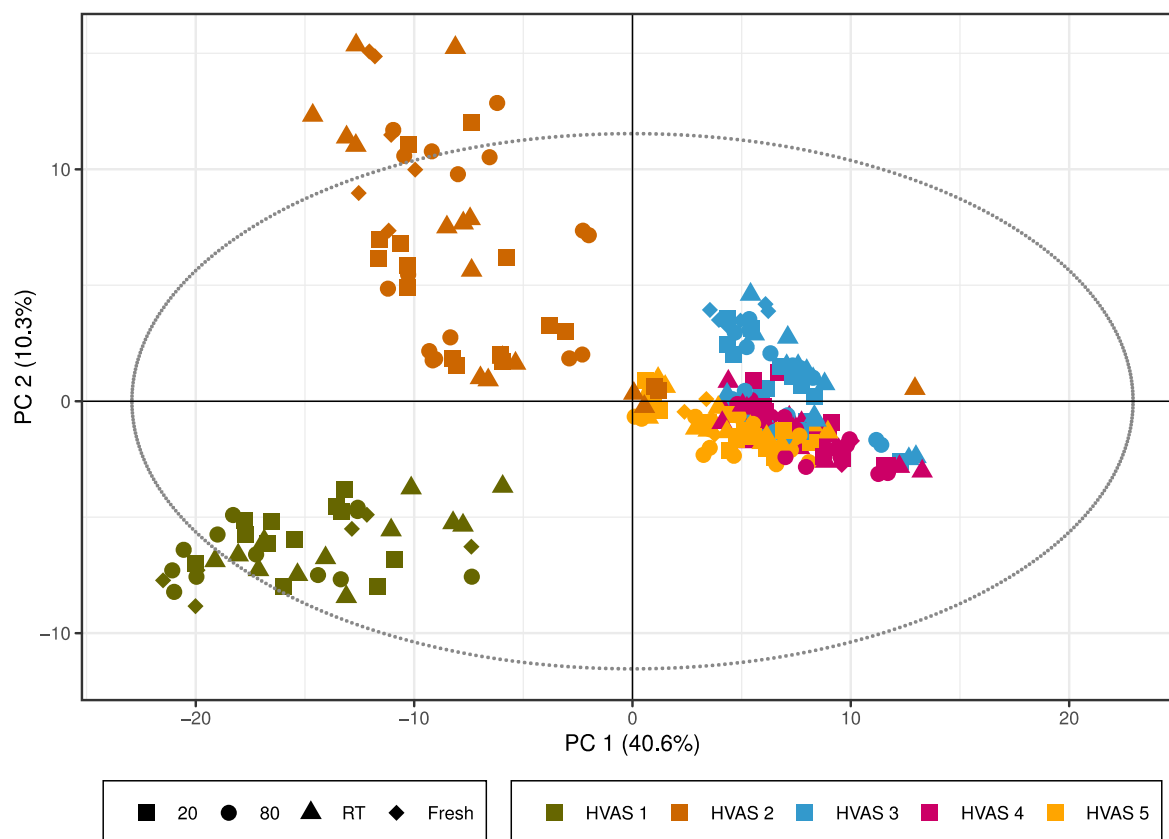
315 Figure 5: PCA scores plot representing the HVAS filters with the exclusion of the batch effect due to different mobile phases. Colors represent the different HVAS filters and shapes the different storage temperatures R^2X[1] = 0.406 , R^2X[2] = 0.103 , Q^2[1] = 0.399 , Q^2[2] = 0.157 .
