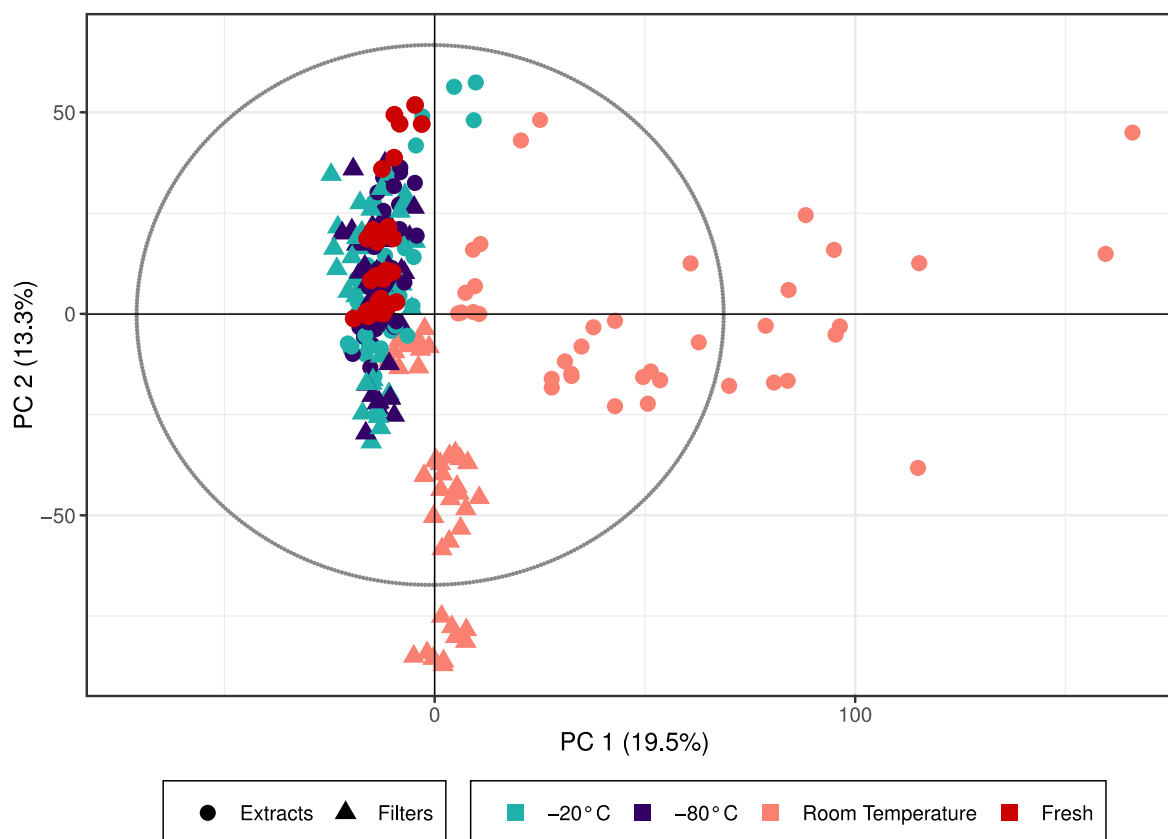
250 Figure 3: PCA scores plot of the naphthalene-SOA samples. Colors represent storage temperature and the directly analyzed (i.e. fresh) samples and icons indicate the storage type. Hotelling's T2 ellipse (95%) represented by the dotted line. R^2X[1] = 0.195 , R^2X[2] = 0.133 , Q^2[1] = 0.135 , Q^2[2] = 0.153 .
