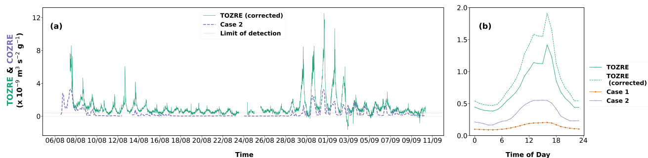
Figure 6. Observation of (a) TOZRE (green) corrected in the presence of a fast reacting compound and case 2 (dashed violet line) of COZRE determined using faster reaction rate. The limit of detection of TORM is also indicated on the graph. (b) Diel plot of TOZRE, TOZRE (corrected), case 1 and case 2.
