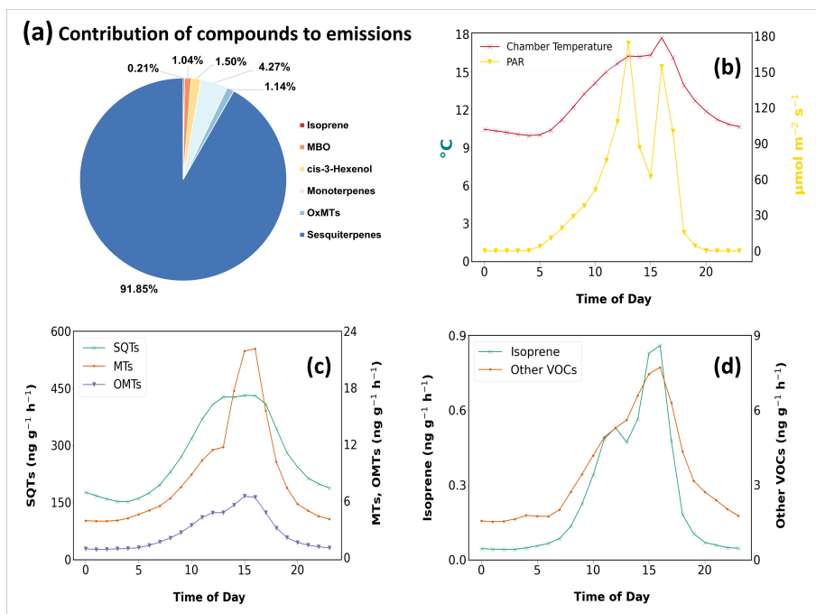
Figure 4. (a) Contribution of observed BVOC to Norway spruce emissions. Mean diel variation in emission rates of (b) chamber temperature and PAR, (c) MTs, OMTs, and SQTs and (d) isoprene and the sum of the rest of BVOCs
