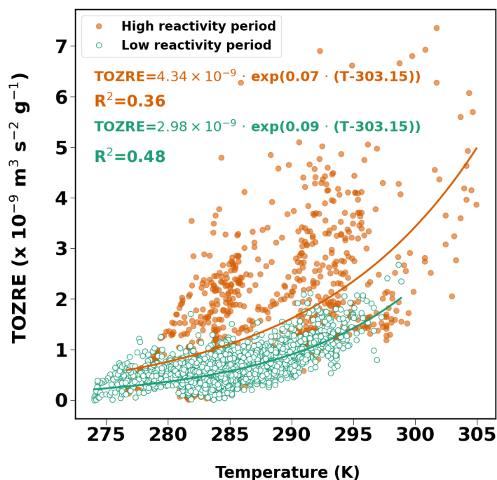
Figure 8. TOZRE as a function of temperature for high reactivity period (orange dots) and low reactivity period (green dots). Red and green lines indicate the exponential fit for the high and low reactivity periods respectively.
