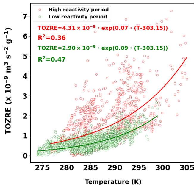
Figure 8. Measured total ozone reactivity as a function of temperature for different periods. TOZRE as a function of temperature for high reactivity period (red dots) and low reactivity period (green dots). Red and green lines indicate the exponential fit for the high and low reactivity periods respectively.
