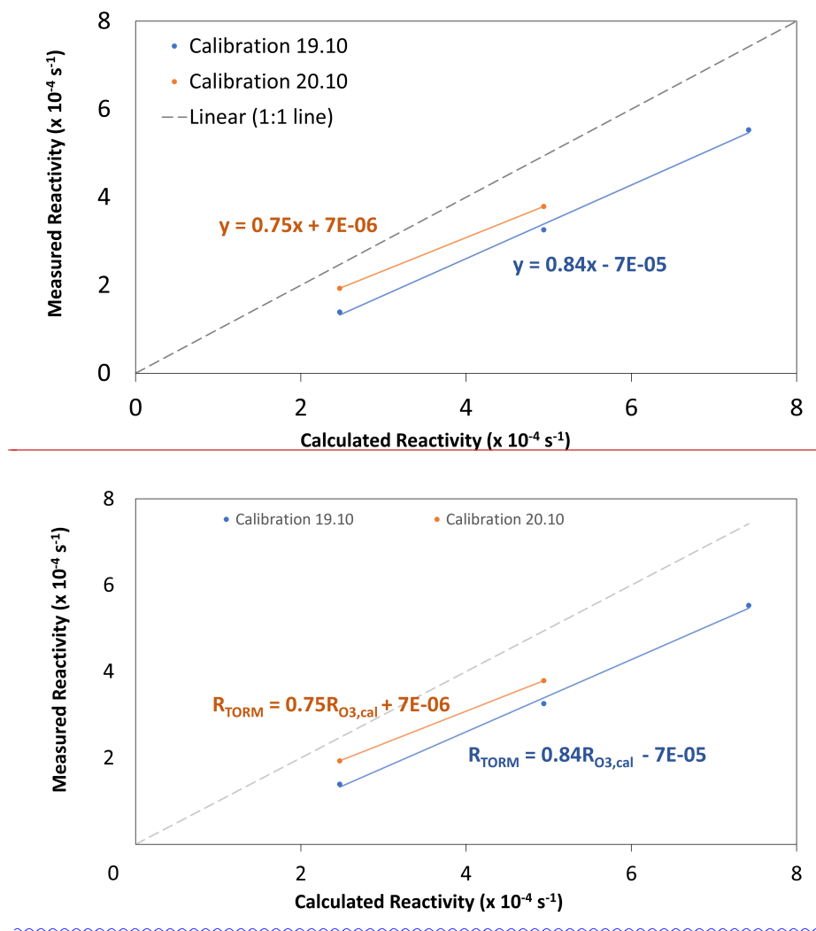
Figure B1. Calibration of the total ozone reactivity monitor. The mean slope and intercept from the two calibration lines were used as the correction factors.
