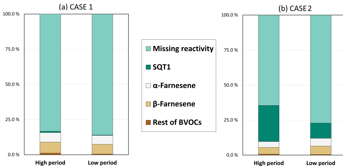
Figure 7. Fraction of various contributions of observed BVOCs and missing fraction to the total ozone reactivity TOZRE for two different cases. (a) Case 1 was calculated after applying the lower slower reaction rate to the unknown sesquiterpene (SQT1). (b) Case 2 was calculated after applying the higher faster reaction rate to the unknown sesquiterpene (SQT1).
