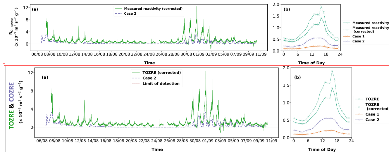
Figure 6. Observation of (a) measured total ozone reactivity (green) corrected in the presence of fast reacting compound and case 2 (dashed violet line) calculated ozone reactivity using higher reaction rate. (b) Diel plot of measured reactivity, measured reactivity (corrected), case 1 and case 2. Observation of (a) TOZRE (green) corrected in the presence of a fast reacting compound and case 2 (dashed violet line) of COZRE determined using faster reaction rate. The limit of detection of TORM is also indicated on the graph. (b) Diel plot of TOZRE, TOZRE(corrected), case 1 and case 2.
