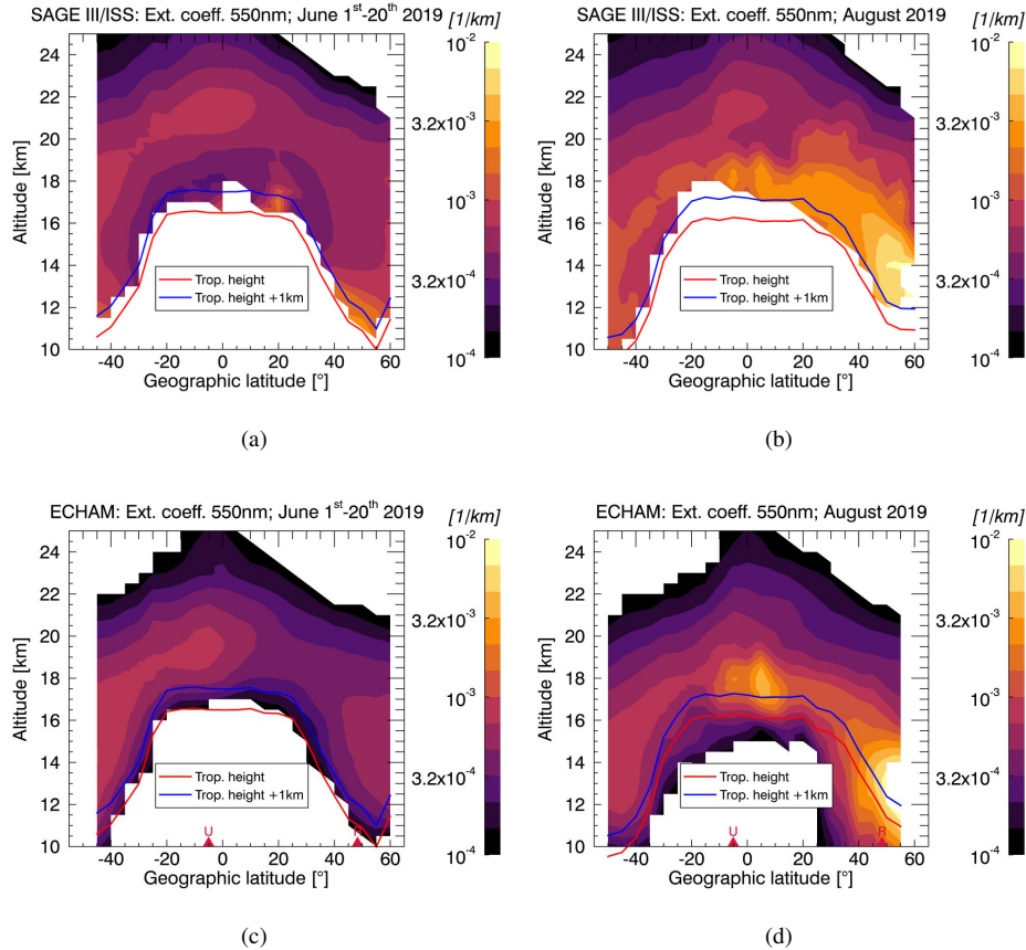
Figure 7. Zonal means of the aerosol extinction coefficient at 550 nm for June 1 st to 20 th (left) and August 2019 (right) from the SAGE III/ISS data set (upper plots) and from the ECHAM simulations using the spatial and temporal sampling of SAGE III/ISS (lower plots). Triangles on the bottom of each plot indicate the volcano’s locations. Tropopause height is illustrated by a red line, with the blue line indicating an uncertainty interval of 1 km above tropopause height.
