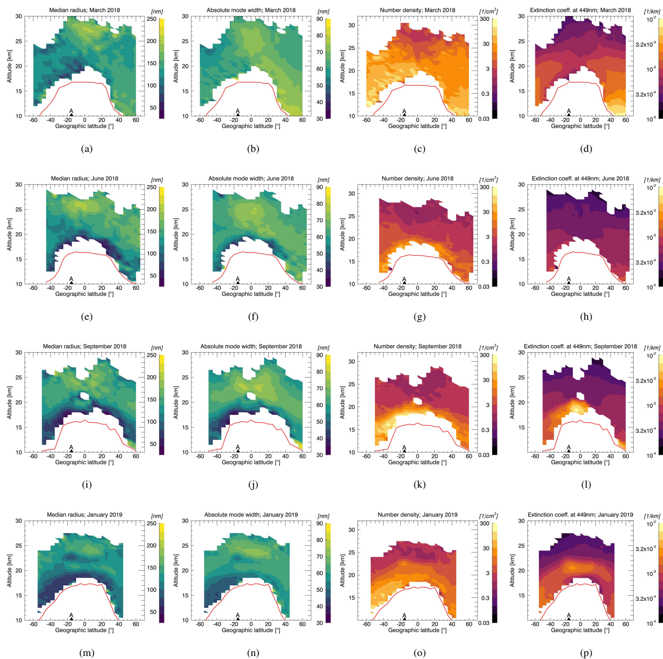
Figure 3. Median radius (leftmost column), absolute mode width \omega (second column), number density (third column) and extinction coefficient at 449 nm (rightmost column) for characteristic months before and after the Ambae eruptions in 2018. The location of the volcano is marked with a triangle and letter on the bottom of each plot and tropopause height is indicated by a red line.
