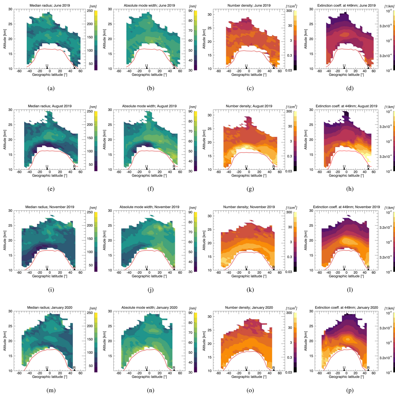
Figure 4. Analogous to Fig. 3 but for the months around the Raikoke and Ulawun eruptions.
