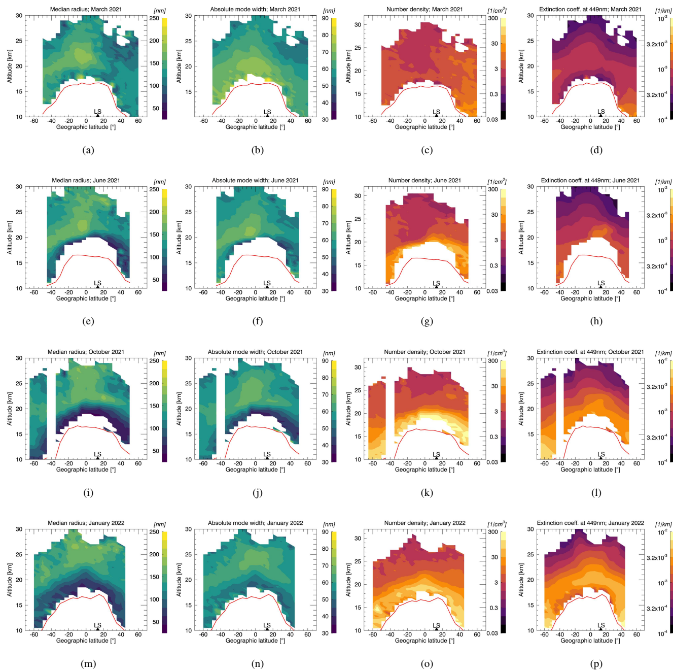
Figure 5. Analogous to Fig. 3 but for the months around the La Soufriere eruption.
