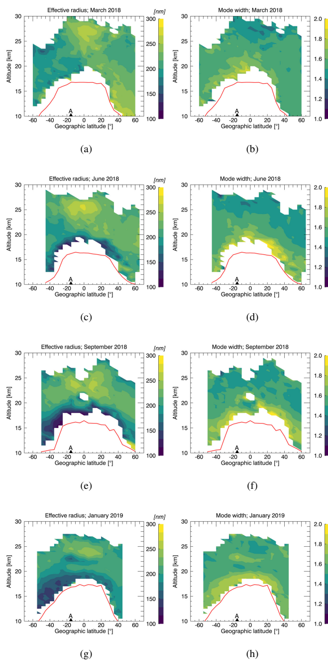
Figure A1. Analogous to Fig. 3, but showing the effective radius and the mode width \sigma for the characteristic months before and after the Ambae eruptions in 2018.
