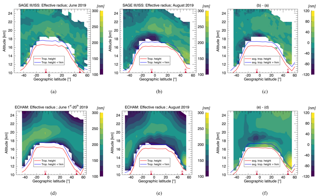
Figure 8. Zonal means of the effective radius retrieved from SAGE III/ISS (upper row) and calculated with the ECHAM model using the spatial and temporal sampling of SAGE III/ISS (lower row) for June 1 st to 20 th 2019 (leftmost column) and August 2019 (middle column). The rightmost column shows the temporal anomaly of the effective radius, i.e. the difference between the first two plots in each row. Triangles on the bottom of each plot indicate the volcano’s locations. Tropopause height is illustrated by a red line, with the blue line indicating an uncertainty interval of 1 km above tropopause height.
