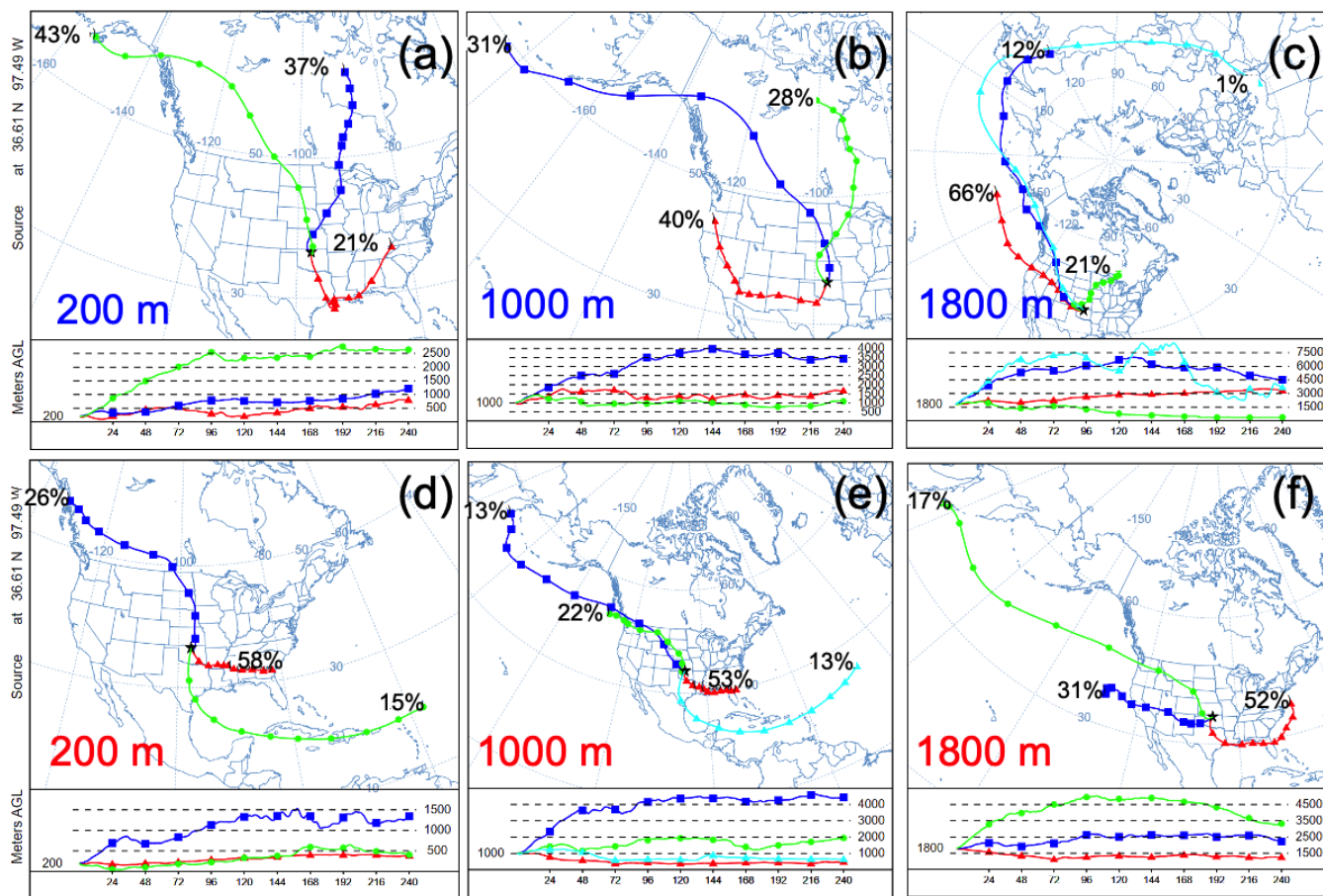
Fig. 3. Cluster analysis of 10-day back trajectories arriving at 200, 1000, and 1800 m above the SGP site during the spring (first row) and summer (second row) IOP campaign. The average trajectories of the clusters are represented by different colors, and the associated numbers denote the occurrence percentages of the clusters.
