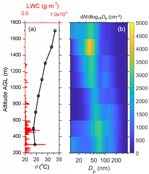
930 Fig. 14. Vertical profiles of parameters during a convective downward transport event over the SGP site on September 10, 2016. (a) Potential temperature ( \theta ) and liquid water content (LWC). (b) Vertical profile of aerosol size distributions as a function of altitude. The particle concentrations, surface area concentrations, and size distributions are normalized to standard temperature and pressure (273.15 K and 101.325 kPa; STP).
