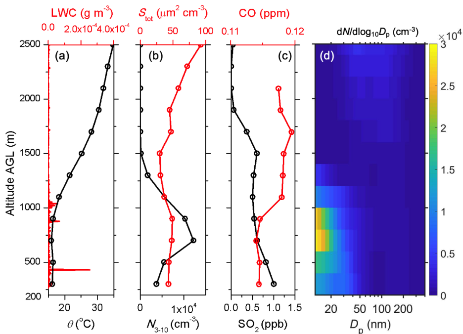
Fig. 8. Vertical profiles of parameters during a NPF event occurring at upper boundary layer over the SGP site on May 14, 2016. (a) Potential temperature ( \theta ) and liquid water content (LWC). (b) Concentration of particles between 3 and 10 nm ( N_{3-10} ) and total aerosol surface area concentration. (c) Mixing ratios of carbon monoxide (CO) and sulfur dioxide ( \text{SO}_2 ). (d) Vertical profile of aerosol size distributions as a function of altitude. The particle concentrations, surface area concentrations, and size distributions are normalized to standard temperature and pressure (273.15 K and 101.325 kPa; STP). Note that \text{SO}_2 mixing ratio is corrected by a constant offset so that the minimum mixing ratio value is set to 0.
