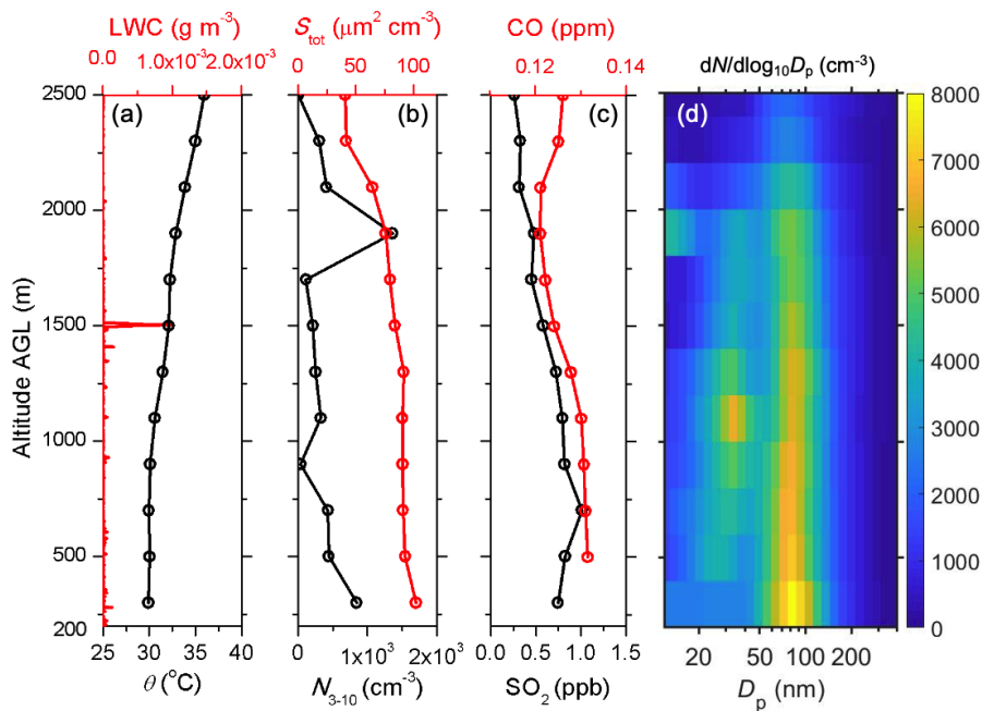
895 Fig. 9. Vertical profiles of parameters during a NPF event occurring in the free troposphere over the SGP site on May 13, 2016. (a) Potential temperature ( \theta ) and liquid water content (LWC). (b) Concentration of particles between 3 and 10 nm ( N_{3-10} ) and total aerosol surface area concentration. (c) Mixing ratios of carbon monoxide (CO) and sulfur dioxide ( \text{SO}_2 ). (d) Vertical profile of aerosol size distributions as a function of altitude. The particle concentrations, surface area concentrations, and size distributions are normalized to standard temperature and pressure (273.15 K and 101.325 kPa; STP). Note that \text{SO}_2 mixing ratio is corrected by a constant offset so that the minimum mixing ratio value is set to 0.
