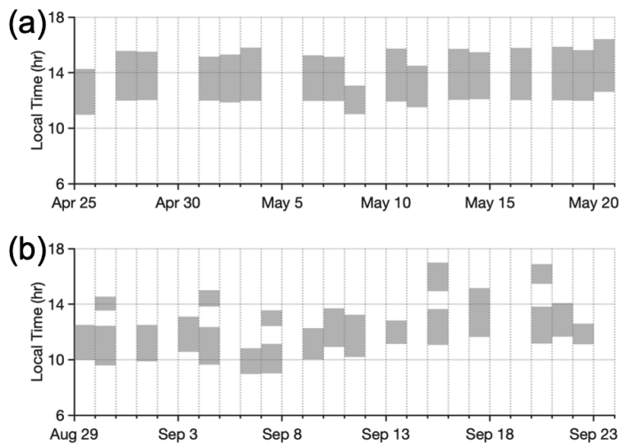
Fig. 1. Date and local time of the flights conducted during the HI-SCALE campaign: (a) spring IOP campaign (b) summer IOP campaign. During the summer IOP campaign, same-day flights were conducted to examine the temporal variation of aerosols over the SGP.
