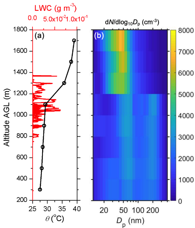
915 Fig. 12. Vertical profiles of parameters during an entrainment event over the SGP site on April 25, 2016. (a) Potential temperature ( \theta ) and liquid water content (LWC). (b) Vertical profile of aerosol size distributions as a function of altitude. The particle concentrations, surface area concentrations, and size distributions are normalized to standard temperature and pressure (273.15 K and 101.325 kPa; STP).
