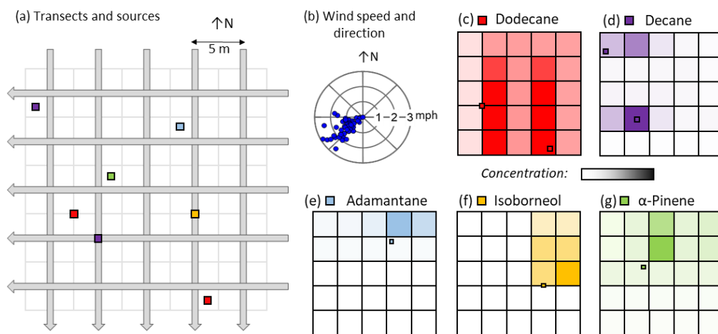
Figure 56: Overview of transect mapping. Set up shown as (a) N-S and E-W transects sampled through a 5 x 5 grid of 5m x 5m grid cells with emission sources are shown as coloured squares, and (b) wind direction and speed measured during sampling. Results are shown as colour scales representing the minimum of the two transect-average concentration observed for each cell, with colour scales normalized between zero (no fill) and the maximum observed transect-average concentration for the compound (dark fill). Compounds are (c) dodecane, red, maximum concentration of 50 pptv; (d) decane, purple, maximum concentration of 2,600 pptv; (e) adamantane, blue, maximum concentration of 7 pptv, (f) isoborneol, yellow, maximum concentration of 2 pptv, and (g) \alpha -pinene, green, maximum concentration of 400 pptv. For each result grid, the emission location of the analyte is shown.
