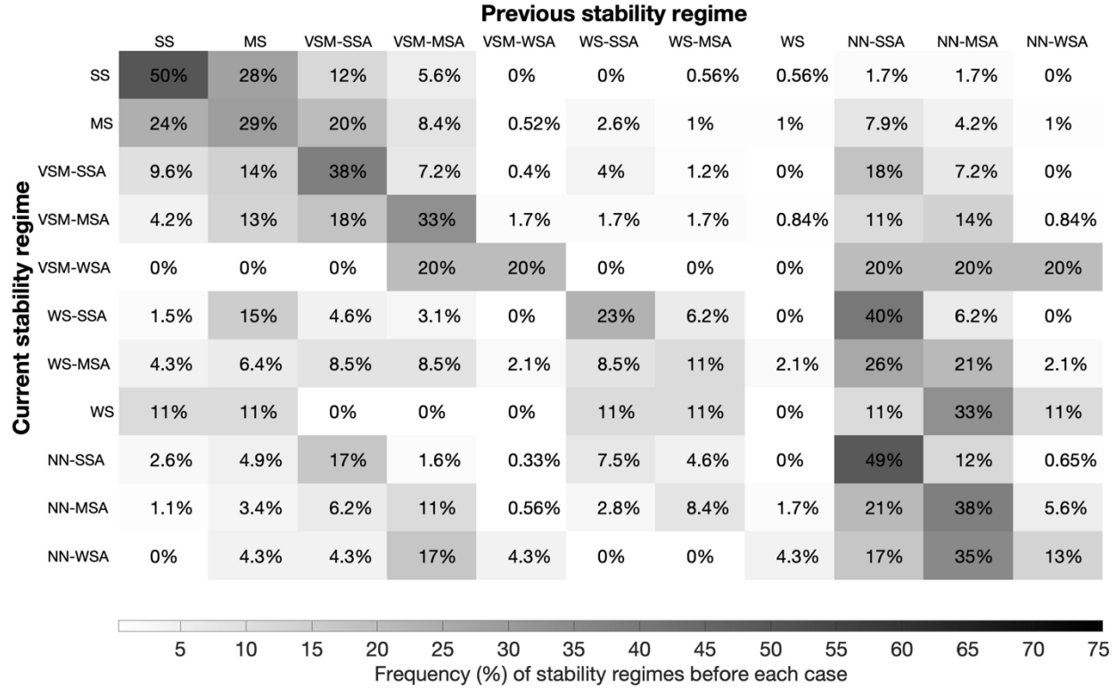
Figure 4. Grid plot showing, for each stability regime, what was the frequency of the previous case's stability regime, where the rows indicate the current stability regime, and the columns indicate the stability regime of the previous radiosonde observation. The greyscale color bar corresponds to the percent of previous cases in each stability regime, where darker grey signifies a higher percent of cases.
