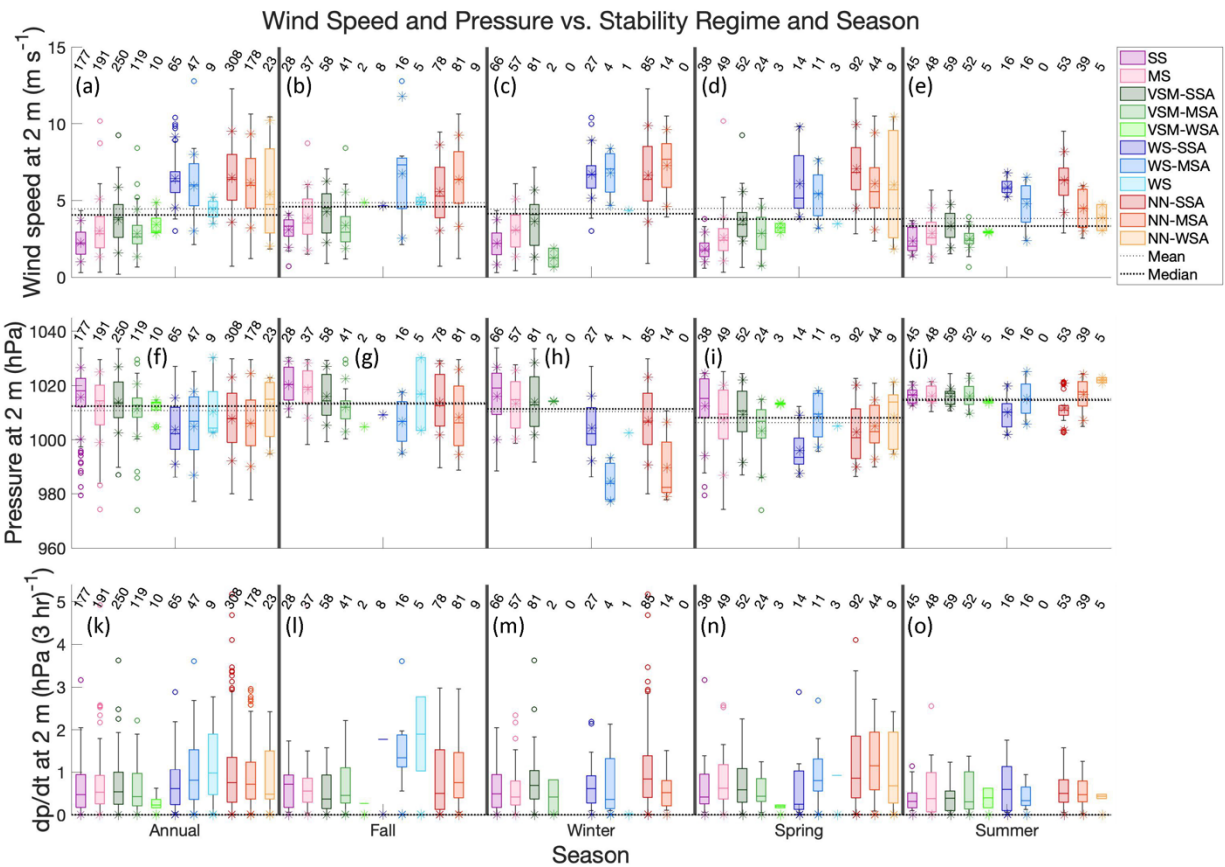
Figure 5. Top: Box and whisker plots showing the range of 2 m wind speed (a) annually, and during (b) fall, (c) winter, (d) spring, and (e) summer for each stability regime. Middle: Box and whisker plots showing the range of 2 m pressure (f) annually, and during (g) fall, (h) winter, (i) spring, and (j) summer for each stability regime. Bottom: Box and whisker plots showing the range of 2 m pressure tendency (k) annually, and during (l) fall, (m) winter, (n) spring, and (o) summer for each stability regime. The center line of each box is the median, and the outer ranges of the boxes
