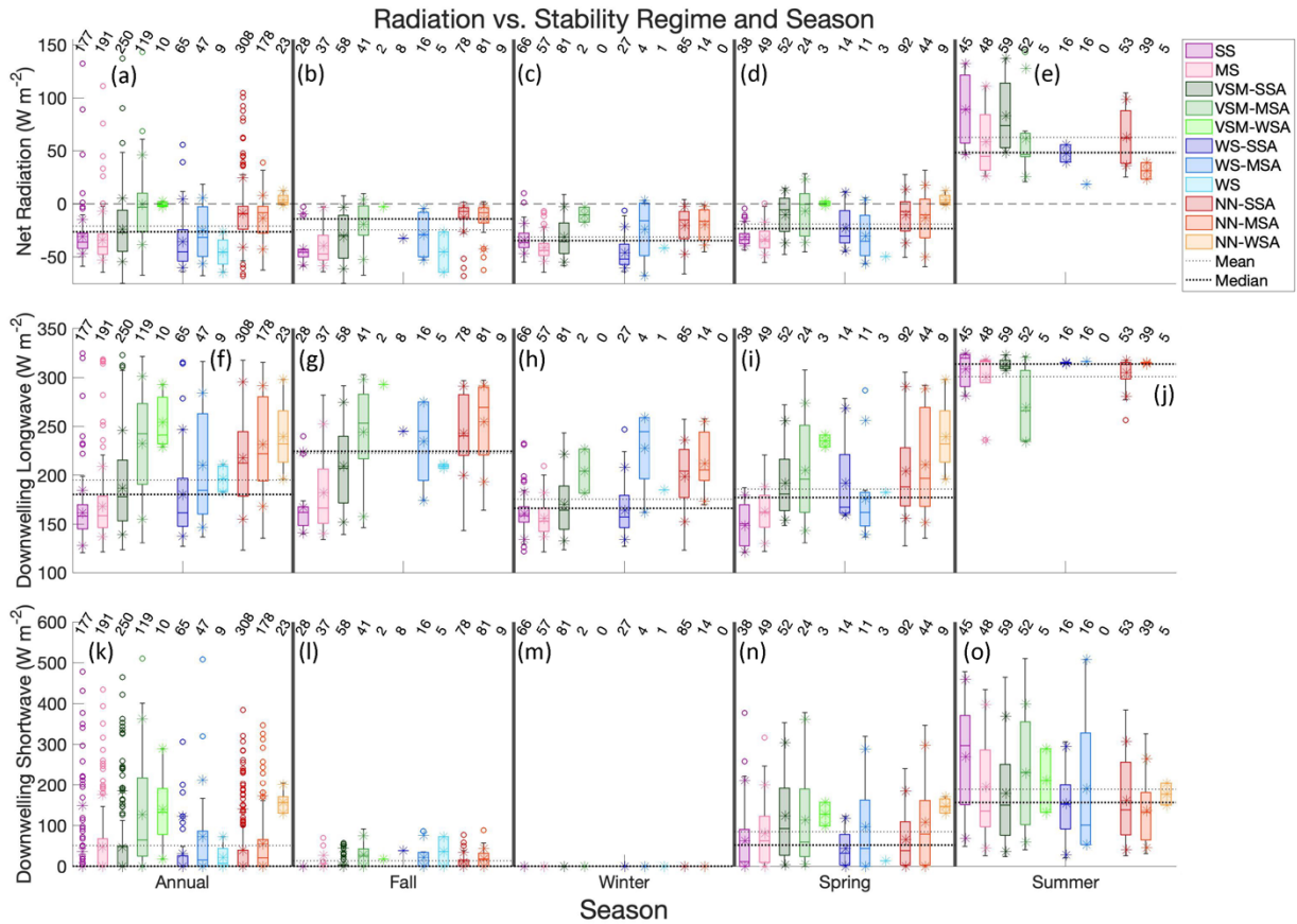
Figure 6. Top: Box and whisker plots showing the range of net radiation (a) annually, and during (b) fall, (c) winter, (d) spring, (e) summer for each stability regime. Middle: Box and whisker plots showing the range of downwelling longwave radiation (f) annually, and during (g) fall, (h) winter, (i) spring, and (j) summer for each stability regime. Bottom: Box and whisker plots showing the range of downwelling shortwave radiation (k) annually, and during (l) fall, (m) winter, (n) spring, and (o) summer for each stability regime. The center line of each box is the median, and the outer ranges of the boxes are the upper and lower quartiles. The whiskers show the range of values within 1.5 times the interquartile range from the top or bottom of the box, and outliers are shown with hollow circles. Asterisks are included at the mean, 10 th percentile, and 90 th percentile. Horizontal dotted black lines show the annual and seasonal mean (light dotted) and median (heavy dotted) values of each variable. The number of cases in each stability regime and season are written along the top of the figure.
