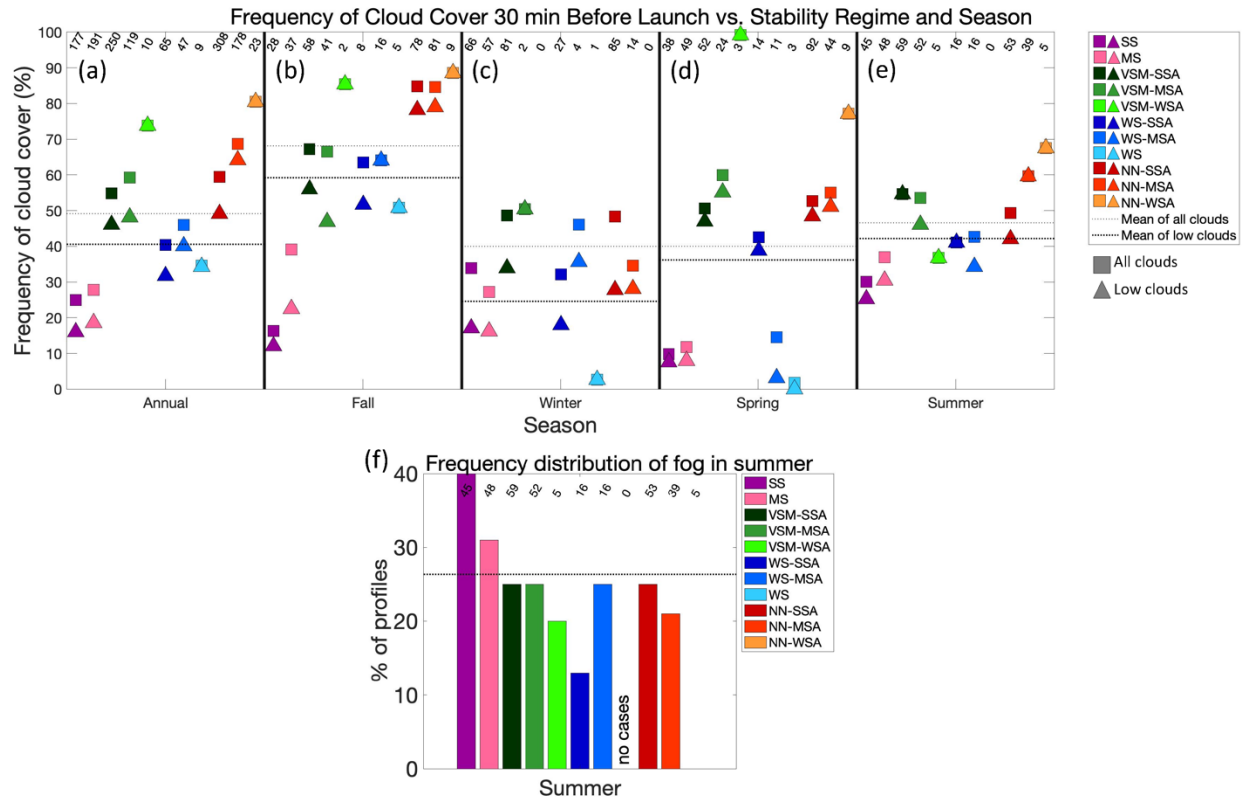
Figure 7. Top: Mean frequency of cloud cover within 30 minutes before radiosonde launch (a) annually, and during (b) fall, (c) winter, (d) spring and (e) summer for each stability regime. Square symbols show mean frequency of all clouds, and triangle symbols show mean frequency of low clouds only (cloud base height \leq 2 km). Horizontal dotted black lines show the annual and seasonal mean values of frequency of all cloud cover (light dotted) and low cloud cover (heavy dotted). The number of cases in each stability regime and season are written along the top of the figure. Bottom: (f) Percent of radiosonde profiles during summer in which fog was present, depending on stability regime. Horizontal dotted black line indicates the overall frequency of fog in summer. The number of cases in each stability regime are written along the top of the figure.
