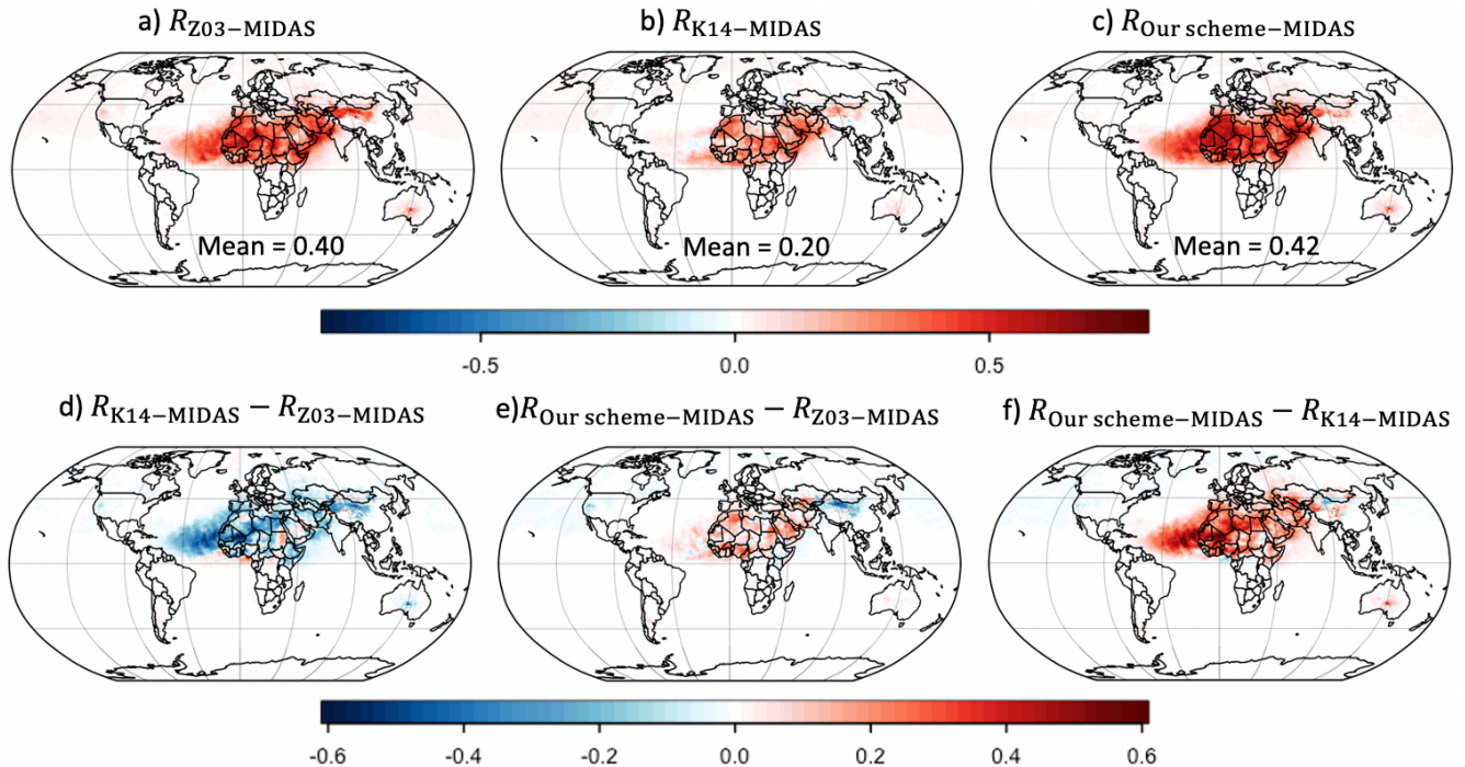
915 Figure 6. Grid-by-grid MIDAS DAOD daily Pearson correlation maps with CESM2 DAOD for 2004–2008. (a-c) Correlation maps R of MIDAS daily DAOD time series vs. CESM2 daily DAOD time series using (a) Z03, (b) K14, and (c) our scheme. The correlation maps focus on gridboxes with MIDAS DAOD/AOD ratio > 0.25 only. Pixels with MIDAS annual DAOD uncertainty (defined by Gkikas et al., 2021) larger than annual mean DAOD (see Fig. 9) are filtered out (Fig. S8 shows the unfiltered correlation maps). The values at the bottom of the panels show the global mean correlation values (for all gridboxes with MIDAS DAOD/AOD > 0.25 ). (d-f) Changes ( \Delta R ) in correlation maps from (d) Z03 to K14, (e) Z03 to our scheme, and from (f) K14 to our scheme.
