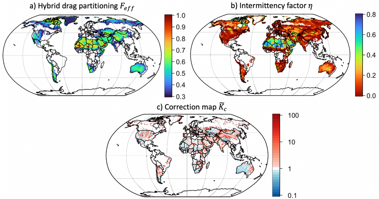
Figure 1. Implementations of proposed modifications in Leung et al. (2023) into the Community Land Model version 5 (CLM5). (a) Simulated hybrid drag partition effect F_{eff} on wind friction velocity considering the land surface roughness due to rocks and green vegetation. (b) The fraction of time that dust emission is active (intermittency factor \eta ), averaging across all time steps when the emission flux F_d > 0 . Note that the colorbar in (b) is inverted compared to (a) to show the contrasts in \eta between hyperarid and nonarid regions more clearly. (c) Correction map \tilde{K}_c for 0.9^\circ \times 1.25^\circ dust emission from the standalone dust emission model obtained in Leung et al. (2023).
