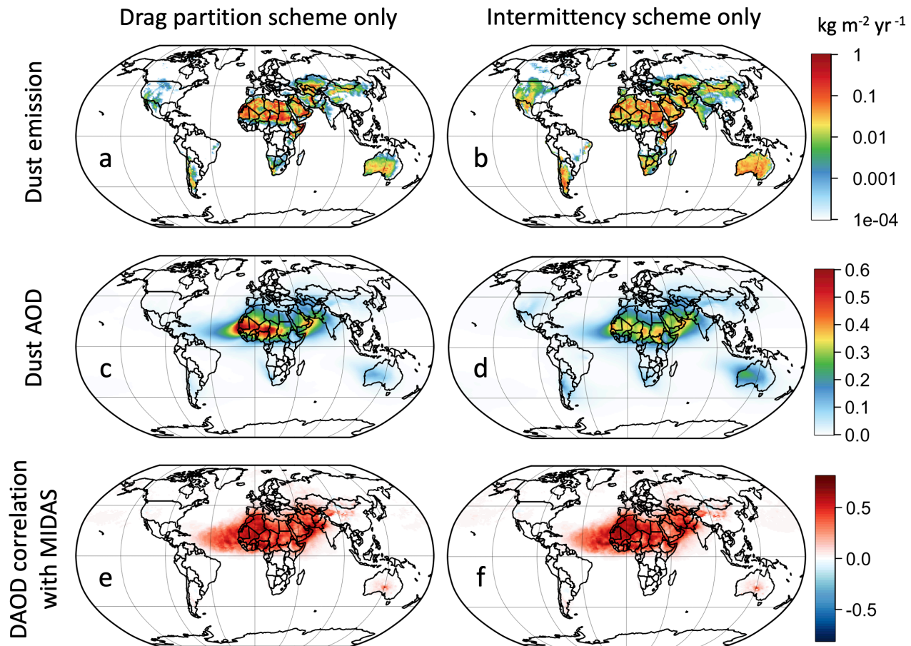
1065 Figure 10. Separating the contributions of the hybrid drag partition scheme (left) and the Comola et al. (2019) intermittency scheme (right) to our dust emission scheme (Leung et al., 2023). The rows represent simulated (a, b) dust emission, (c, d) dust aerosol optical depth (DAOD) with global means of 0.03, and (e, f) daily DAOD correlation with MIDAS DAOD from Gkikas et al. (2021).
