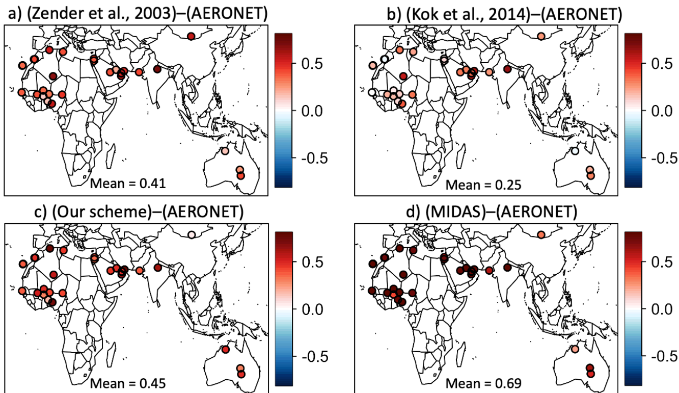
945 Figure 7. AERONET–SDA coarse mode AOD daily correlations for 2004–2008 over selected sites with CESM DAOD using (a) Z03, (b) K14, and (c) our study. (d) MIDAS DAOD versus AERONET–SDA AOD daily correlation. The values at the bottom of the panels represent the mean correlation across all AERONET stations.
