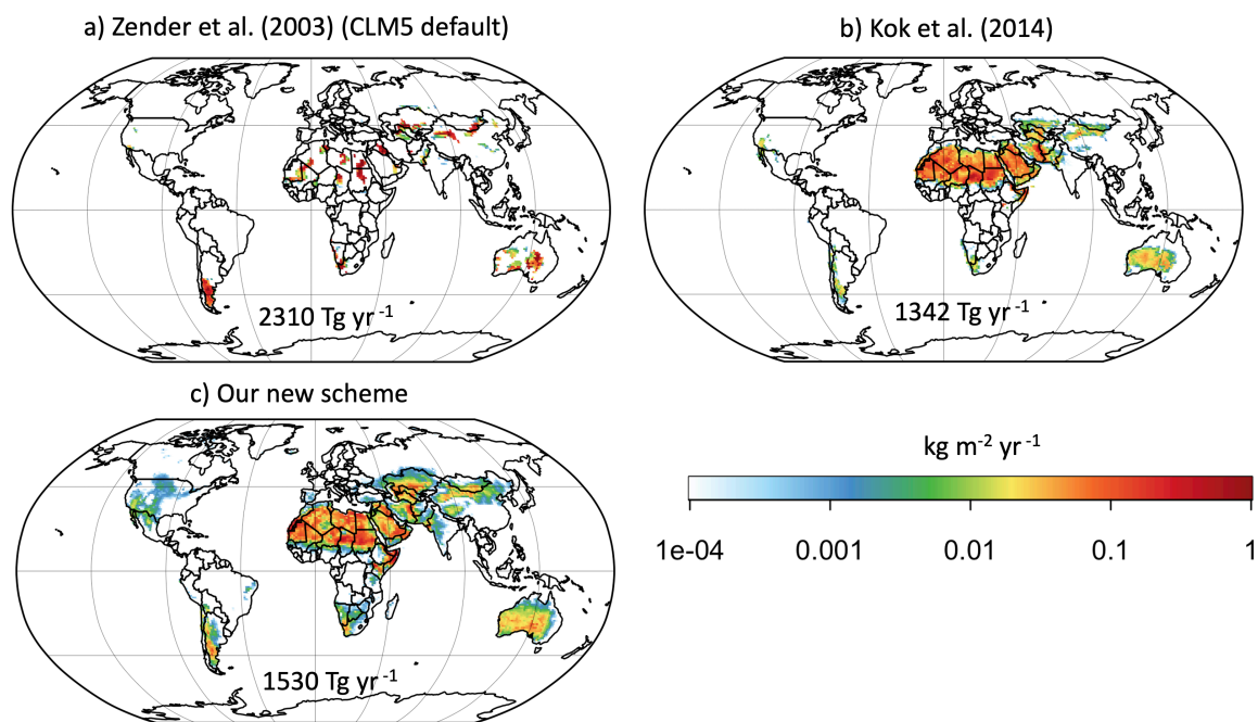
705 Figure 2. CESM/CLM5 dust emissions averaged across 2004–2008, for (a) Z03, (b) K14, and (c) our new scheme (Leung et al., 2023). All emissions are normalized such that the corresponding CAM6 dust aerosol optical depth (DAOD) is 0.03 \pm 0.01 (following the global DAOD constraint obtained by Ridley et al., 2016). The global total emissions (in Tg yr -1 ) to yield a global mean DAOD of 0.03 are indicated in each 710 panel.
