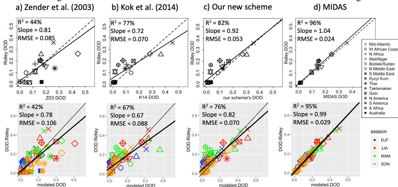
800 Figure 4. Ridley et al. (2016) regional mean DAOD vs. modeled CESM2 DAOD using (a) Z03, (b) K14, and (c) our scheme, as well as (d) MIDAS DAOD (Gkikas et al., 2021), for 2004–2008 over 15 dusty regions (see Fig. S5) defined following Kok et al. (2021). Top panels show annual mean DAOD scatterplots, with dashed lines as 1:1 lines and solid lines as the reduced major axis (RMA) regression lines. Bottom panels show seasonal mean DAOD scatterplots for the three schemes, with thin lines as 1:1 805 lines and thick lines as the RMA regression lines. Seasons are defined as: DJF (December–January– February), MAM (March–April–May), JJA (June–July–August), and SON (September–October– November).
