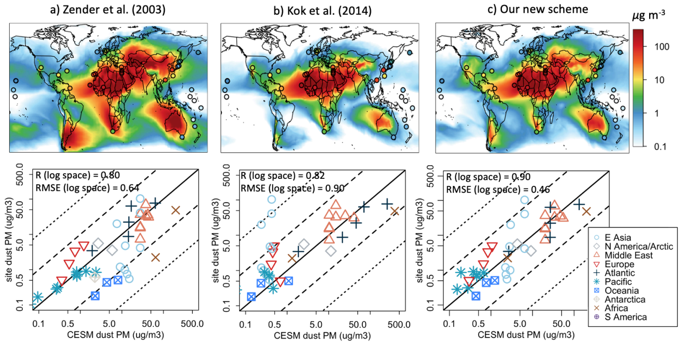
995 Figure 8. CESM2 dust PM_{10} concentration (in \mu g m^{-3} ) vs. climatological in-situ PM_{10} measurements (Sect. 4.4) for (a) Z03, (b) K14, and (c) our study. In the bottom panels, sites are labeled over different continents / oceans with different symbols and colors.
