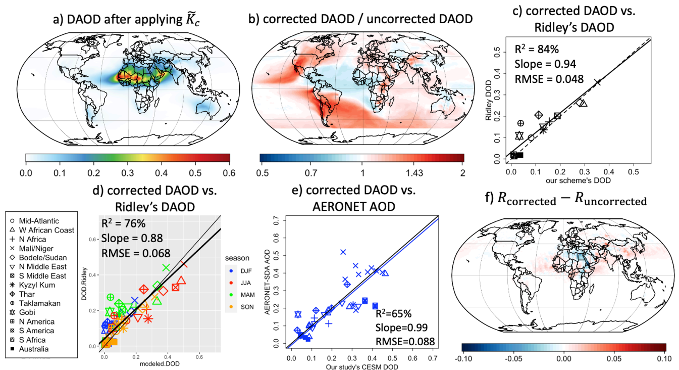
1120 Figure 11. Effects of using the scaling map \tilde{K}_c to correct the 0.9^\circ \times 1.25^\circ CLM5 dust emissions on the CAM6 dust cycle. (a) DAOD spatial pattern simulated by our scheme after the global dust emission pattern is corrected by \tilde{K}_c . (b) Corrected DAOD (Fig. 11a) divided by the uncorrected DAOD (Fig. 3c). Both DAOD maps are rescaled to have the same global mean to emphasize their difference in spatial variability. (c, d) Corrected DAOD versus Ridley regional DAOD (c) annually and (d) seasonally. (e) Corrected DAOD versus AERONET-SDA coarse mode AOD. (f) Changes in correlation maps ( \Delta R ) between 1125 corrected DAOD vs. MIDAS DAOD and uncorrected DAOD vs. MIDAS DAOD.
