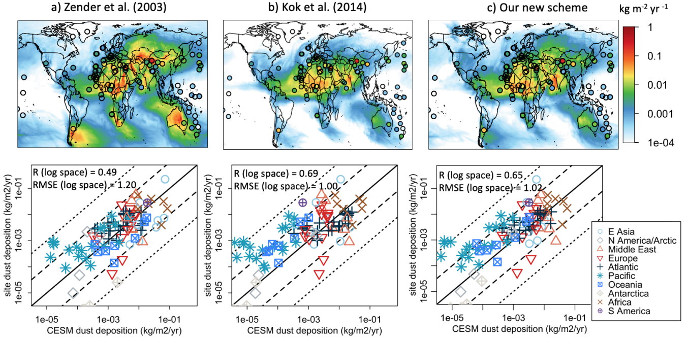
Figure 9. CESM2 dust total (dry + wet) deposition (in \text{kg m}^{-2} \text{yr}^{-1} ) vs. climatological in-situ deposition measurements for (a) Z03, (b) K14, and (c) our study. In the bottom panels, sites are labeled over different continents / oceans with different symbols and colors.
