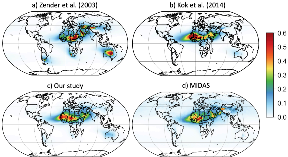
760 Figure 3. Global DAOD averaged across 2004–2008 from CESM2 and MIDAS. (a-c) CESM DAOD for (a) Z03, (b) K14, and (c) our new scheme (Leung et al., 2023). (d) MIDAS DAOD (Gkikas et al., 2021). All maps have a global mean of 0.03 \pm 0.01 consistent with the global DAOD constraint obtained by Ridley et al., 2016).
