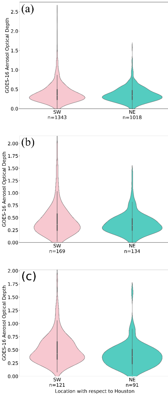
Figure 12: Violin plots depicting the distributions of the average of the 30-minute AOD values for the period prior to cell initiation to the southwest (red) and northeast (blue) of Houston for (a) shallow, (b) modest deep, and (c) vigorous deep convective cells. The number n under each violin plot corresponds to the number of cells considered for each distribution.
