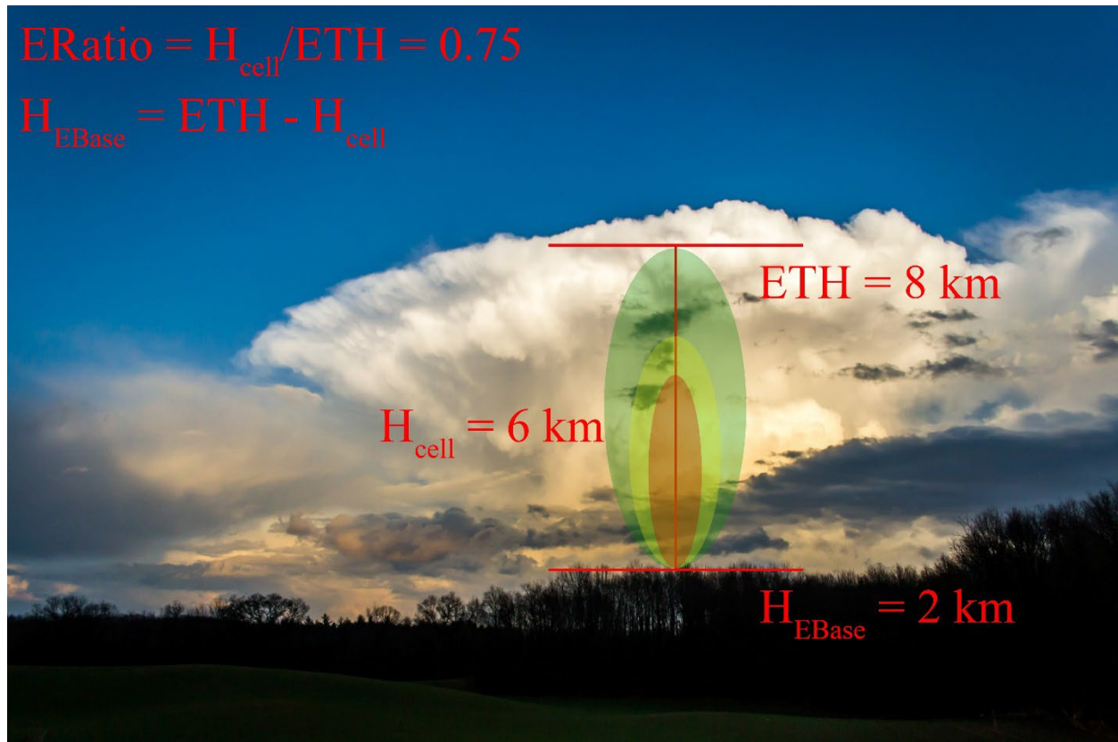
665 Figure 1: A visual illustration of ERatio , H_{cell} , and H_{EBase} . This image is meant to provide a visual context for these three variables. The red, yellow, and green shaded areas represent arbitrary high, medium, and low reflectivity contours respectively. ERatio and H_{EBase} are calculated using the maximum ETH and H_{cell} , which are radar-derived quantities and will always be less than the actual height of the storm top and physical depth of a given cell.
