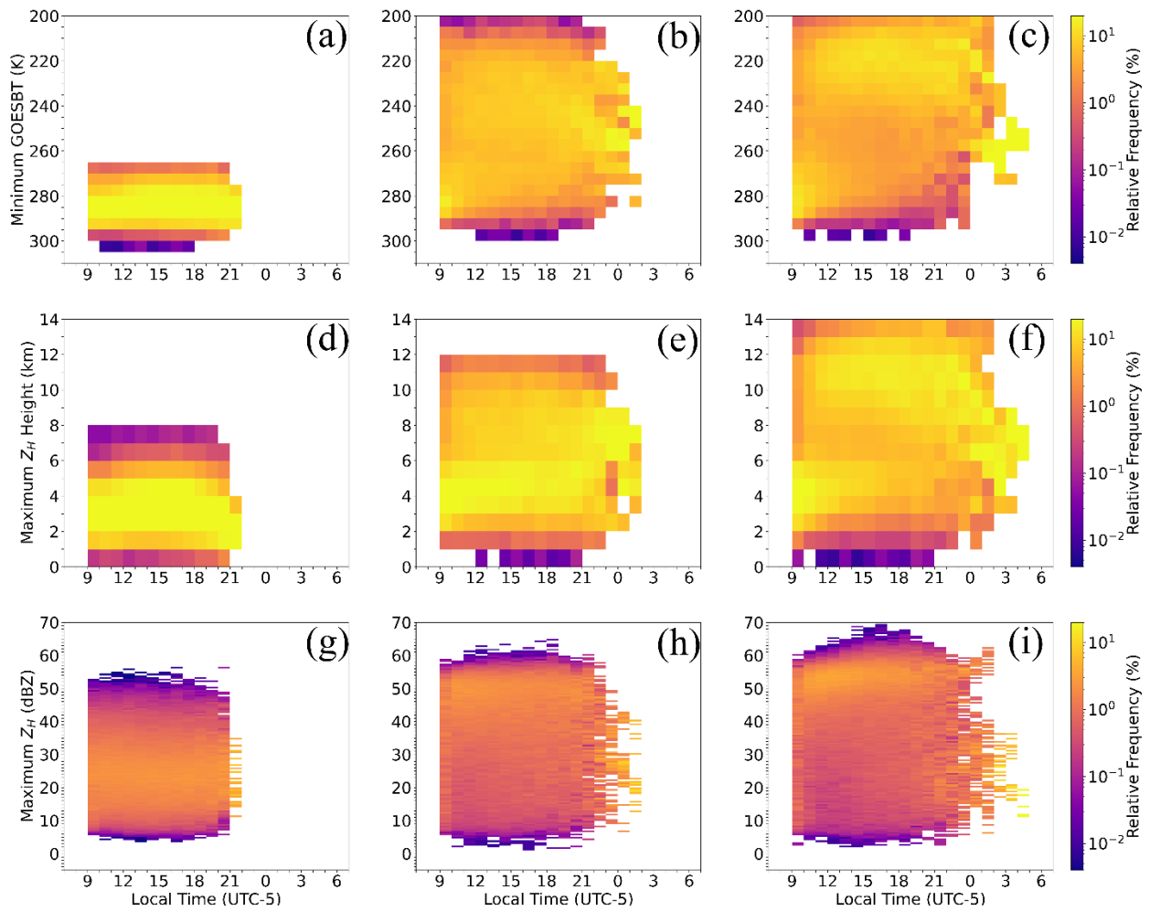
685 Figure 6: The time bin normalized distributions of GOESBT (a, b, c), H_{dBZ_{max}} (d, e, f), and dBZ_{max} (g, h, i) over the course of a day for all scans over the lifetimes of shallow (a, d, g), modest deep (b, e, h), and vigorous deep (c, f, i) convection.
