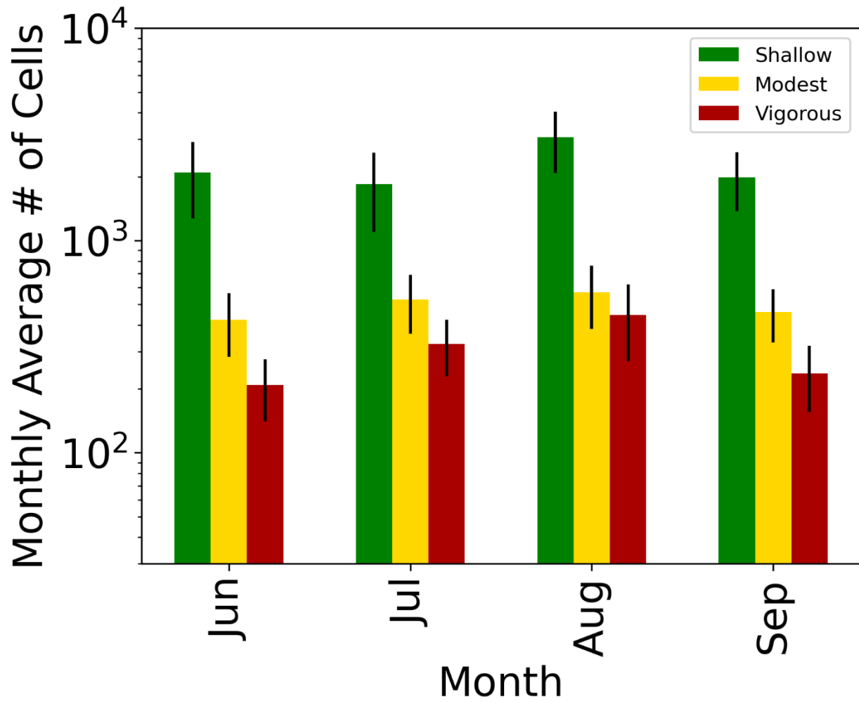
670 Figure 2: Bar graphs showing the monthly average cell count for shallow (green), modest deep (yellow), and vigorous deep (red) convection. The vertical black lines at the top of each bar denote \pm one standard deviation.
