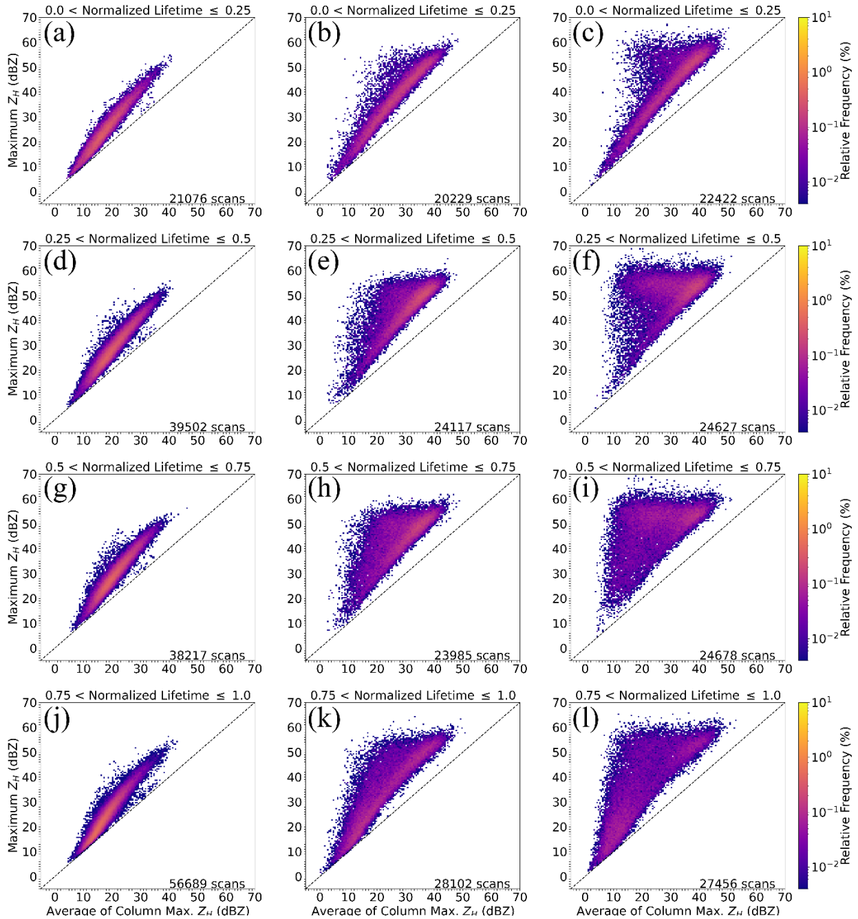
695 Figure 9: As in Fig. 7, but for \text{dBZ}_{\text{avg}} versus \text{dBZ}_{\text{max}} . The dashed line shows the one-to-one value of \text{dBZ}_{\text{avg}} and \text{dBZ}_{\text{max}} .
