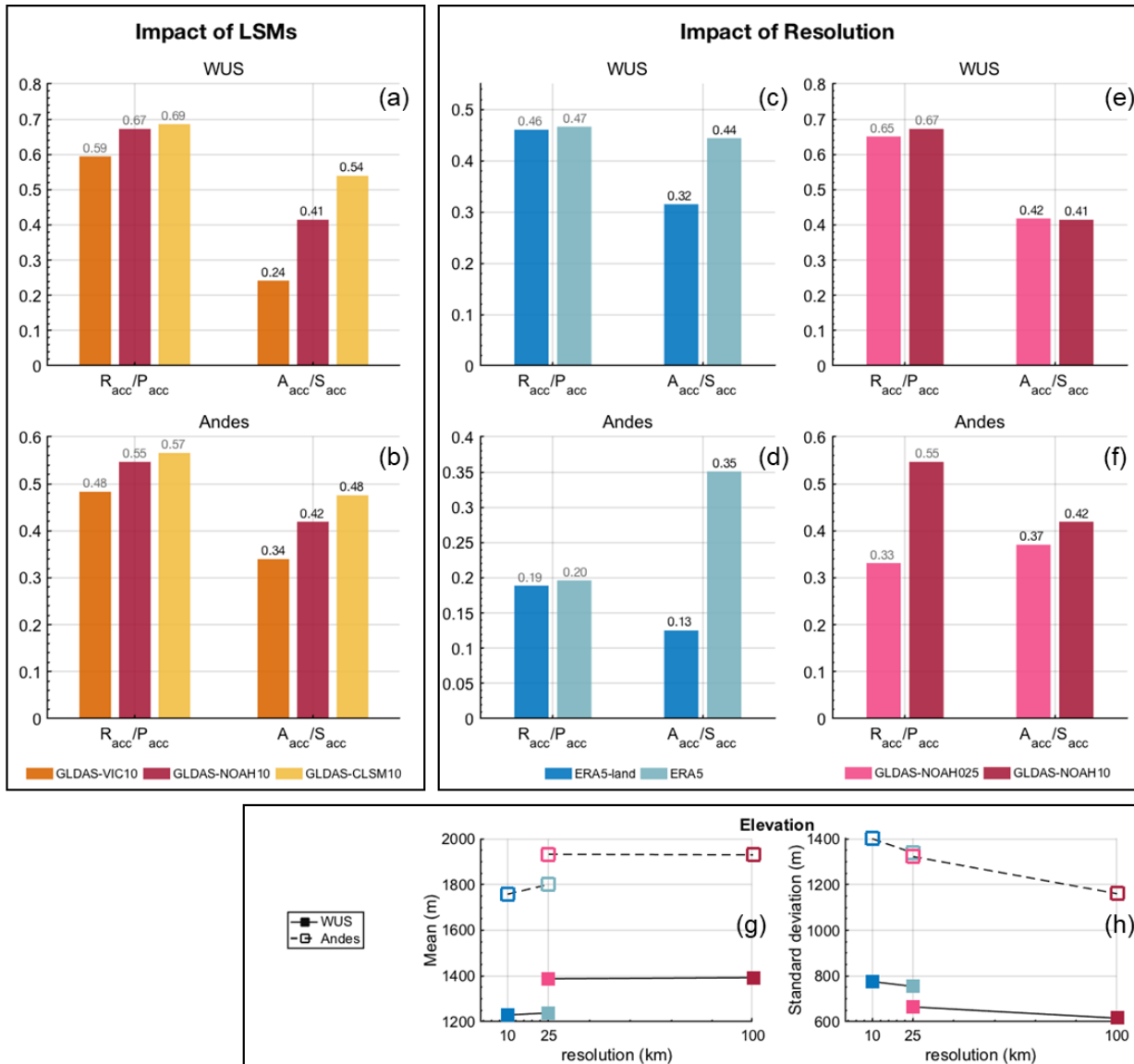
Figure 11. (a) and (b) R_{acc}/P_{acc} and A_{acc}/S_{acc} for three GLDAS LSMs (VIC, Noah, and Catchment) at the same spatial resolution (~ 100 km). (c) and (d) R_{acc}/P_{acc} and A_{acc}/S_{acc} for ERA5-Land (~ 10 km) and ERA5 (~ 25 km) using the same LSM and similar forcings, but different spatial resolutions. (e) and (f) R_{acc}/P_{acc} and A_{acc}/S_{acc} for GLDAS-NOAH025 (~ 25 km) and GLDAS-NOAH10 (~ 100 km) using the same LSM and similar forcings, but different spatial resolutions. (g) and (h) mean and standard deviation of elevation over WUS and Andes from the ERA5-Land and ERA5 group, and the GLDAS-NOAH025 and GLDAS-NOAH10 group (where colors represent the products shown in (c)-(f)).
