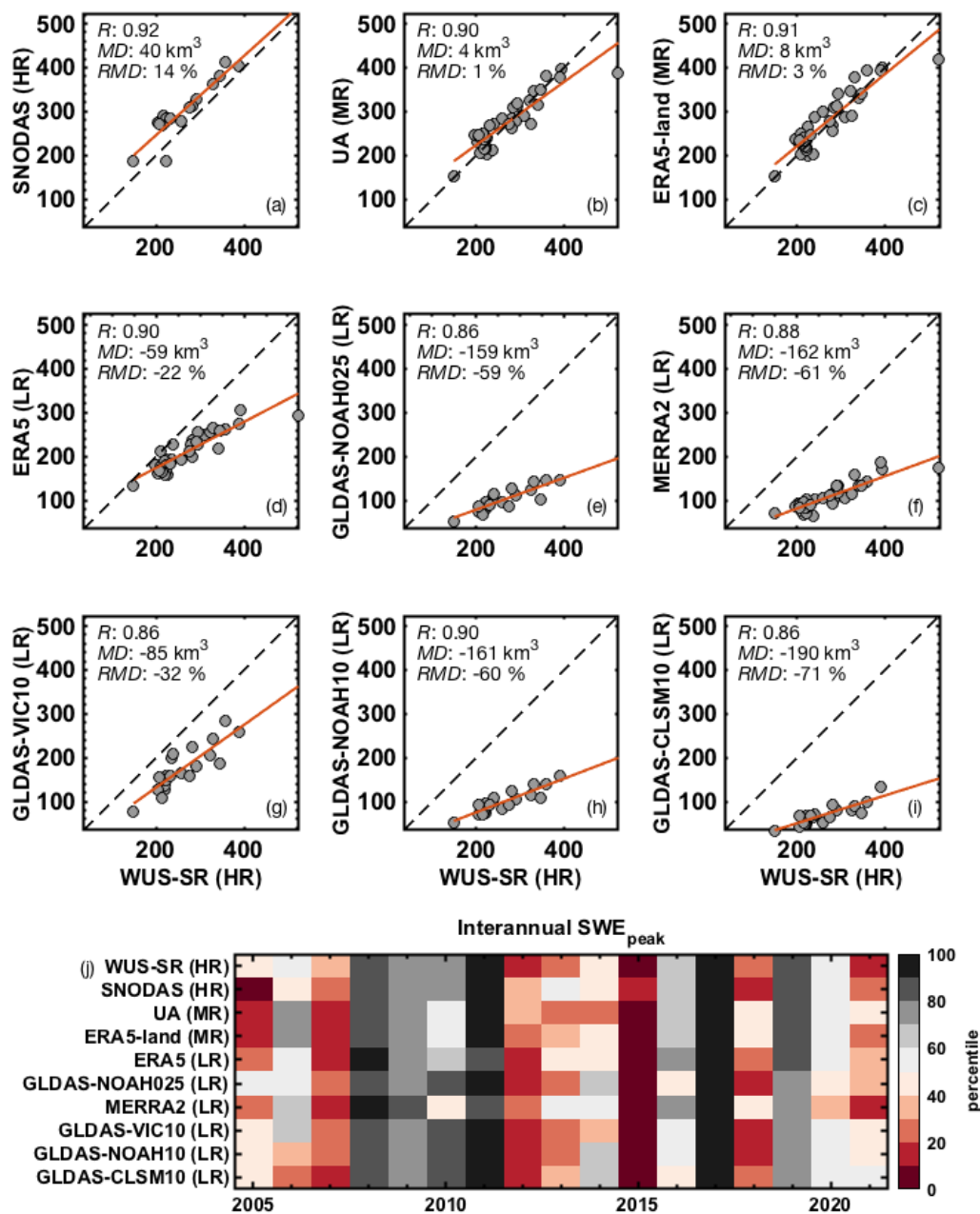
295 Figure 7. Scatter plots (a – i) of SWE_{\text{peak}} volumes between WUS-SR and other products. Each dot represents SWE_{\text{peak}} volume ( \text{km}^3 ) for each year over the study period (WYs 1985 to 2021) where data is available. For the SNODAS and GLDAS products, the comparison is over WYs 2005 to 2021, and 2001 to 2021, respectively. (j) shows the SWE_{\text{peak}} percentiles in each WY over the overlapping period including all products (WYs 2005 to 2021).
