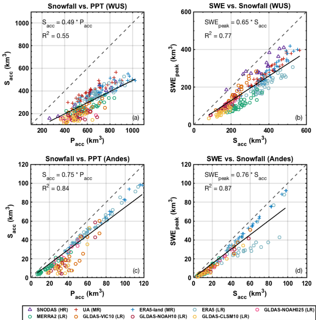
Figure 9. Left panels show scatter plots of accumulation-season S_{acc} ( km^3 ) vs. P_{acc} ( km^3 ) volumes over the WUS and Andes, respectively, indicating the partitioning of precipitation into snowfall. Right panels show scatter plots of accumulation-season SWE_{peak} ( km^3 ) vs. S_{acc} ( km^3 ) over WUS and Andes, respectively, indicating how much snowfall remains as SWE vs. being lost to ablation. Solid lines are linear regression and dashed lines are 1:1 lines.
