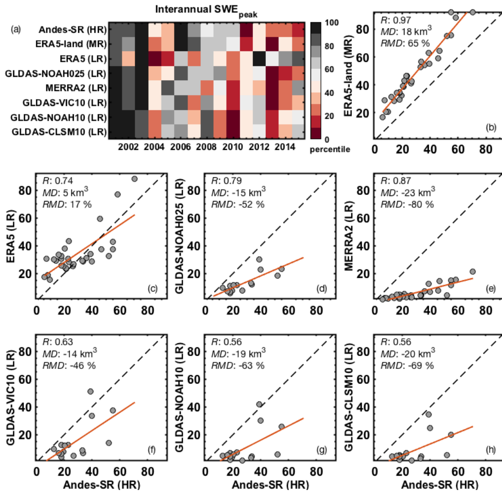
300 Figure 8. Scatter plots (b – h) of SWE_{peak} volumes between Andes-SR and other products. Each dot represents SWE_{peak} volume ( km^3 ) for each year over the study period (WYs 1985 to 2015) where data is available. For the GLDAS products, the comparison is over WYs 2001 to 2015. (a) shows the SWE_{peak} percentiles in each WY over the overlapping period including all products (WYs 2001 to 2015).
