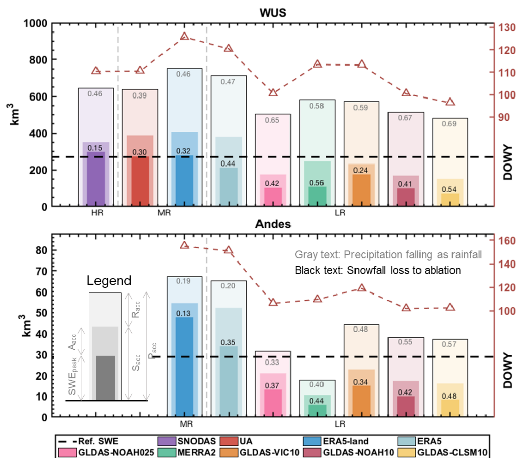
Figure 10. Climatological SWE_{peak} , S_{acc} , and P_{acc} volumes aggregated over WUS (top panel) and Andes (bottom panel) in km^3 . Red triangles (corresponding to right y-axis) shows the t_{peak} averaged over all pixels and WYs. The horizontal dashed lines are the reference snow reanalysis SWE volumes from WUS-SR and Andes-SR. The vertical dashed lines group the products by spatial resolution (i.e., HR, MR, LR). The black text lists the A_{acc}/S_{acc} and gray text lists the R_{acc}/P_{acc} .
