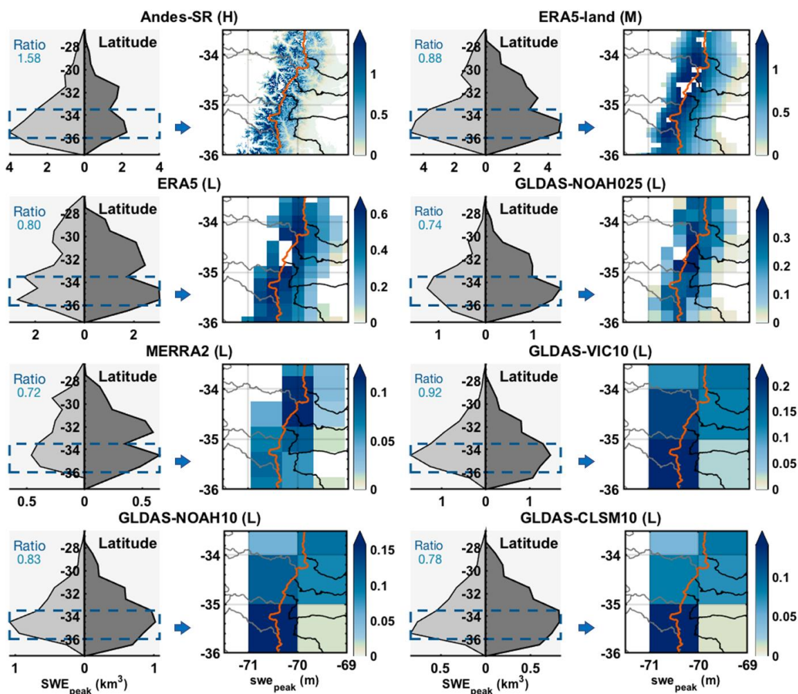
265 Figure 6. Latitudinal distribution of SWE_{peak} ( km^3 ) over windward ( SWE_{peak}^{wind} ; light gray areas) and leeward basins ( SWE_{peak}^{leeward} ; dark gray areas) in the Andes in first and third columns. Text labels indicate the ratios of latitudinally-integrated SWE_{peak}^{wind} to SWE_{peak}^{leeward} . The climatological swe_{peak} (m) spatial patterns corresponding to the latitude bands indicated by dashed boxes are illustrated in the second and fourth columns. The red line represents the Andes ridgeline separating windward (western) from leeward (eastern) basins. Note: Different swe_{peak} ranges are used for each product to highlight latitudinal/spatial patterns.
