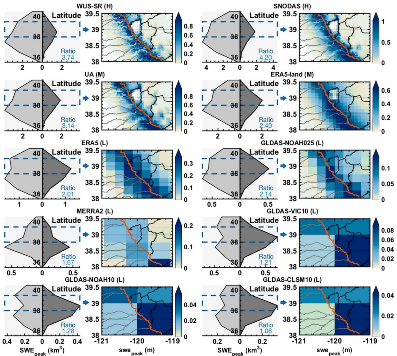
Figure 5. Latitudinal distribution of integrated SWE_{peak} ( km^3 ) over windward ( SWE_{peak}^{wind} ; light gray areas) and leeward basins ( SWE_{peak}^{lee} ; dark gray areas) in the Sierra Nevada in first and third columns. Text labels indicate the ratio of latitudinally- 260 integrated SWE_{peak}^{wind} to SWE_{peak}^{lee} . The climatological swe_{peak} (m) spatial patterns corresponding to the latitude bands indicated by dashed boxes are illustrated in the second and fourth columns. The red line represents the Sierra Nevada ridgeline separating
