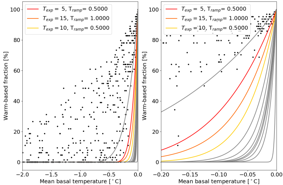
Figure 10. Warm-based fraction (basal temperature with respect to the pressure melting point at 0 °C) vs. mean basal temperature with respect to the pressure melting point when upscaling a 3.125 km run to 25 km horizontal grid resolution including all 5 parameter vectors using the GSM. For example, an upscaled 25 km patch (containing 64 3.125 km grid cells) with 32 3.125 km grid cells at the pressure melting point and 32 3.125 km grid cells at -1^{\circ}\text{C} with respect to the pressure melting point has a warm-based fraction of 50 % and a mean basal temperature of -0.5^{\circ}\text{C} . Only grid cells within the pseudo-Hudson Strait and time steps within the surges of the 10 kyr after the first surge are considered. The restriction to the 10 kyr after the first surge for these experiments is set by storage limitations due to the high temporal resolution of the model output fields (10 yr). The colored ramps correspond to the 25 km horizontal grid resolution basal temperature ramps in Table S11 and the gray lines show all other ramps that were tested at this resolution.
