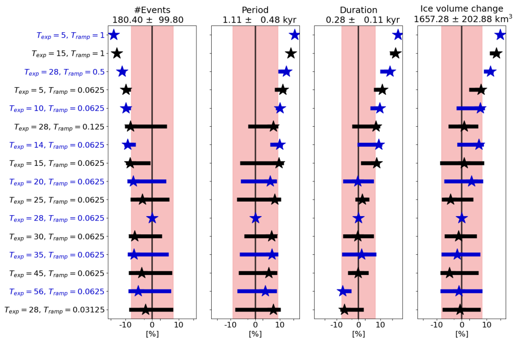
Figure 9. Percentage differences in surge characteristics compared to the GSM reference setup ( T_{ramp} = 0.0625, T_{exp} = 28 ) for different basal temperature ramps at 3.125 km horizontal grid resolution (average of the 5 parameter vectors). The ramps are sorted from widest (first row) to sharpest (last row, see Fig. S25 for a visualization of all ramps). Otherwise same as Fig. 6. No runs crashed and all runs had more than 1 surge event. The exact values are given in Table S10.
