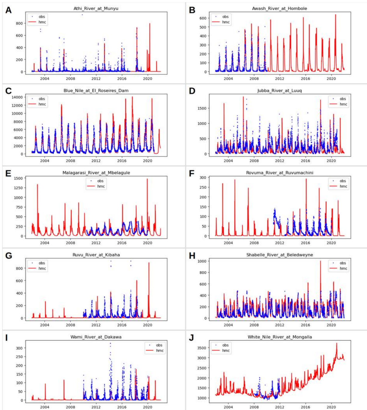
390 Figure 3: Comparison of simulated versus available observed discharges at 10 stations sampled from all 8 validation domains for the period 2002-2021.
