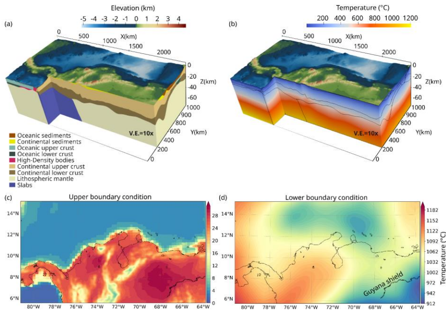
180 Figure 2. 3D thermal model with its structural layers and boundary conditions. The thermal calculation was based on a 3D data-integrative model of the study area, which includes the thermal signature of the heterogeneities from the lithospheric mantle (75 km depth) to the surface. (a) 3D structural model (Gómez-García et al., 2020, 2021) used to compute the 3D thermal field. The model includes fifteen different layers, although the figure only depicts those visible in the 3D view. Lithology- constrained thermal parameters were assigned to each of them (Table 1). (b) 3D steady-state thermal field, with the boundaries 185 between layers of the structural model depicted as black thin lines. Both the structural and thermal models are shown with a 10X vertical exaggeration. (c) Upper boundary condition, which integrates the temperatures over the continent from the ERA5- Land dataset (Copernicus Climate Change Service, 2019) with those on the seabed from the GLORYS dataset (Ferry et al., 2010). (d) Lower boundary condition, set as the temperatures at 75 km depth, after converting S-wave velocities into temperatures (details in Sect. 3.1.2).
