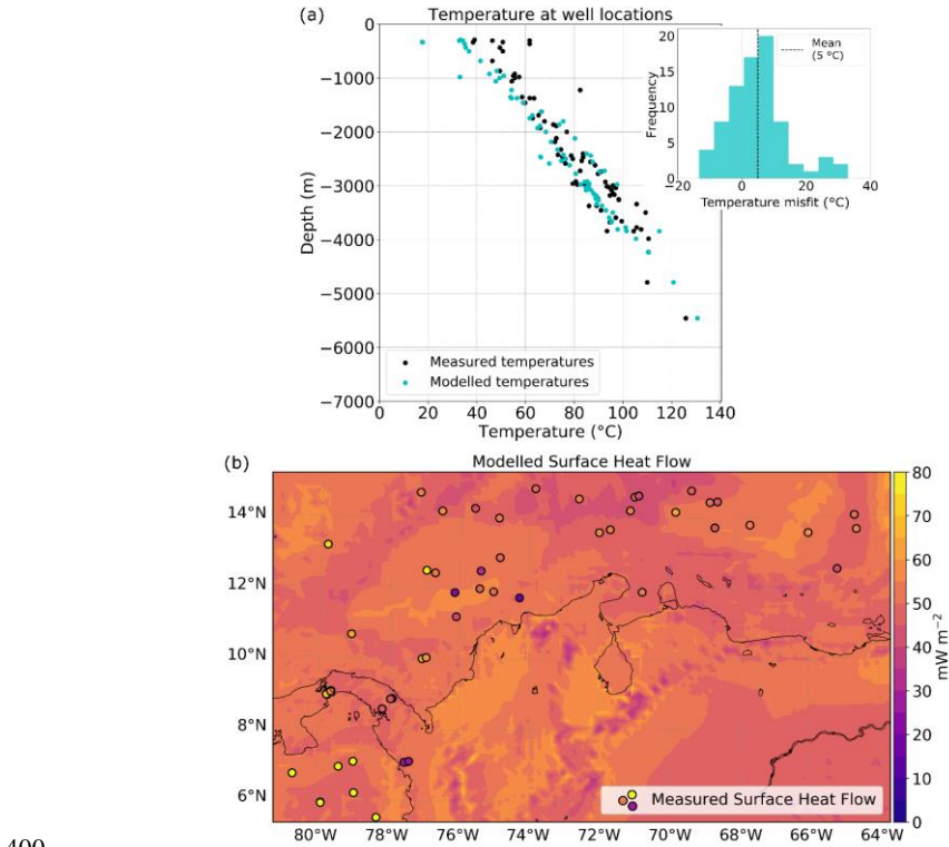
400 Figure 4. Validation of the 3D thermal field against measurements of downhole temperatures and surface heat flow. (a) Modelled borehole temperatures show a good agreement with the observed temperatures. The largest misfits
