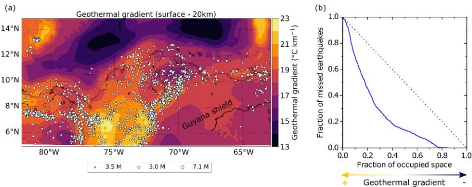
475 Figure 5. Correlation between geothermal gradient and the spatial distribution of crustal seismicity. (a) Geothermal gradient in the study area computed in the uppermost 20 km of the lithosphere (about the regional average of the crustal seismogenic depth, Sect. 4.3). Large spatial variations are observed both onshore and offshore. White dots: Crustal seismicity analyzed in this study (Sect. 3.2.1). (b) Molchan diagram showing the skill of the spatial distribution of the geothermal gradient at forecasting the distribution of crustal earthquakes.
