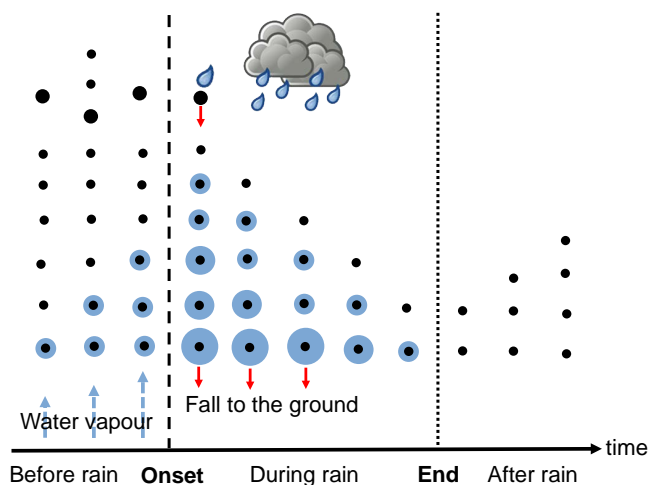
Figure 5. Schematic diagram of the temporal evolution of aerosols before, during, and after rain. The dashed line indicates the onset of rainfall, while the dotted line marks its end. The black dots represents aerosol particles, and the blue area represents the water film. The dashed blue arrow represents water vapor, and the red arrow represents particles falling to the ground.
