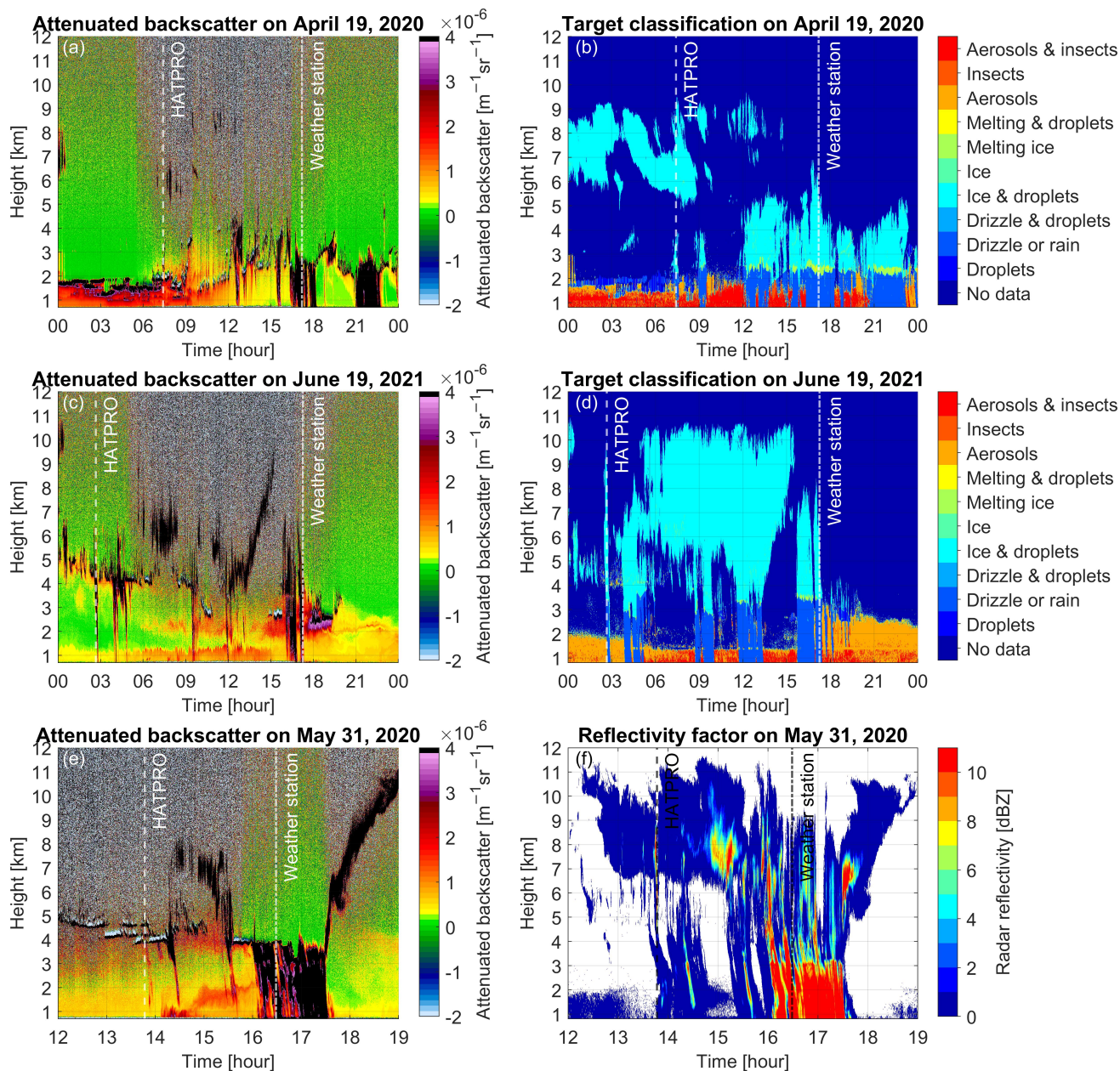
Figure 7. Ceilometer attenuated backscatter and cloud radar target classification for (a and b) April 19, 2020 and (c and d) June 19, 2021. (e) Ceilometer attenuated backscatter and (f) cloud radar reflectivity factor on May 31, 2020. Dashed and dash-dotted lines are the onset of rain identified by HATPRO and the weather station respectively.
