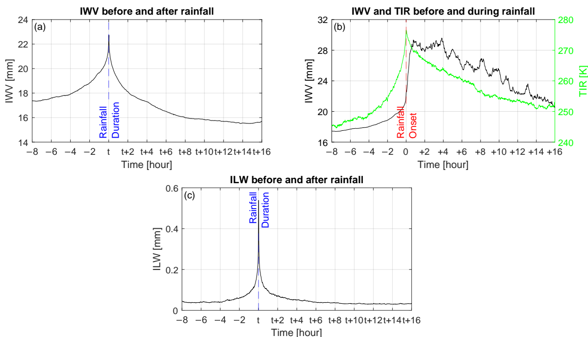
Figure 3. Composites of (a) IWV 8 h before and 16 h after rain, (b) IWV and TIR (green line) 8 h before and 16 h during rain, and (c) ILW 8 h before and 16 h after rain provide by HATPRO in Granada.
