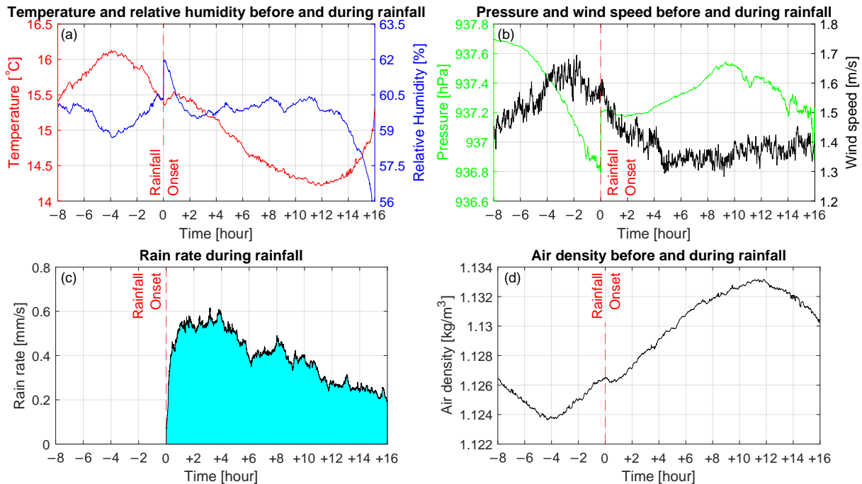
Figure 6. Composites of (a) temperature (red line) measured by weather station, relative humidity (blue line) measured by weather station, (b) pressure (green line) measured by HATPRO weather sensor, wind speed (black line) measured by weather station, and (c) rain rate (black line) retrieved from HATPRO 8 h before and 16 h during rain in Granada. 0 is the onset of rain. -1 and +1 represent 1 h before and during rain respectively.
