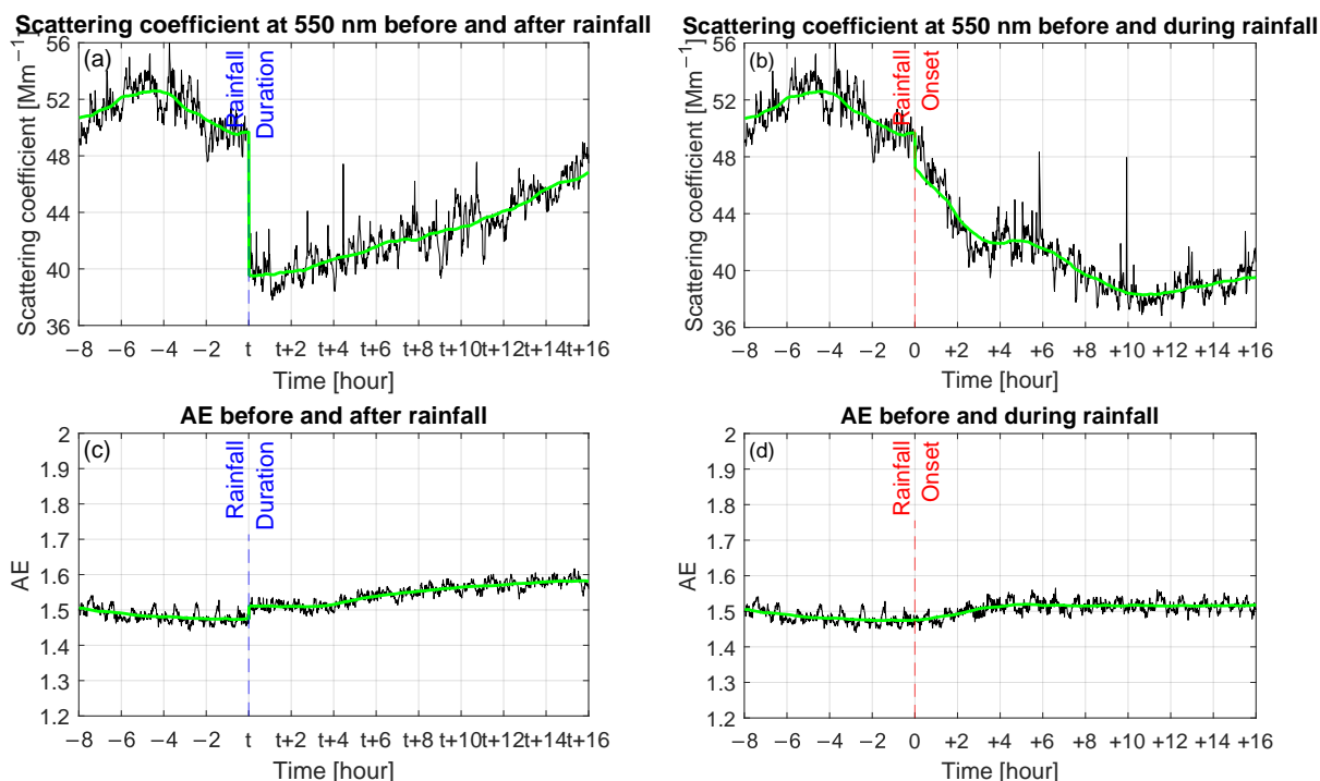
Figure 4. Composites of (a) scattering coefficient 8 h before and 16 h after rain, (b) scattering coefficient 8 h before and 16 h during rain, (c) AE 8 h before and 16 h after rain, and (d) AE 8 h before and 16 h during rain provide by integrating nephelometer in Granada. t is the duration of rain. 0 is the onset of rain. -1, +1, and t+1 represent 1 h before, during, and after rain respectively. The green line is the mean value calculated over a sliding window of 3 h.
